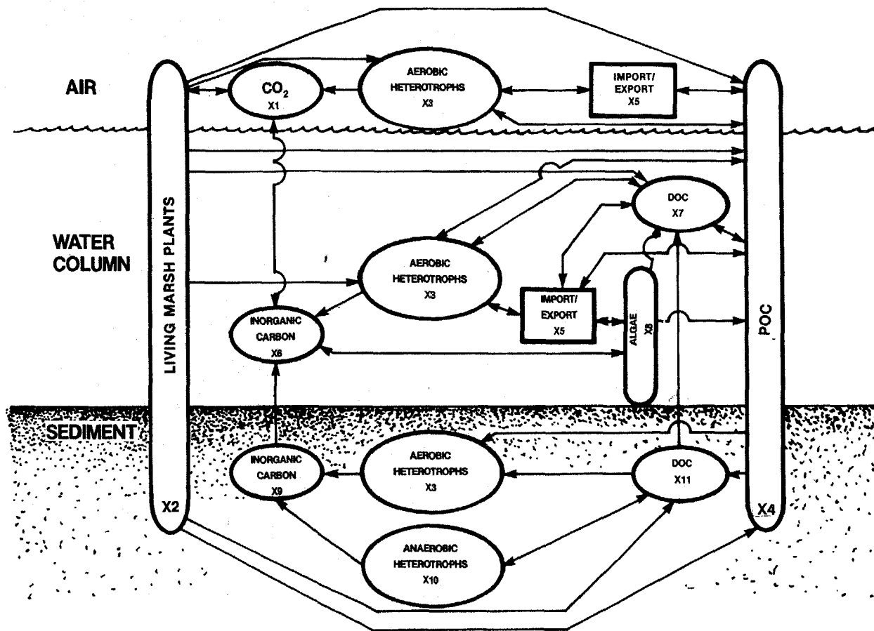
Figure 17. Conceptual model of carbon flow between components of tidal marsh ecosystems in the Pacific Northwest.
