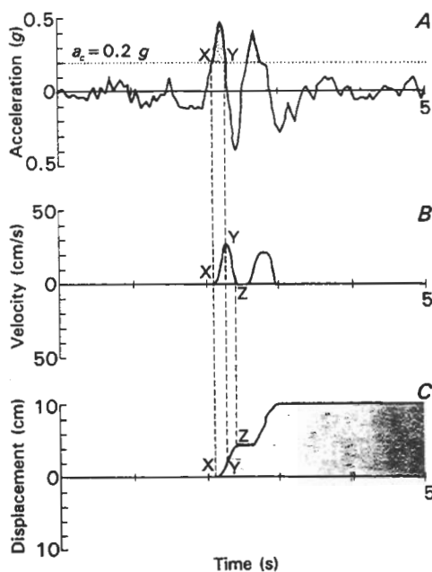
FIGURE 3 Demonstration of the Newmark-analysis algorithm, adapted from Wilson and Keefer (2). Points X, Y, and Z are discussed in text; A, earthquake acceleration-time history with critical acceleration (dotted line) of 0.20 g superimposed; B, velocity of landslide block versus time; C, displacement of landslide block versus time.
