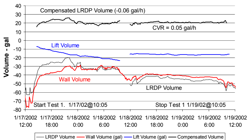
Figure 7. Results of the First Test Conducted by KWA without Introducing an Induced Leak.
