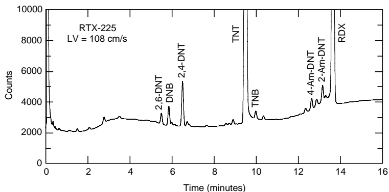
c. RTX-225 confirmation column.
