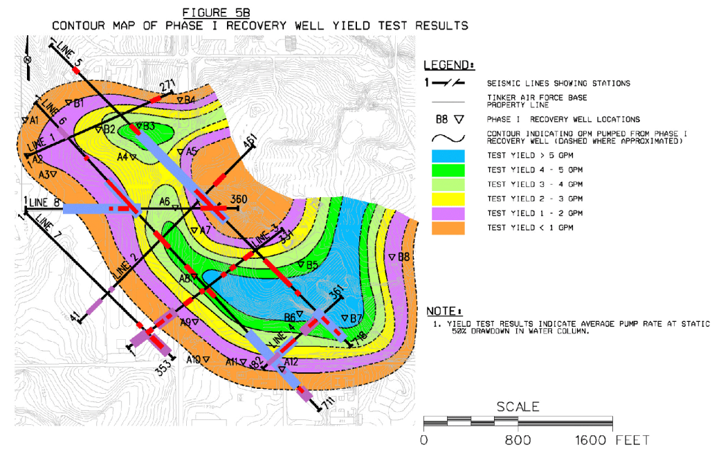
Figure 5: Location of Significant Seismic Anomalies and Correlation with Well Yields[2]
