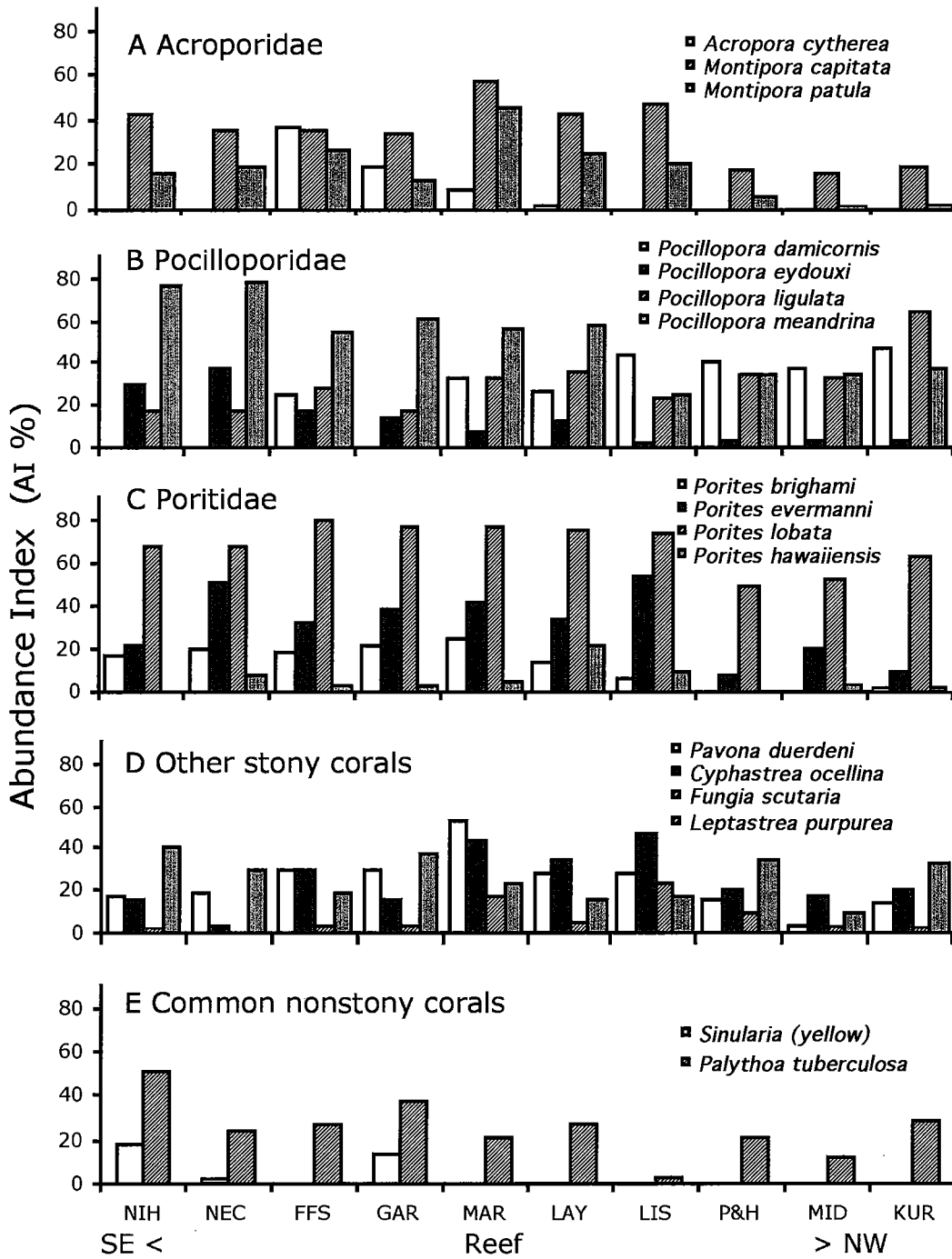
FIGURE 2. Abundance indices for common corals, based on sums of abundance indices for each species on each reef in Appendixes 1 and 2. Reefs arranged from southeast (SE) to northwest (NW). Reef codes from Table 1.
