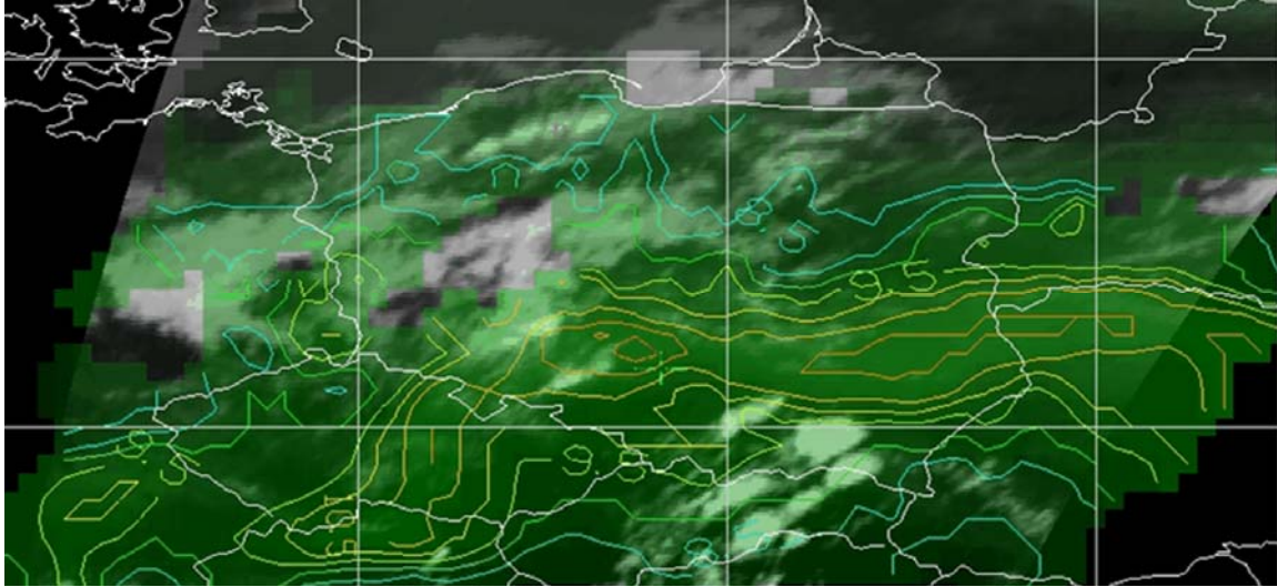
Figure 2 – Thermal IR image and NearCast of 840 hPa Mixing Ratio valid 1200 UTC on 20 July 2007, 3 hours prior to tornado formation.
