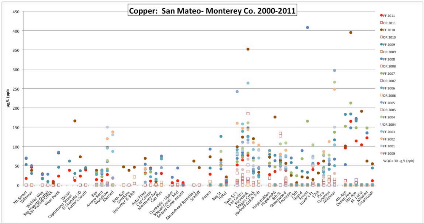
Figure 8. Total copper results for the Dry Run and time series averages for First Flush. For two sites, Twins in Monterey and 17 th in Pacific Grove, results are based upon one sample. All sites grouped by city from north to south- Montara, Moss Beach, El Granada, Santa Cruz, Capitola, Pajaro (Monterey County), Seaside, Monterey, Pacific Grove and Carmel.
