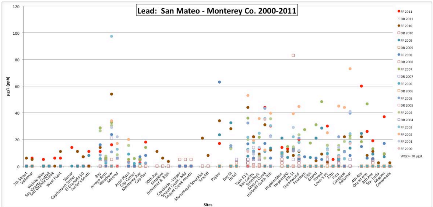
Figure 9. Total lead results for all sites for Dry Run and time series averages for First Flush. For two sites, Twins in Monterey and 17 th in Pacific Grove, results are based upon one sample. All sites grouped by city from north to south- Montara, Moss Beach, El Granada, Santa Cruz, Capitola, Pajaro (Monterey County), Seaside, Monterey, Pacific Grove and Carmel.
