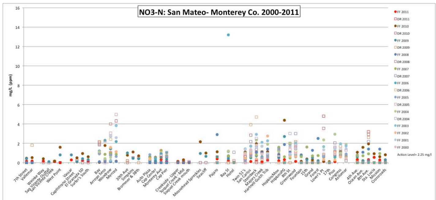
Figure 2. Results for Nitrate-N for the Dry Run and time series averages for First Flush. For two sites, Twins in Monterey and 17 th in Pacific Grove, results are based upon one sample. All sites grouped by city from north to south- Montara, Moss Beach, El Granada, Santa Cruz, Capitola, Pajaro (Monterey County), Seaside, Monterey, Pacific Grove and Carmel.
