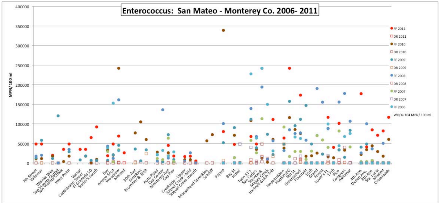
Figure 6. Results for enterococcus for the Dry Run and time series averages for First Flush. For two sites, Twins in Monterey and 17 th in Pacific Grove, results are based upon one sample. All sites grouped by city from north to south- Montara, Moss Beach, El Granada, Santa Cruz, Capitola, Pajaro (Monterey County), Seaside, Monterey, Pacific Grove and Carmel.
