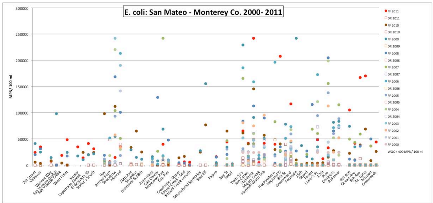
Figure 5. E.coli results for the Dry Run and time series averages for First Flush. For two sites, Twins in Monterey and 17 th in Pacific Grove, results are based upon one sample. All sites grouped by city from north to south- Montara, Moss Beach, El Granada, Santa Cruz, Capitola, Pajaro (Monterey County), Seaside, Monterey, Pacific Grove and Carmel.
