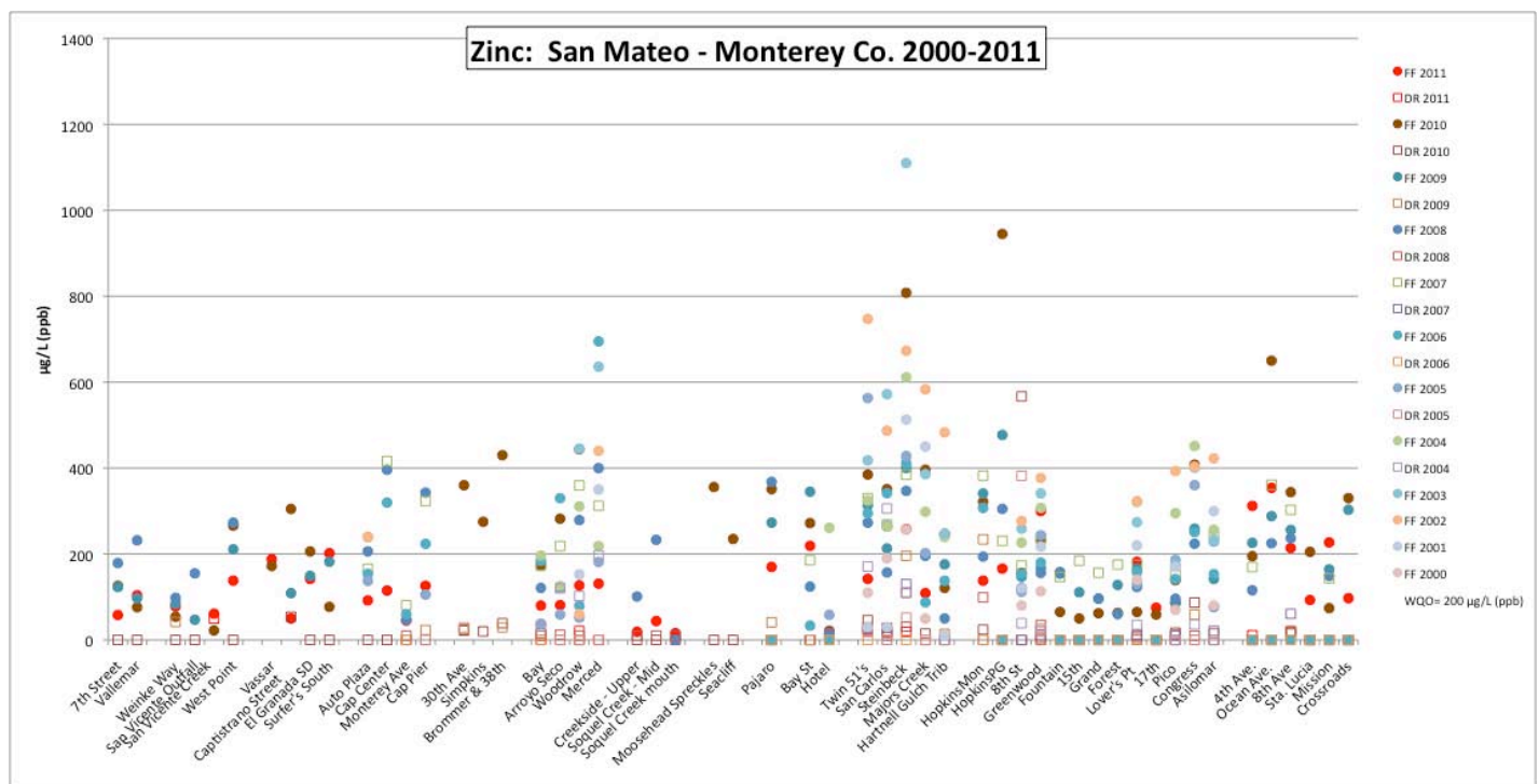
Figure 7. Total zinc results for all sites for Dry Run and time series averages for First Flush. For two sites, Twins in Monterey and 17 th in Pacific Grove, results are based upon one sample. All sites grouped by city from north to south- Montara, Moss Beach, El Granada, Santa Cruz, Capitola, Pajaro (Monterey County), Seaside, Monterey, Pacific Grove and Carmel.
