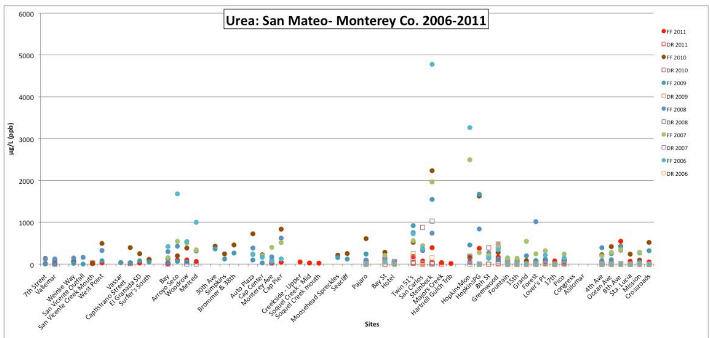
Figure 4. Urea results for the Dry Run and First Flush. All sites grouped by city from north to south- Montara, Moss Beach, El Granada, Santa Cruz, Capitola, Pajaro (Monterey County), Seaside, Monterey, Pacific Grove and Carmel.
