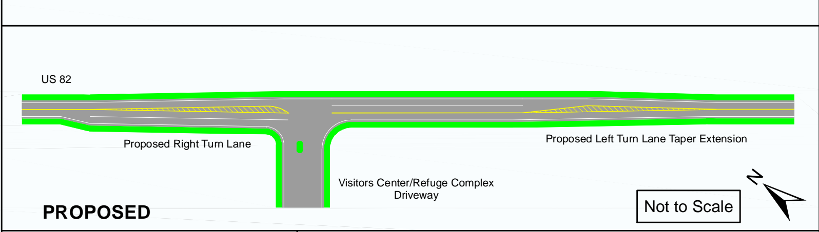
Figure 5.3: Potential Turn-Lane Improvements at Refuge Visitors Center
