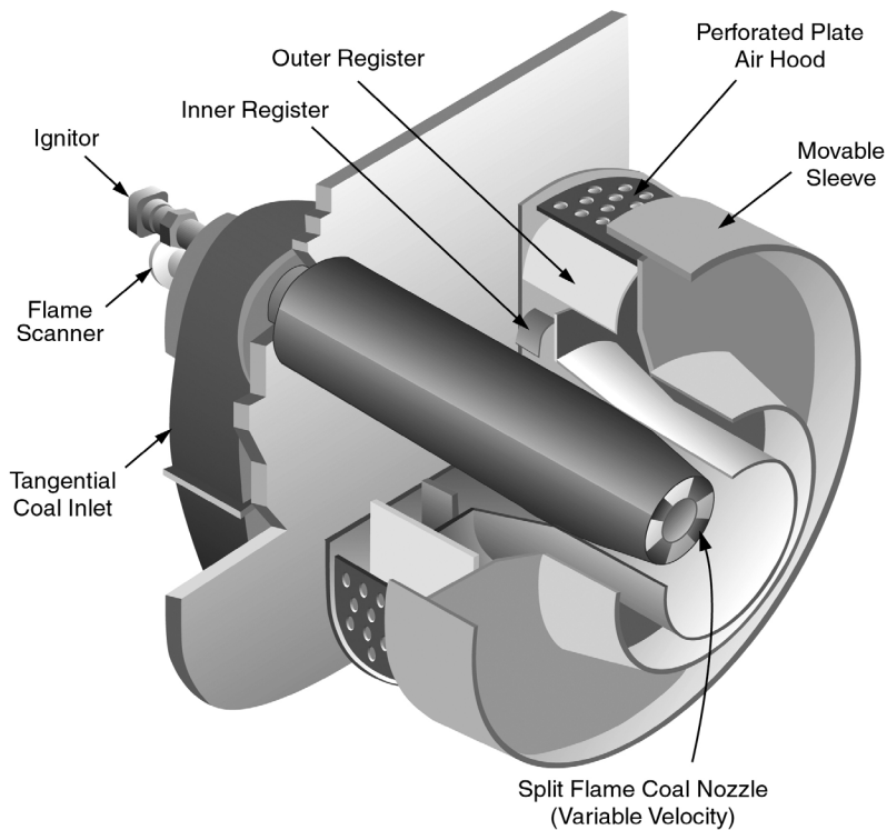
Figure 3. Controlled Flow/Split Flame Low NO x Burner
