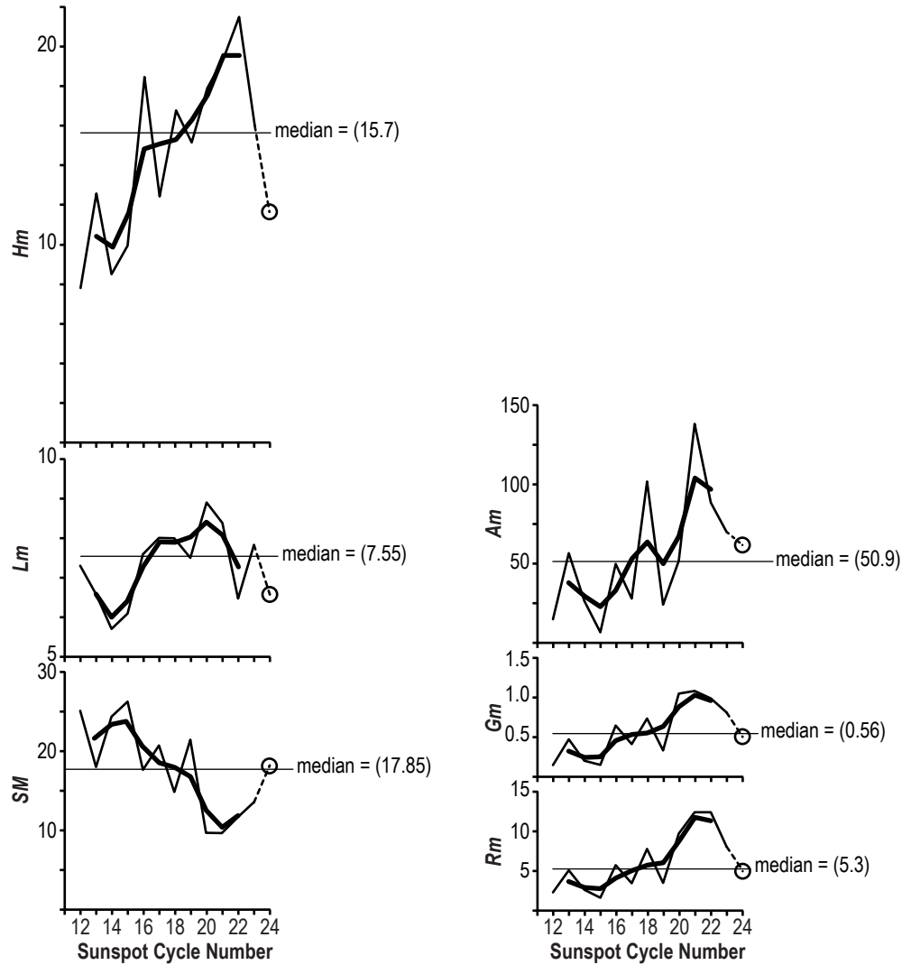
Figure 1. Cyclic variation of R_m , G_m , A_m , SM , L_m , and H_m for cycles 12–24. Circled values represent tentative values for cycle 24, which may change for R_m , G_m , A_m , and SM , but are considered valid for L_m and H_m .
