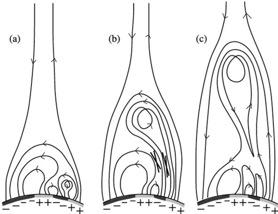
Figure 1. Schematic of the magnetic-arch-blowout model for the production of a streamer-puff over-and-out CME (from Bemporad et al 2005). A compact sheared-core arcade explodes up the leg of an outer loop of a streamer arcade. Reconnection of the legs of the escaping field unleashes an expanding “plasmoid” that becomes the core of the CME. For the events of Bemporad et al (2005), the rightmost light band at the base represents the positive-polarity sunspot and the adjacent short dark band represents the island of negative flux that was the seat of the compact ejective flares.
