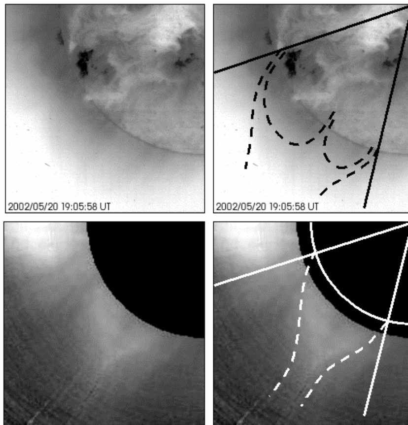
Figure 4. Evidence that the base of our streamer spanned both the magnetic arcade over the filament and the magnetic arcade over the filament channel, that the flare site was embedded in the northern flank of the magnetic arcade over the filament, and that the streamer was unipolar (had no extended current sheet) (see text). Upper left: EIT Fe XV 284 Å negative image taken a few hours after the flare and the coronal dimming had faded out. Upper right: Same image as on the left, with dashed arches outlining emission from the two arcades, dashed open curves indicating the span of the streamer base needed to cover both arcades, and solid radial lines showing the needed angular span. Lower left: Visible-light image obtained by the Mauna Loa Solar Observatory Mark-4 Coronagraph on the day before our event. Lower right: Same image as on the left, with dashed curves tracing the northern and southern sides of the streamer, solid quarter circle marking the limb, and solid radial lines showing the approximate angular span of the streamer base at the limb.
