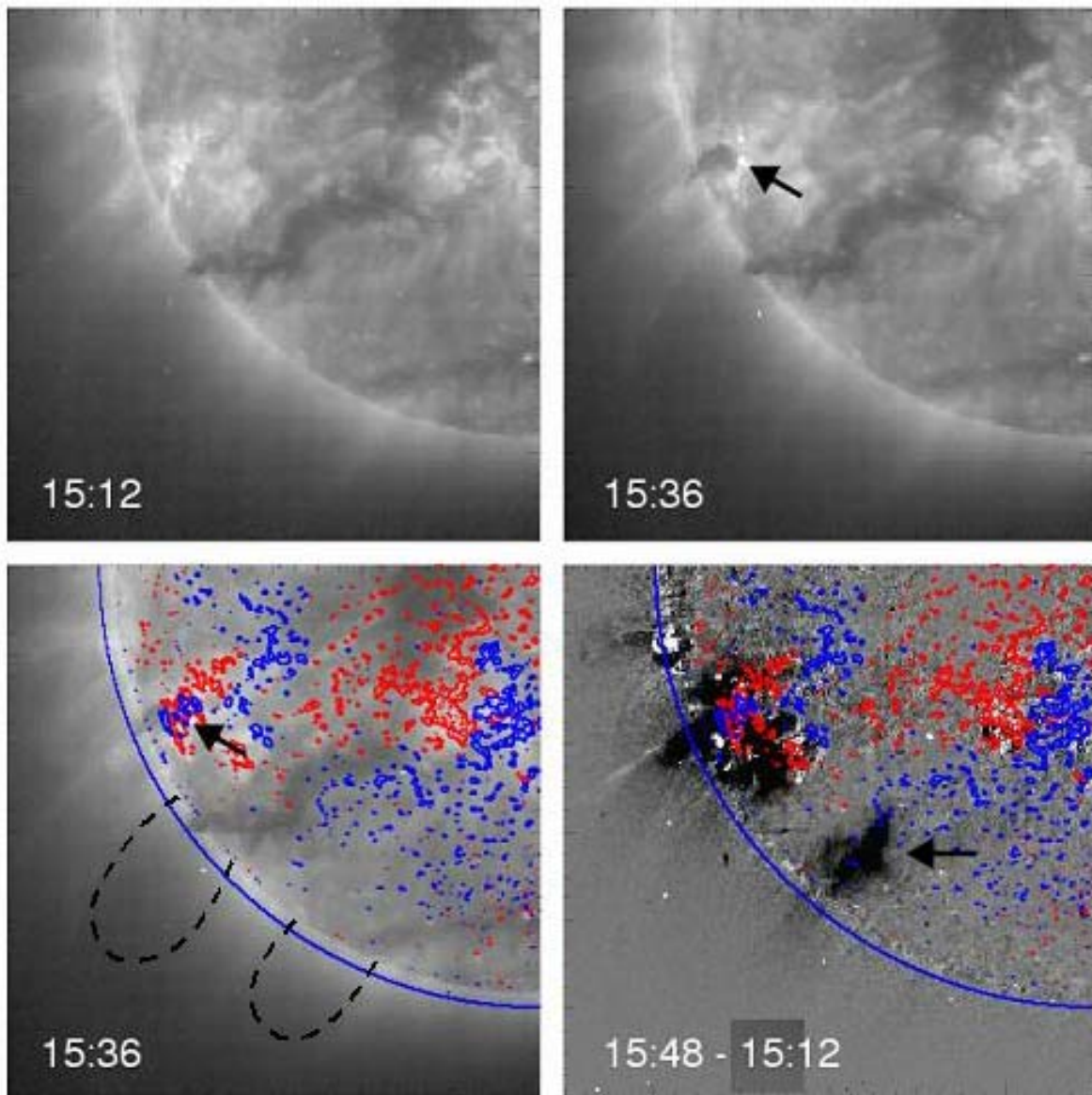
Figure 3. The compact ejective flare, the coronal dimming footprint of the streamer-puff CME, and their magnetic setting. Upper left: EIT Fe XII 195 Å image at 15:12 UT, minutes before the flare. Upper right: EIT Fe XII image showing the ejective flare (arrow) in progress at 15:36 UT, and showing no change in either the filament south of the flare or in the polar-crown filament channel farther south. Lower left: The 15:36 UT EIT image registered with an MDI magnetogram, showing that the flare was in an emerging active region. The dashed arches over the filament and over the filament channel outline faint coronal cavities. Lower right: EIT Fe XII difference image (the image at 15:48 UT minus the image at 15:12 UT) registered with the magnetogram, showing the coronal-dimming footprint of the CME.
