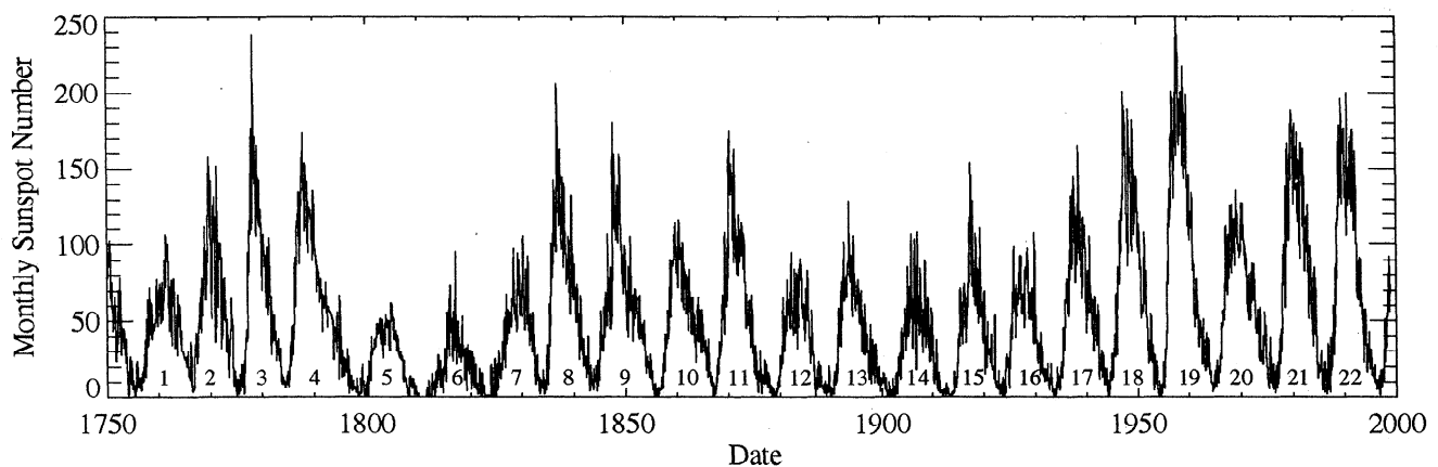
Figure 1. Monthly averaged International Sunspot Number as a function of time. The individual sunspot cycles (numbered along the bottom) vary in amplitude, duration, and shape.
