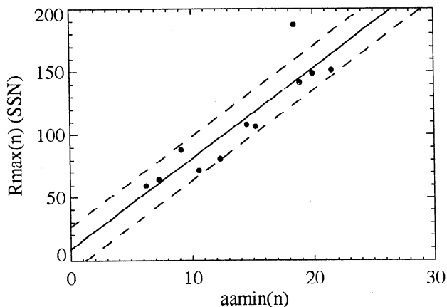
Figure 10. Ohl's Method for cycles 12-22. The maximum amplitude of a cycle is proportional to the aa index at the minimum preceding it. This relationship is shown with the solid line. The standard deviation about this line is shown with the dashed lines.
