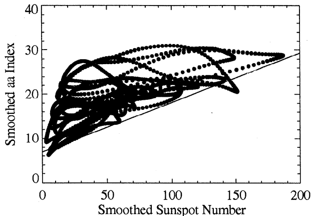
Figure 11. Our version of Feynman's Method for determining the dependence of the aa index upon the current sunspot number. A line is fit through the lowest values of the smoothed monthly aa index from each of 20 bins in smoothed monthly sunspot number.
