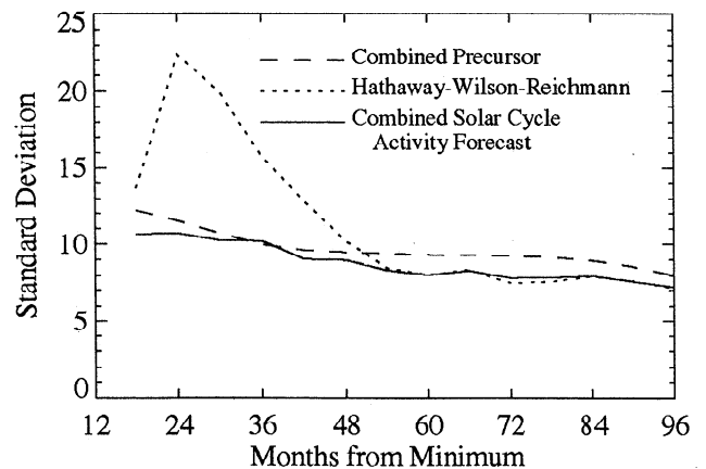
Figure 16. The standard deviation between the observed (24-month FWHM Gaussian filtered) sunspot numbers and those predicted by the Combined Precursor, the Hathaway- Wilson-Reichmann method, and the Combined Solar Cycle Activity Forecast Method. The Combined Solar Cycle Activity Forecast Method provides the best estimate of future sunspot numbers.
