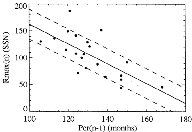
Figure 7. The Amplitude-Period Method for cycles 2-22. The maximum amplitude of a cycle is inversely proportional to the period of the preceding cycle. This relationship is shown with the solid line. The standard deviation about this line is shown with the dashed lines.
