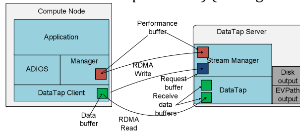
Figure 11. DataTap architecture
