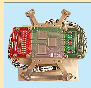
This is a photograph of the TIRS focal plane showing the QWIPs detector arrays. The three squares in the center of the circuit board are QWIPs arrays, which are gallium arsenide semiconductor chips. Each QWIP array contains 327,680 detectors.
