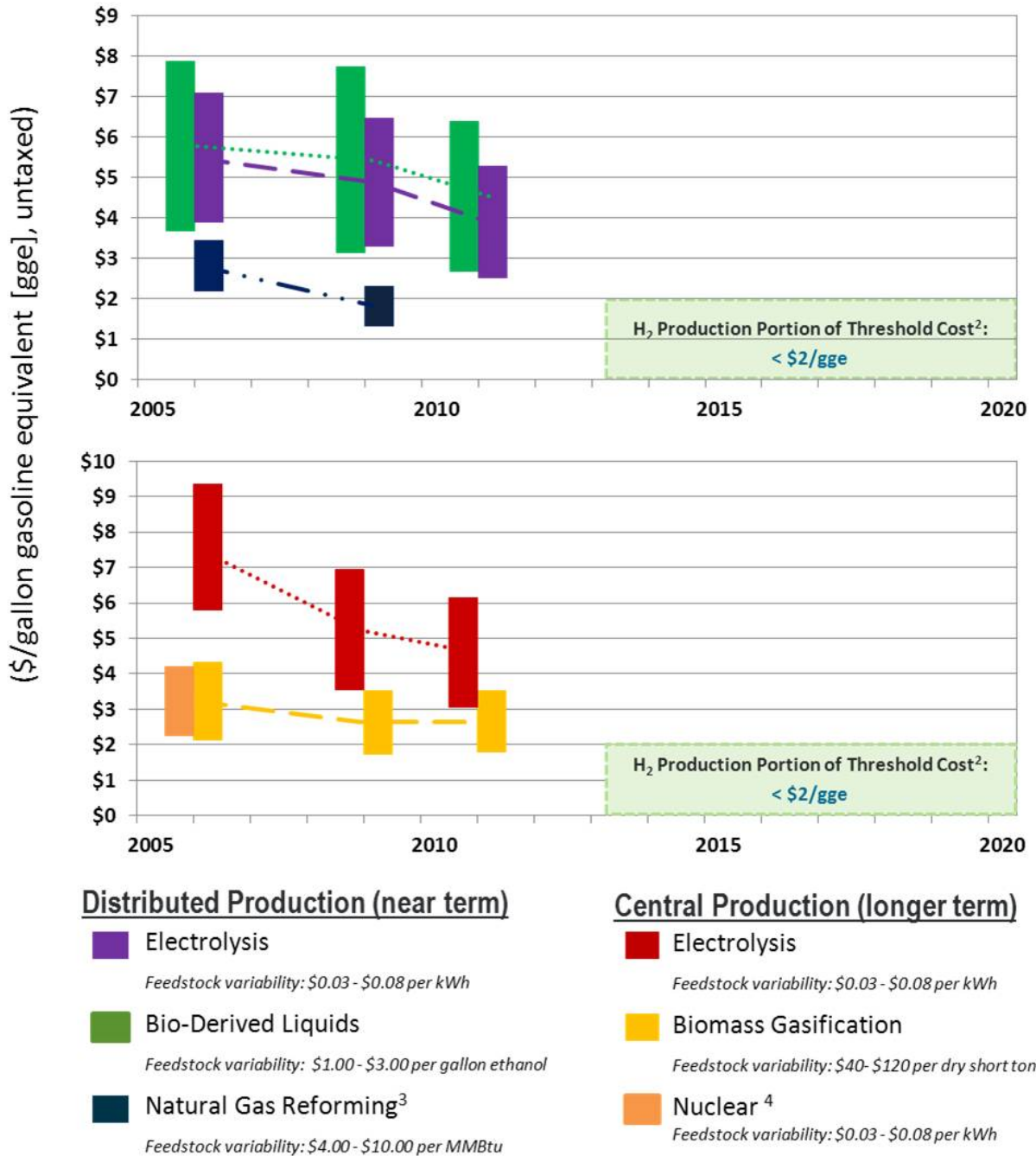
Figure 2: Projected High-Volume Cost of Hydrogen Production 1 —Status
