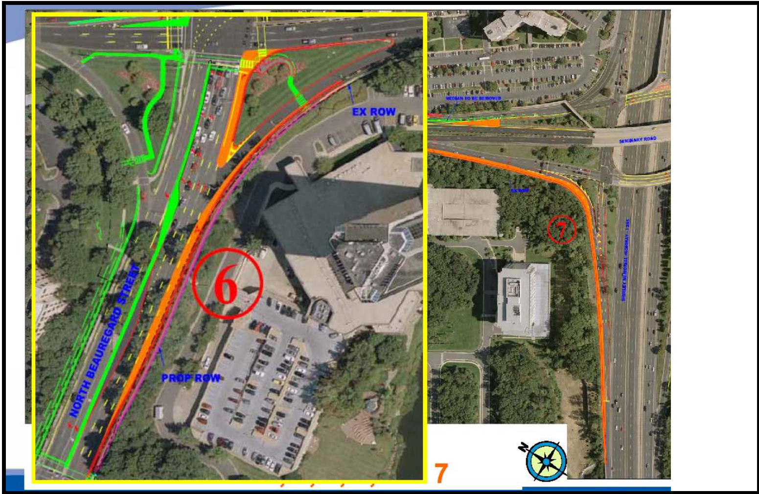
Location 6 Widen northbound Beauregard Street between Mark Center Drive and Seminary Road to provide a dedicated right turn lane at the northbound approach to Seminary Road after the direct connect ramp from northbound Beauregard Street to eastbound Seminary Road. Reconfigure the intersection to allow the three to two through lane drop at the new dedicated right turn lanes in lieu of one of the left turn lanes and provide two dedicated left turn lanes.
