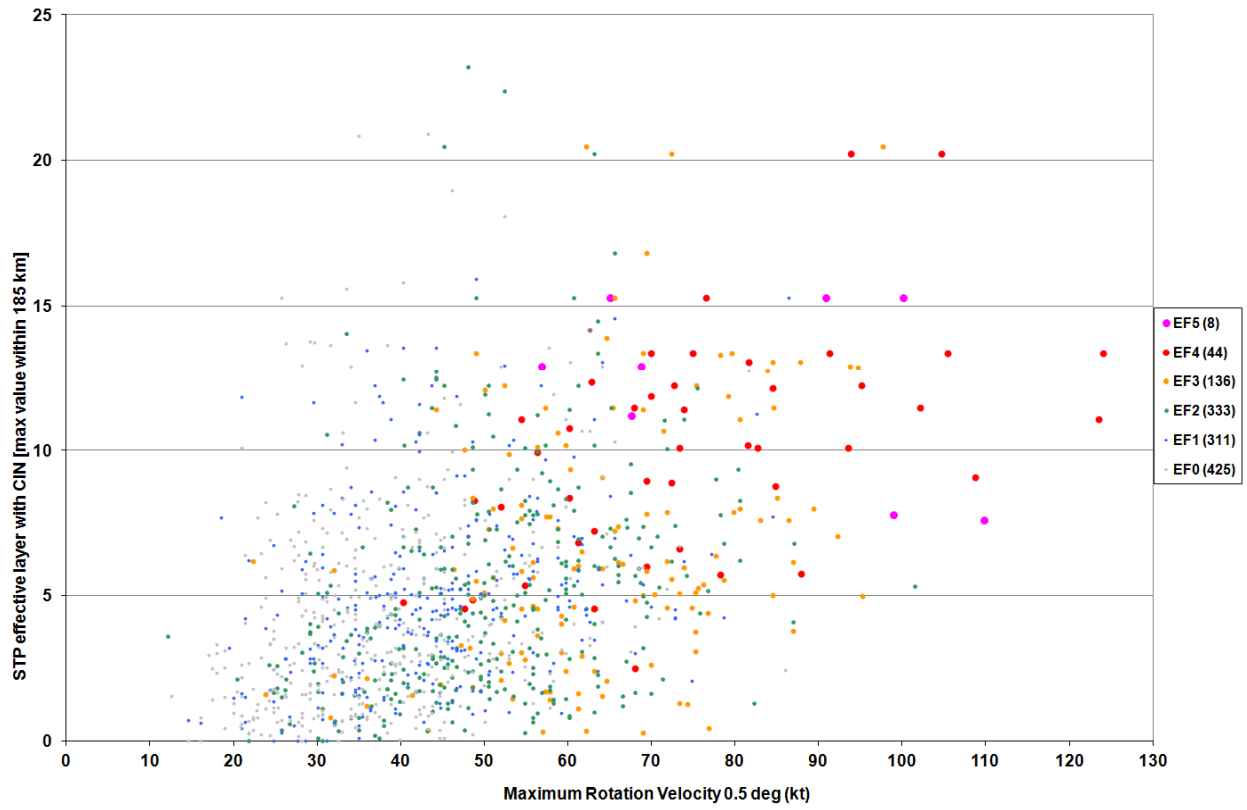
Figure 11. As in Fig. 10 except for RM.
