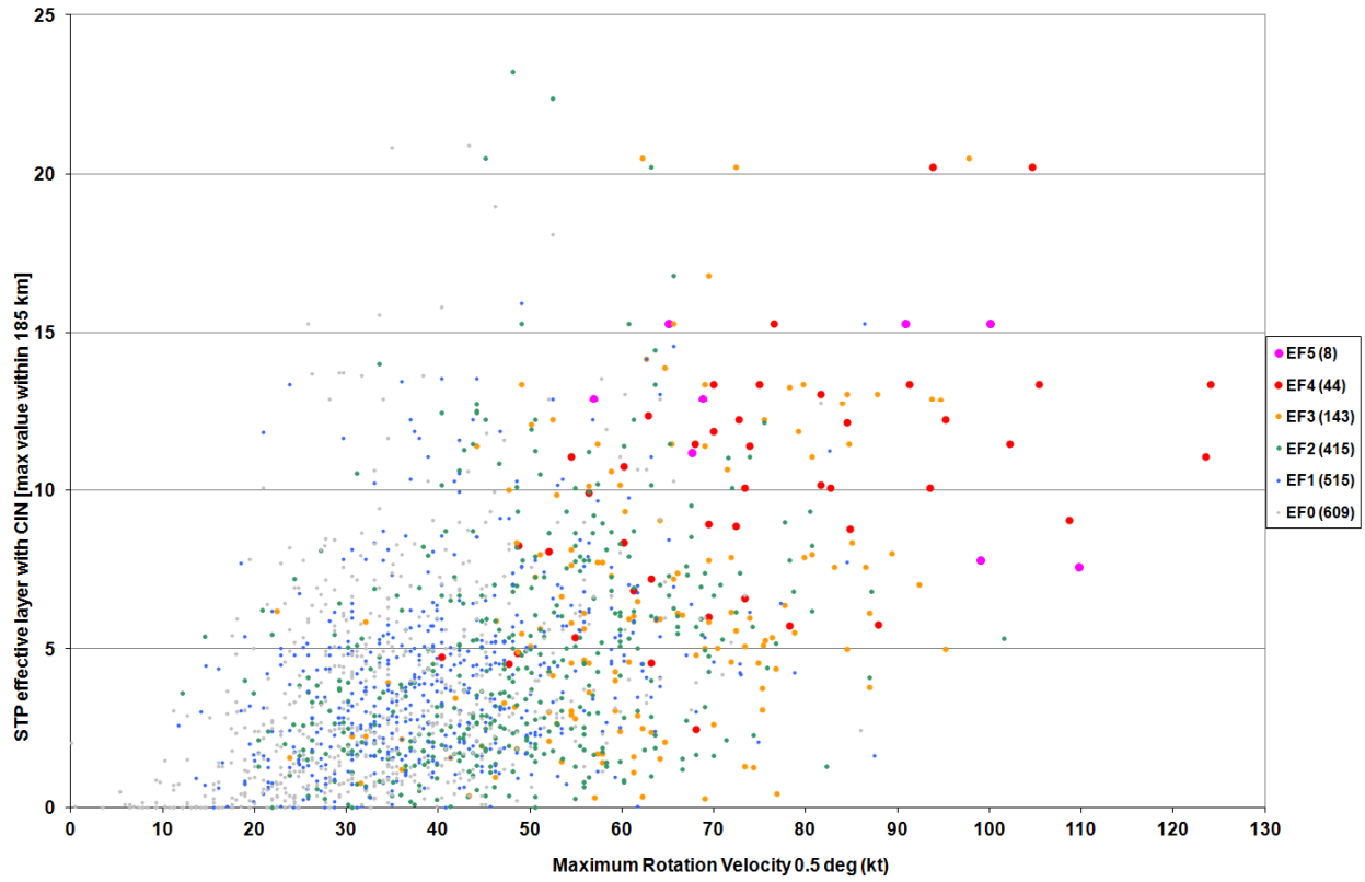
Figure 10. Scatterplot of \geq EF2 2009-2010 and 2011 EF0-EF5 tornado events by EF-scale rating (legend; middle right) of 0.5 degree peak rotational velocity (kt) x-coordinate vs. STP effective layer (max value within 185 km).
