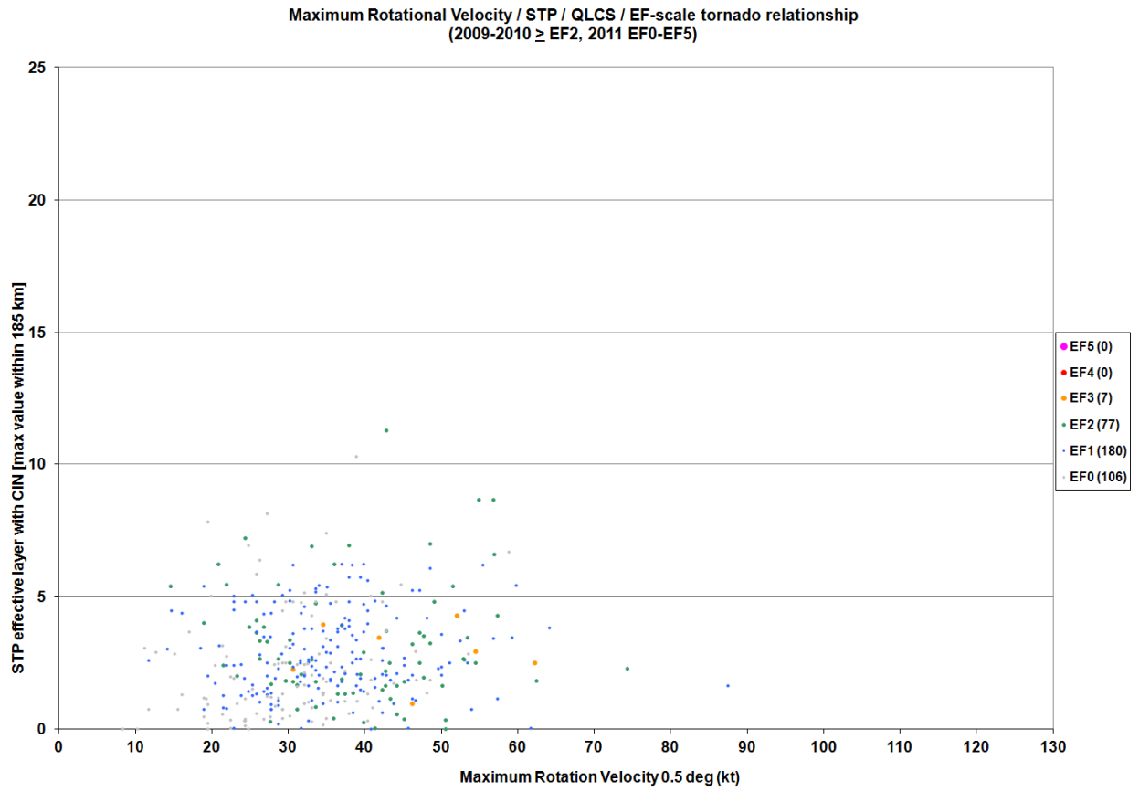
Figure 12. As in Fig. 10 except for QLCS.
