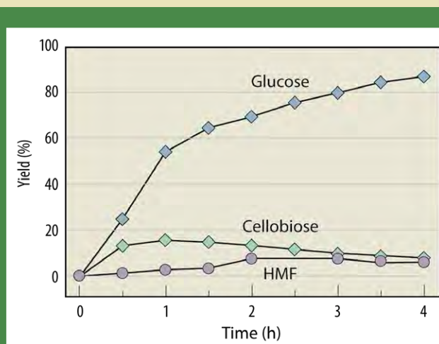
Chemical Hydrolysis of Cellulose Achieves High Glucose Yields. Applying this new chemical approach to the hydrolysis of pure cellulose results in glucose yields approaching 90% in just a few hours. Yields of unwanted by-products such as HMF (5-hydroxymethylfurfural, an inhibitor of microbial fermentation) and cellobiose (a molecule consisting of two linked glucose subunits) were minimal. [Image from Binder and Raines 2010]
