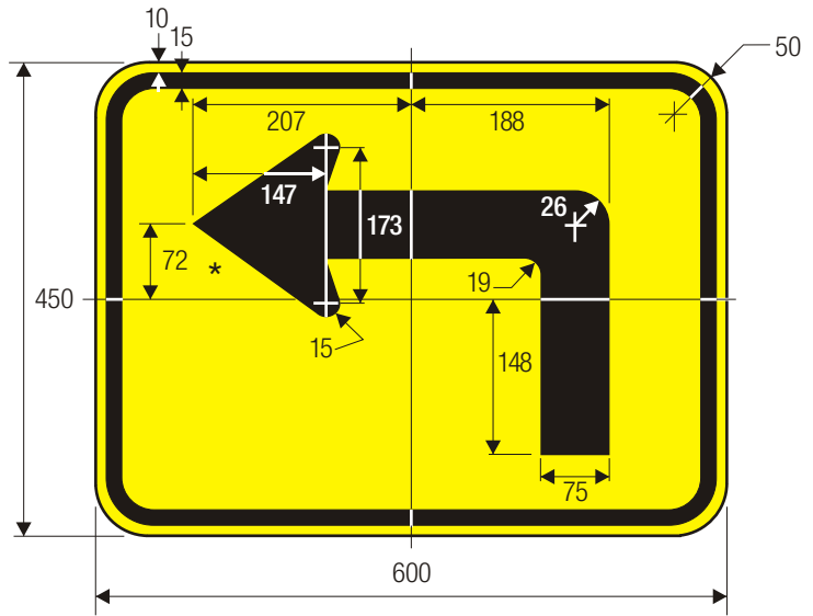
W16-6pL ARROW PLAQUE
