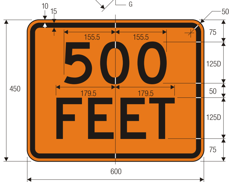
W2-16 DISTANCE (2 LINE) (ENGLISH)
