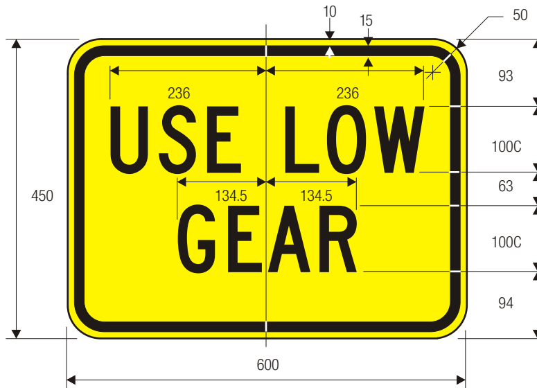
W7-2 HILL PLAQUE
