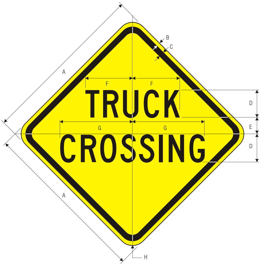
W8-6 TRUCK CROSSING
