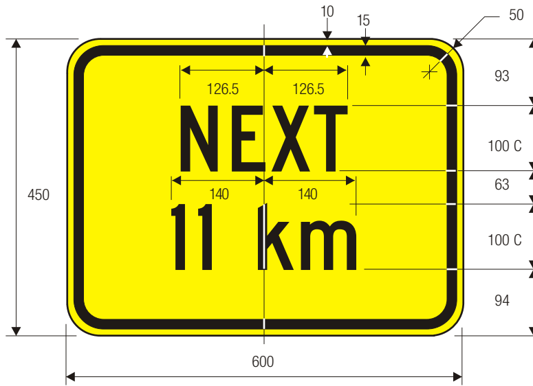
W7-3a Metric HILL PLAQUE
