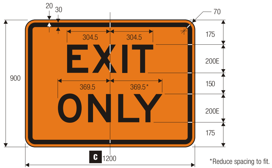
E5-3 EXIT ONLY
