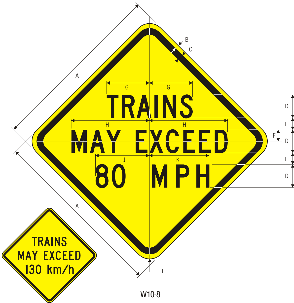
W10-8 TRAINS MAY EXCEED XX MPH
