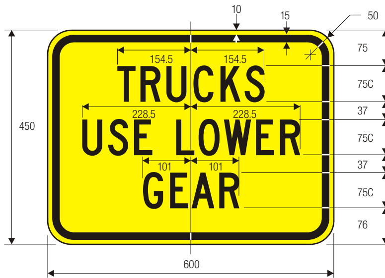
W7-2b HILL PLAQUE
