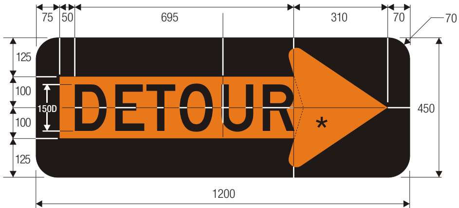
M4-10R DETOUR (INSIDE ARROW)
