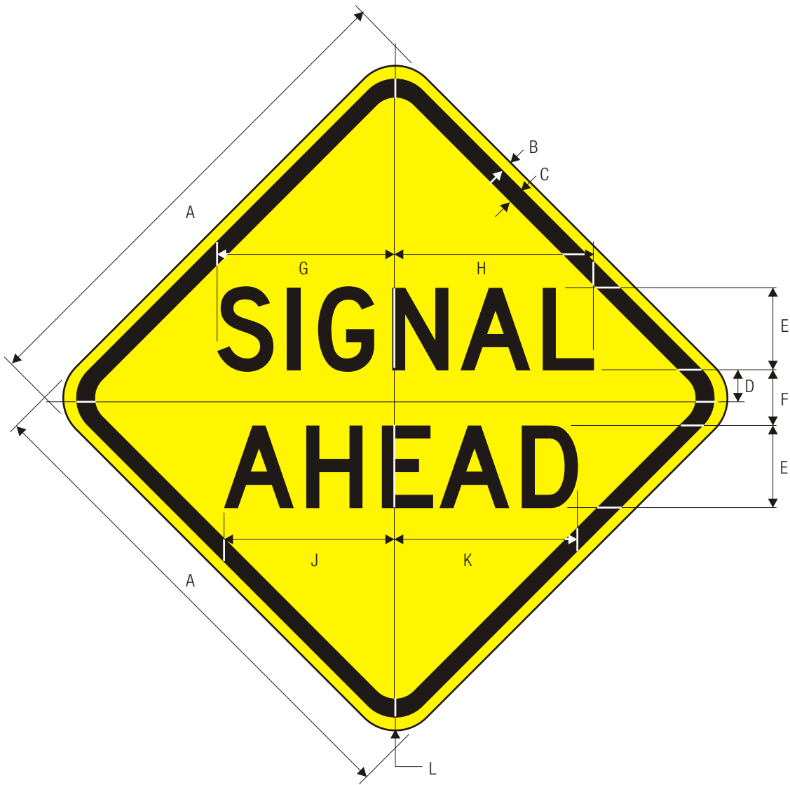
W3-3a SIGNAL AHEAD
