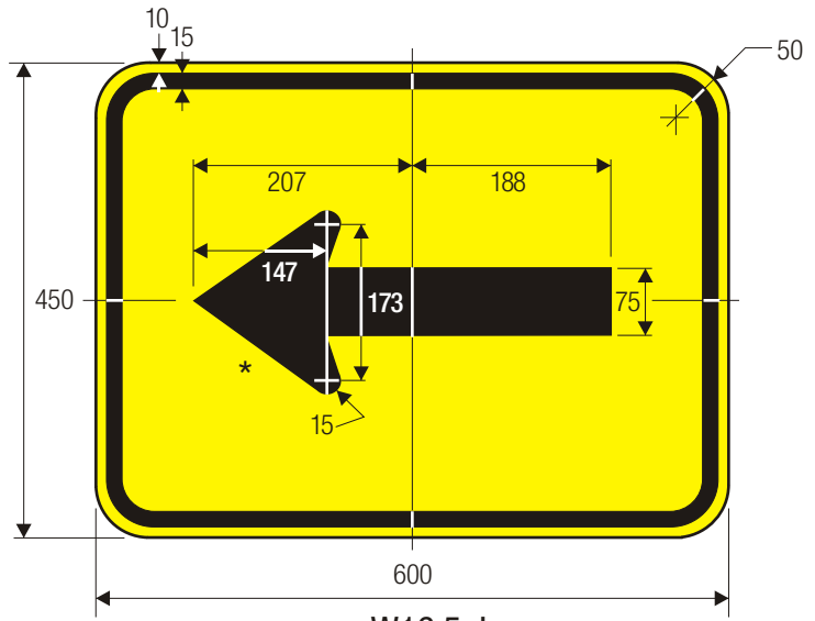
W16-5pL ARROW PLAQUE
