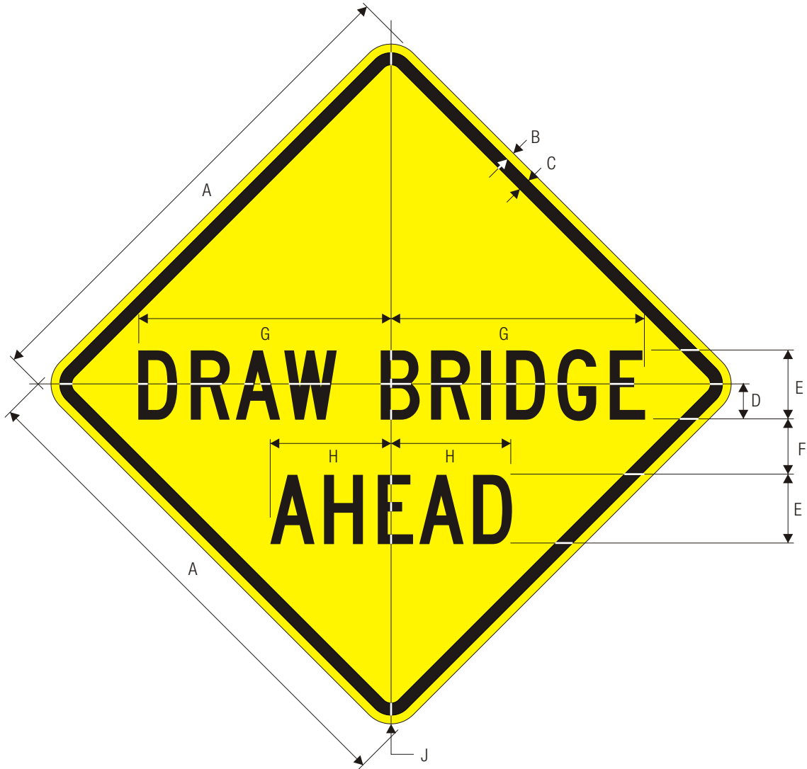
W3-6 DRAW BRIDGE AHEAD
