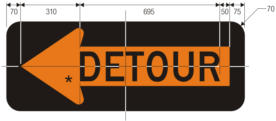
M4-10L DETOUR (INSIDE ARROW)
