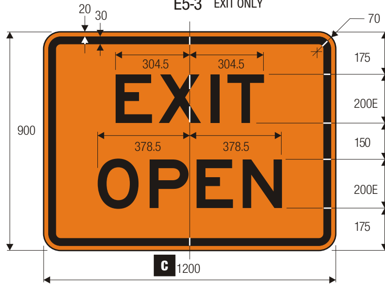
E5-2 EXIT OPEN
