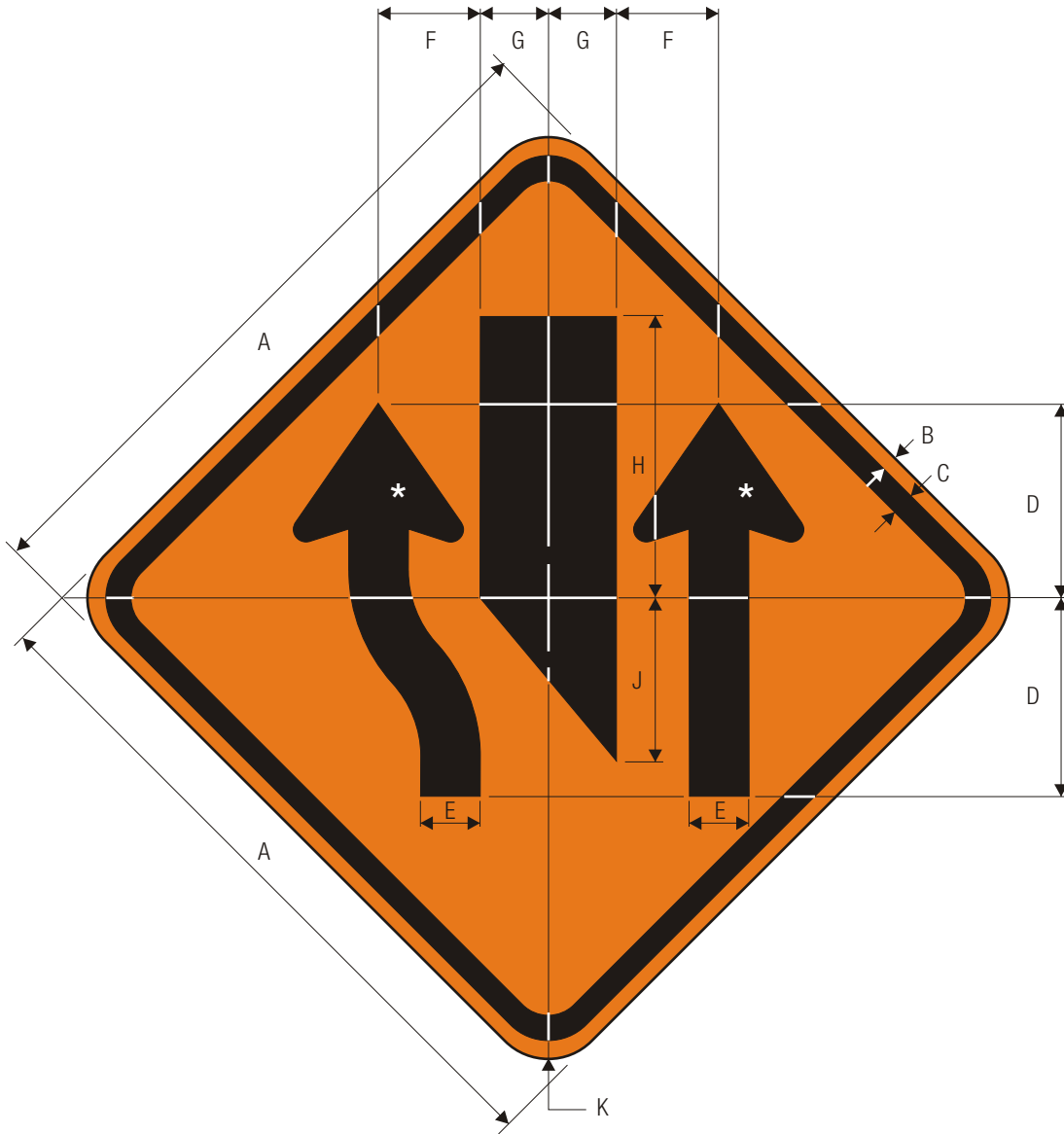
W9-3a CENTER LANE CLOSED
