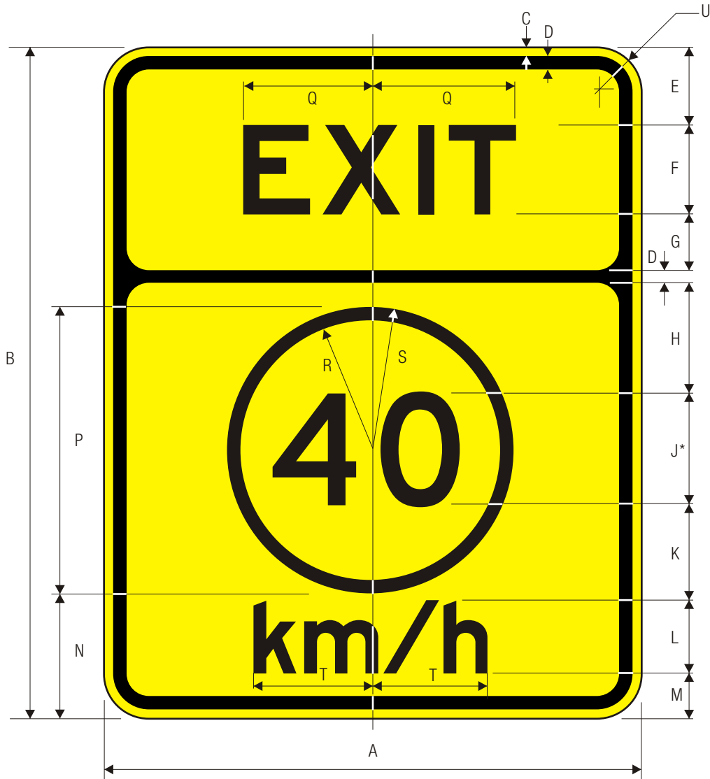
W13-2 ADVISORY EXIT SPEED (METRIC)
