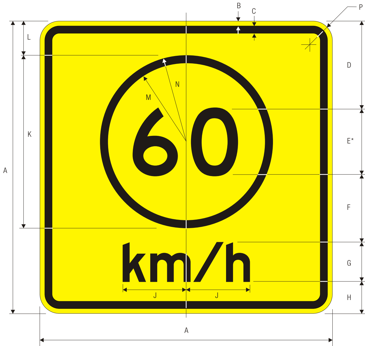
W13-1 ADVISORY SPEED (METRIC)
