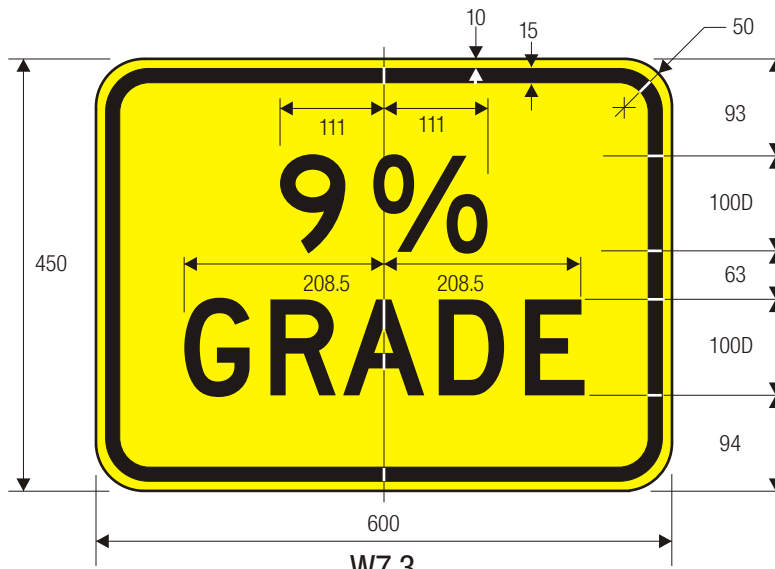
W7-3 HILL PLAQUE
