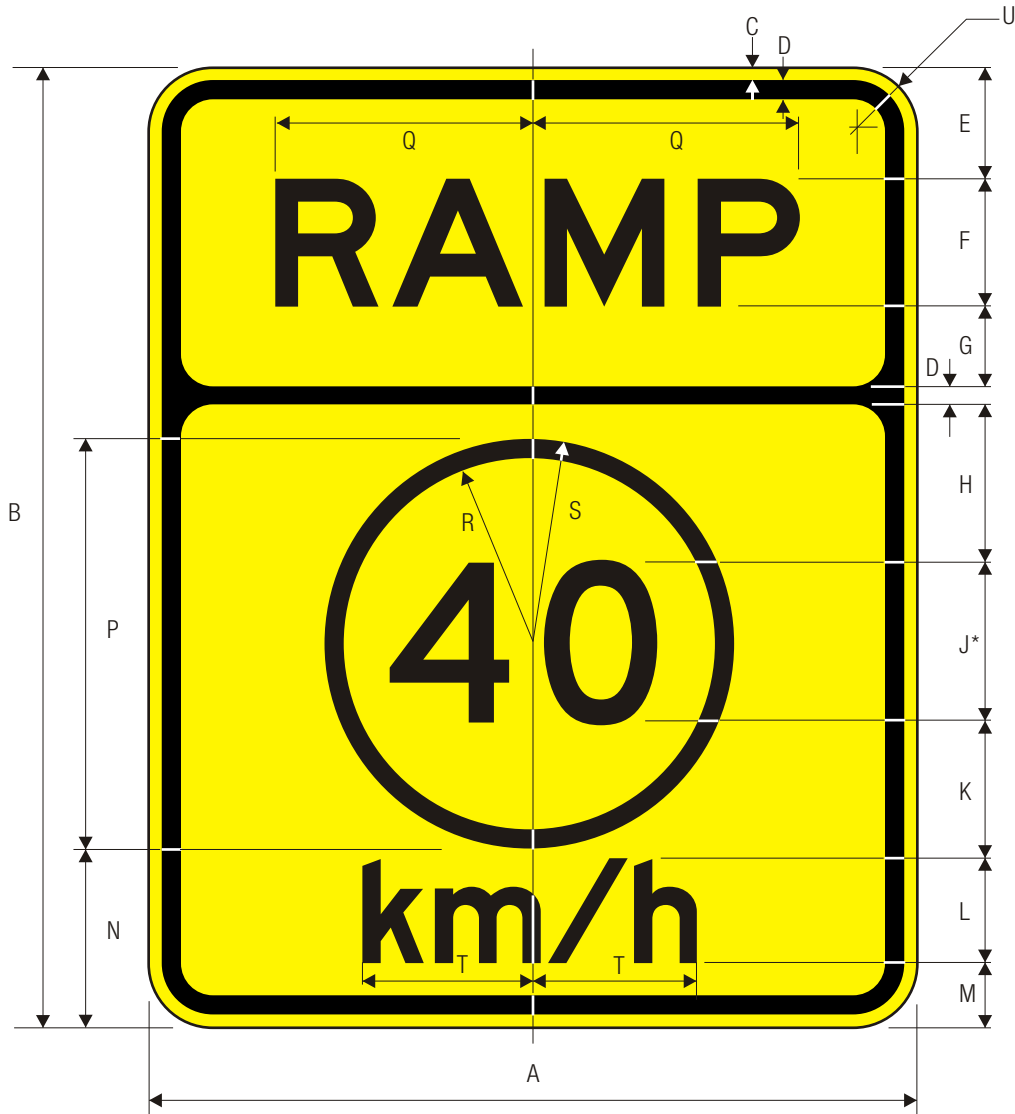
W13-3 ADVISORY RAMP SPEED
