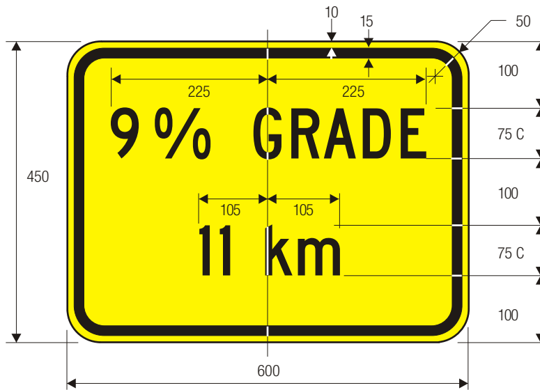
W7-3b Metric HILL PLAQUE
