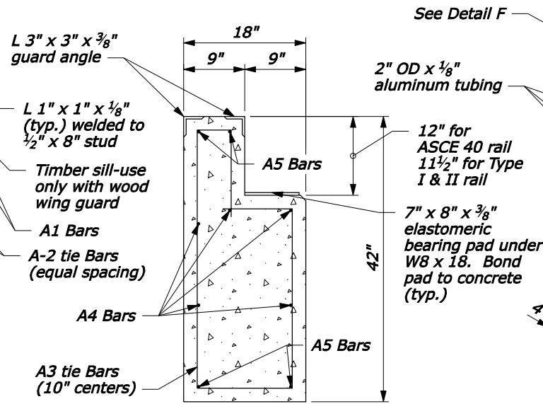
END SUPPORT DETAIL (#4 Reinforcing Bars)
