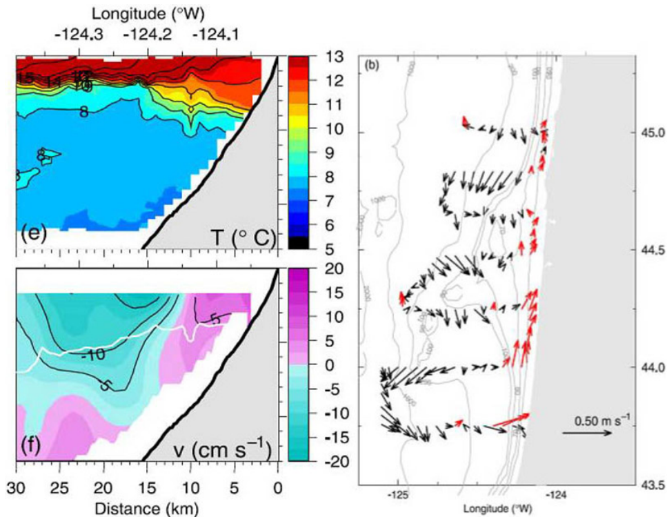
Figure 3.6-1. (Left) Cross-shelf section of temperature (top) and alongshore velocity (bottom) at 45^\circ N on August 25 during a 2-day reversal of winds from southward to northward during August 24-25, 2001. (Right) Velocity vectors at 25-m depth from shipboard Acoustic Doppler Current Profiler (ADCP) measurements during the same 2-day period.
