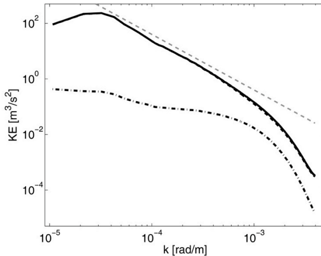
Figure 3.4-2. Horizontal wavenumber spectrum of surface horizontal eddy kinetic energy K(k_h) in a numerical simulation of an idealized Subtropical Eastern Boundary Current: total (solid line), horizontally non-divergent (i.e., geostrophic) component (dark dash), and divergent (ageostrophic) component (dash-dot). Also shown is a k^{-2} power-law (light dash), which is an approximate fit in the submesoscale range for k_h larger than the mesoscale spectrum peak. Note that most of the energy is geostrophic throughout this range, even though local breakdowns of geostrophic balance do occur. (Capet et al., 2008c)
