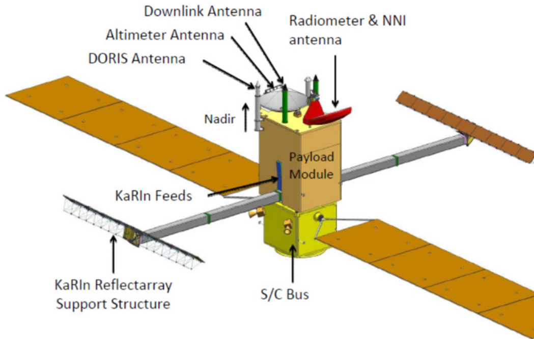
Figure 7.3-1. Proposed SWOT satellite and payload configuration.
