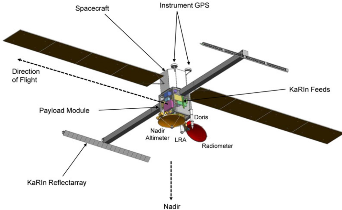
Figure 7.2-1. SWOT spacecraft concept: current design.
