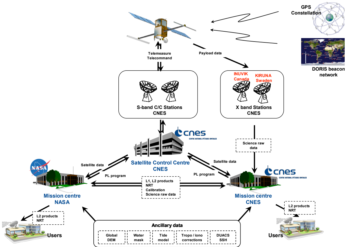
Figure 7.4-1. Overall Ground System architecture, including links to spacecraft.
