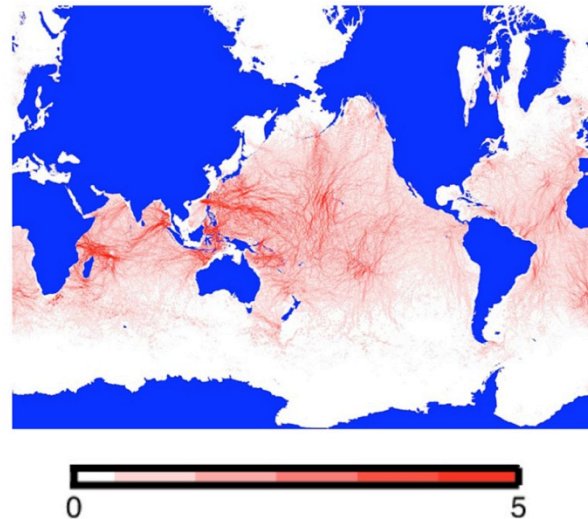
Figure 5.1-3. Amplitude (cm) of M_2 internal tide signature in steric SSH of HYbrid Coordinate Ocean Model (HYCOM) experiment with 32 layers, 1/12.5^\circ horizontal resolution, horizontally nonuniform stratification, and wind-, buoyancy-, and M_2 -forcing included. From Arbic et al. (2010).
