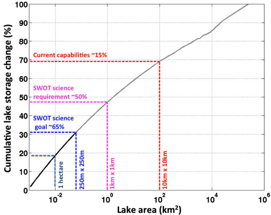
Figure 4-5. Anticipated improvement in global storage changes from SWOT (Biancamaria et al., 2009)
