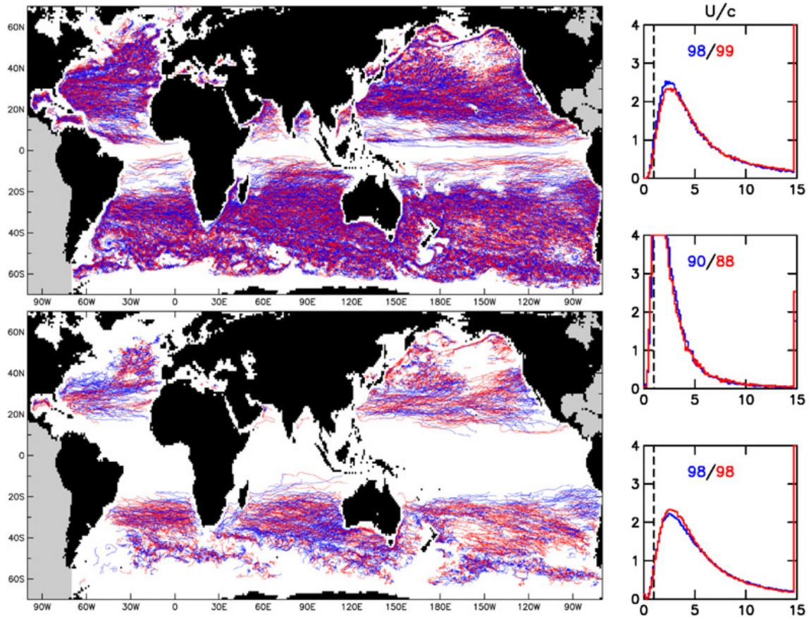
Figure 3.1-1. The trajectories of cyclonic (blue) and anticyclonic (red) eddies with lifetimes longer than 4 months (top left) and longer than 1 year (bottom left). Histograms of the nonlinearity parameter U/c , where U is the maximum fluid speed within an eddy and c is its translation speed, are shown in the right panels for cyclonic (blue curves) and anticyclonic (red curves) eddies in three different latitude bands. The blue and red numbers in each panel indicate the percentages of cyclonic and anticyclonic eddies, respectively, with U/c > 1 . (After Chelton et al., 2011.)
