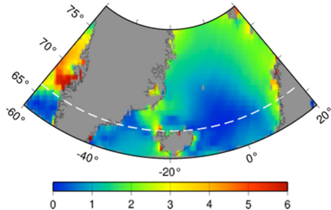
Figure 5.1-1. Maximum differences (cm) between the S2 tide models of FES2004 and TPXO7.1 for the seas near Greenland. The white dashed line marks 66^\circ N, the northernmost latitude reached by the TOPEX/Poseidon and Jason satellites. Large model differences south of 66^\circ are mostly coastal problems; differences increase markedly north of 66^\circ . Both models used data from ERS-1/2 altimetry north of 66^\circ , but those data reveal nothing about S2 owing to the sun-synchronous orbits. SWOT should remedy this situation.
