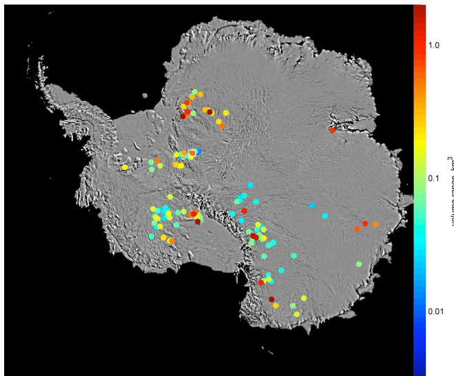
Figure 5.3-4. Locations and volume-range estimates for 124 active lakes under the Antarctic ice sheet found in Smith et al., 2009, shown as points color-coded by the volume range.
