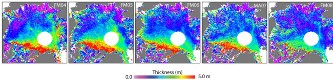
Figure 5.4-2. Sea ice thickness fields from five ICESat campaigns (2004–2008). http://rkwok.jpl.nasa.gov/icesat/index.html ).
