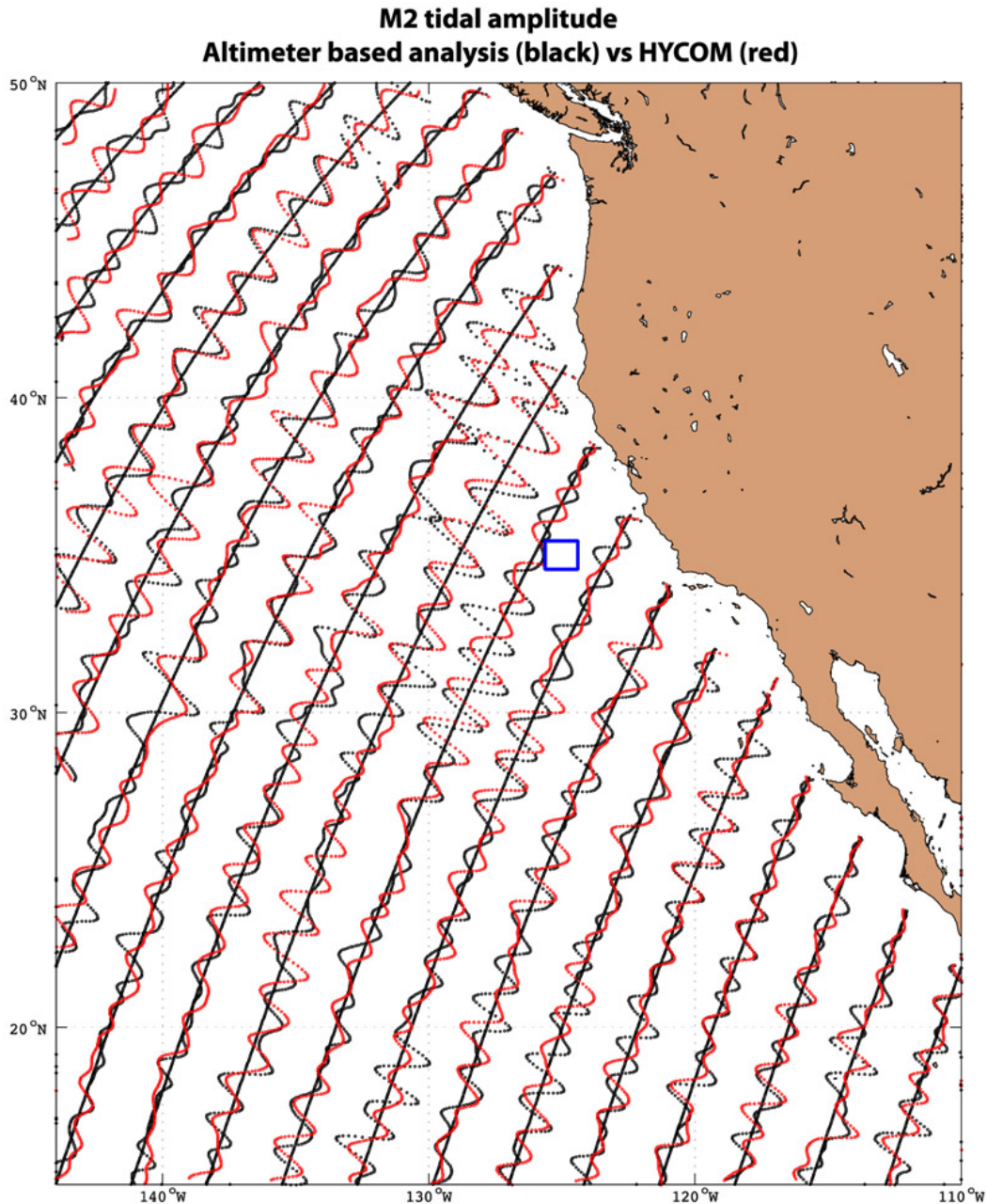
Figure 5.1-5. Internal tide perturbations to amplitude of M_2 sea surface elevation along ascending altimetric tracks in North Pacific. Blue box is a site considered for the AirSWOT mission concept. (Plot courtesy Jay Shriver, 2011.)
