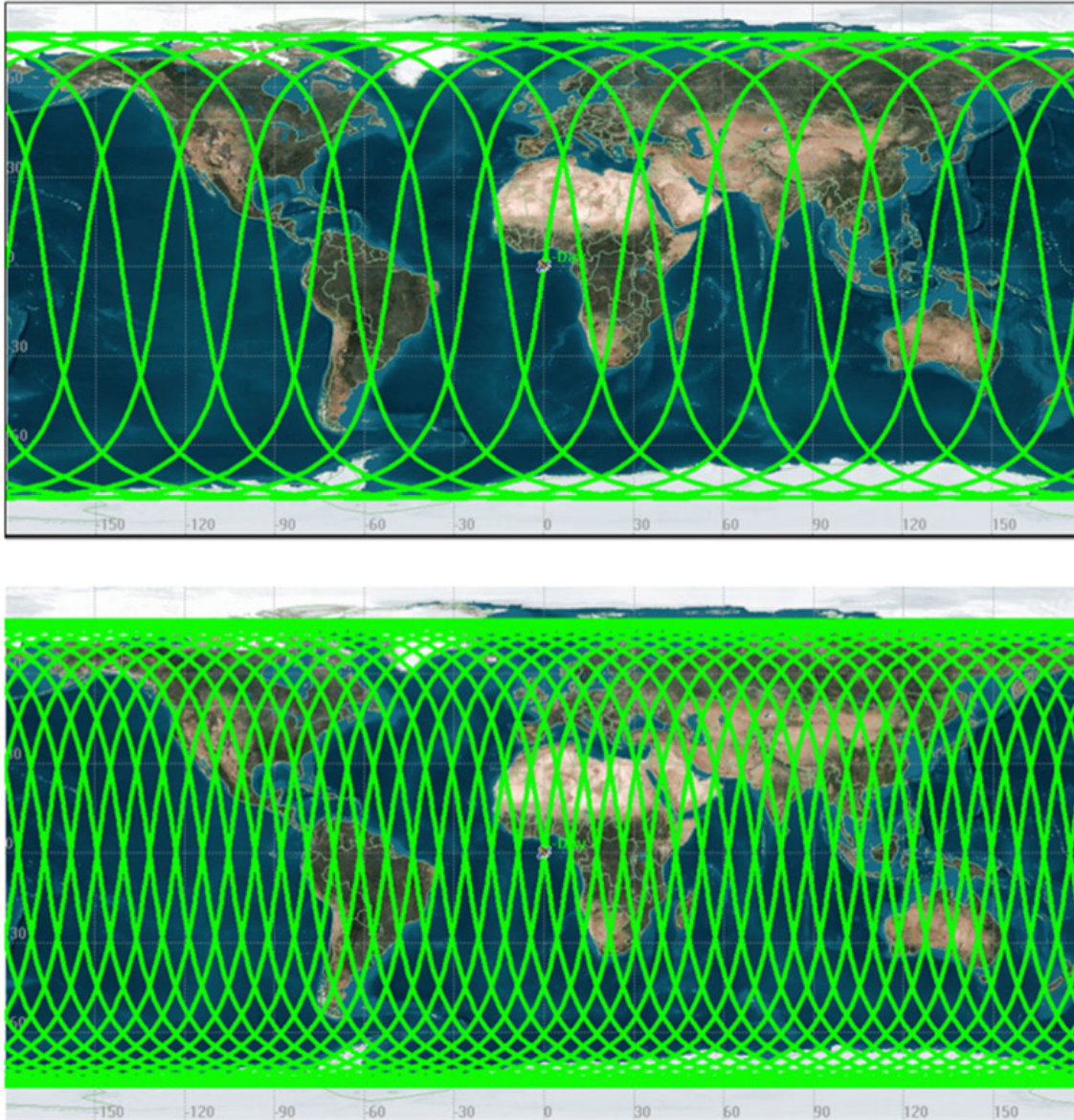
Figure 7.5-1. Ground track configuration for a 1-day (upper panel) or a 3-day (lower panel) repeat orbit assumed for the SWOT fast sampling phase. (Courtesy of S. Nerem, Colorado State University)
