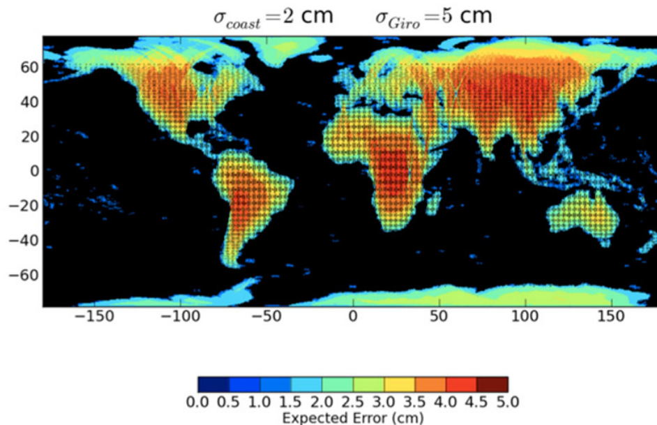
Figure 7.5-4. Expected residual phase/roll errors over land assuming that the ocean cross-over calibration can provide calibration accuracy of 2 cm (1 \sigma ). The results are based on optimal interpolation of the coastal estimates, assuming a known gyro correlation function and a gyro roll uncertainty equivalent to 5 cm (1 \sigma ) of roll error.
