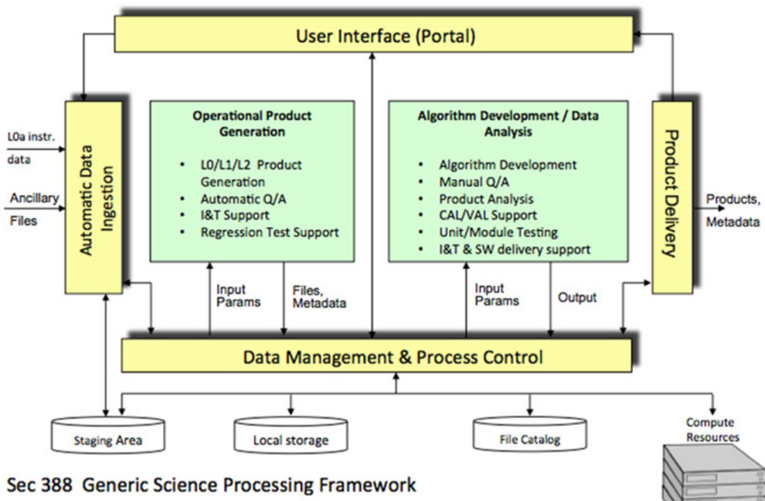
Figure 7.4-3. SDS Block Architecture: A view of SDS showing separate processors for different data types.
