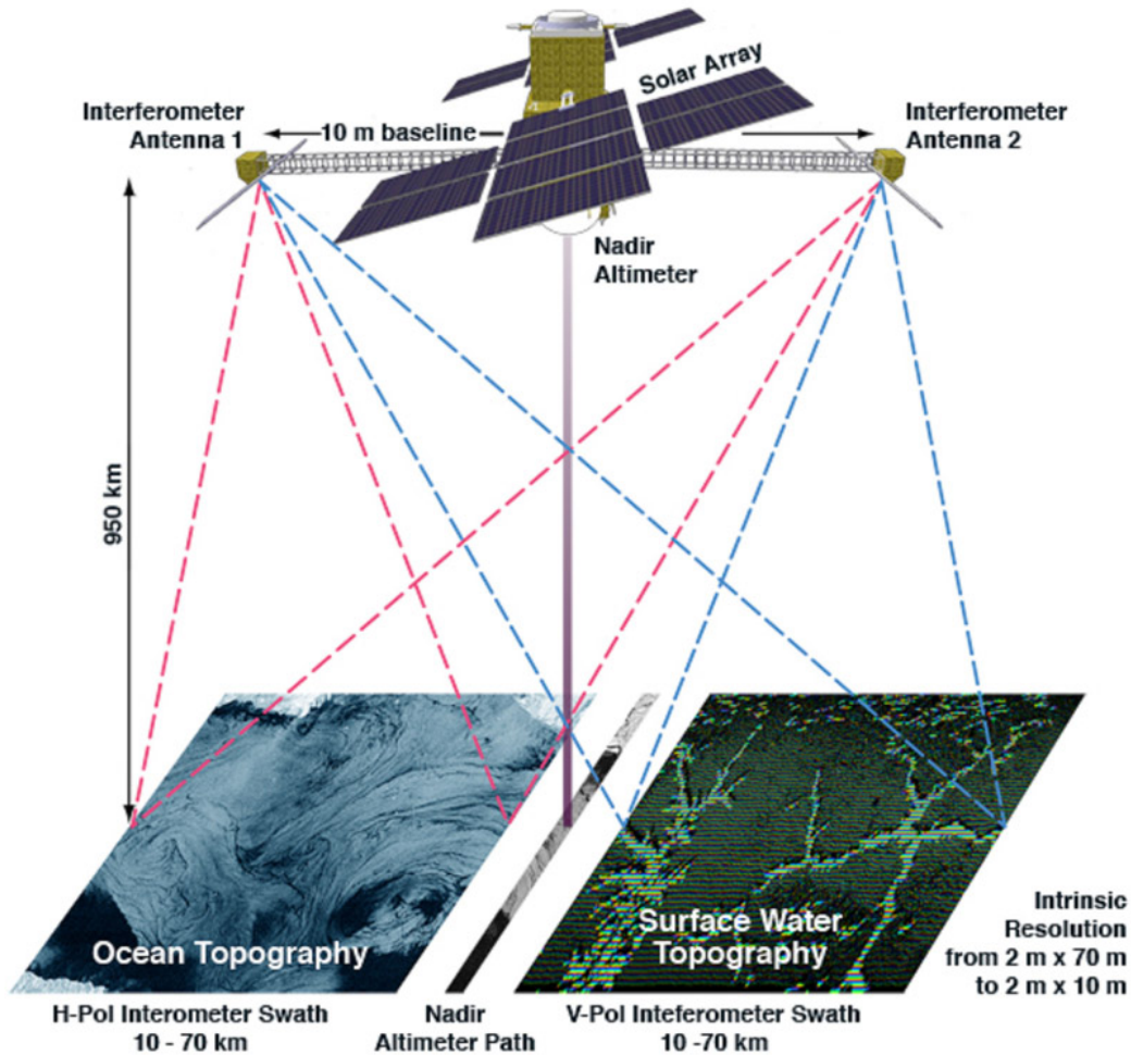
Figure 6.1-2. SWOT mission concept configuration.
