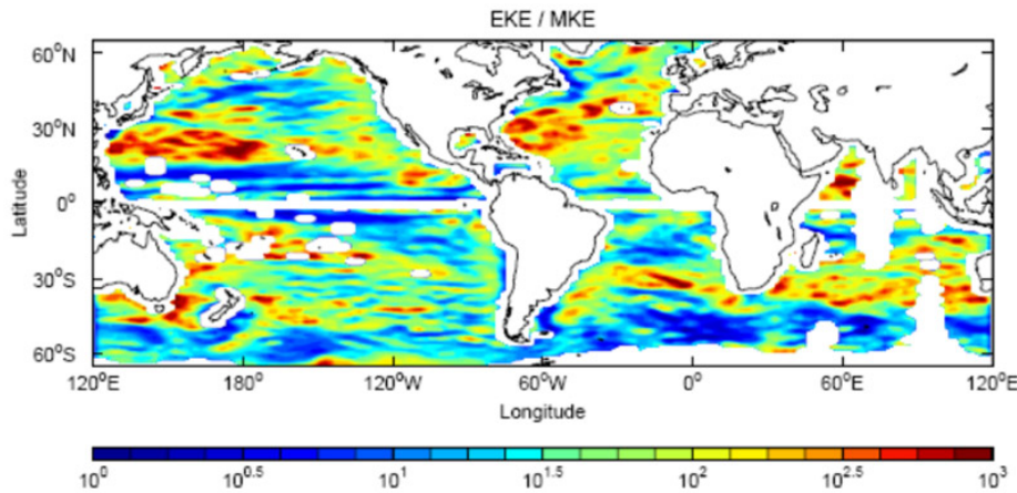
Figure 3-2. Ratio of eddy kinetic energy to the kinetic energy of the mean flow using surface velocities computed from the TOPEX/Poseidon and Jason interleaved mission (Sharffenberg and Stammer, 2009)
