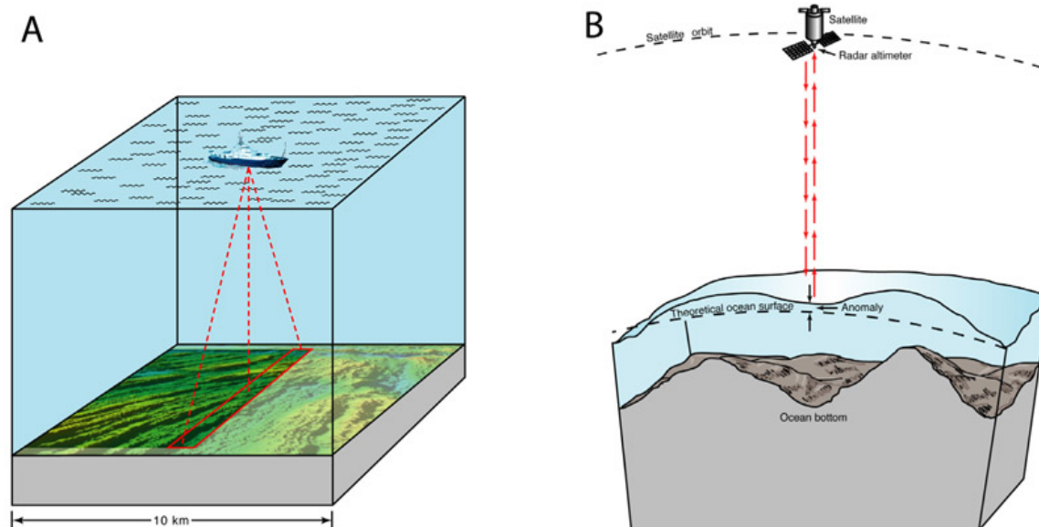
Figure 5.2-2. Modern tools for mapping the deep ocean floor. (A) A shipboard multibeam echo sounders uses sound waves to map 10–20 km wide swaths at \sim 200 horizontal resolution. (B) An Earth-orbiting radar cannot see the ocean bottom, but it can measure ocean surface height variations induced by ocean floor topography. While the resolution of the echo sounder technique is far superior to the ultimate resolution of the satellite altimeter technique ( \sim 8 km), complete mapping of the deep oceans using ships would take 200 ship-years at a cost of billions of dollars (Carron et al., 2001). Indeed, the shipboard and altimeter methods are highly complementary. The current distribution of ship soundings provides the long-wavelength (160 km) information that cannot be obtained from gravity because of spatial variations in isostasy (Figure 5.2-3). Satellite altimeters provide the global uniform coverage in the 16–160 km wavelength band. When interesting features are discovered in satellite gravity, they can be surveyed in fine detail by ships.
