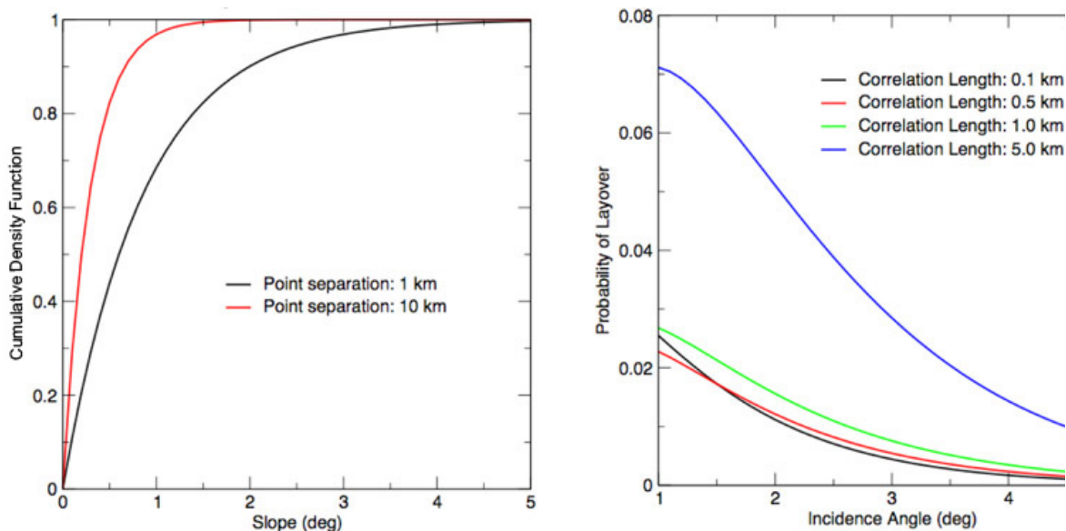
Figure 6.5-2. (Left panel) cumulative density function for slopes for points separated by 1 km (black line) or 10 km (red line) derived from global GTOPO30 topography, as derived by Kreslavsky and Head (1999). (Right panel) Probability of topographic layover, as a function of incidence angle and surface topography correlation length.
