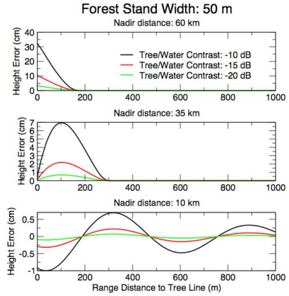
Figure 6.5-7. Height errors as a function of cross-track distance [from near swath (bottom) to far swath (top)], tree/water brightness contrast, and distance between the water pixel and the start of the vegetation patch along the range direction. The tree stand has a range extent of 50 m and was assumed to be 50 m tall.
