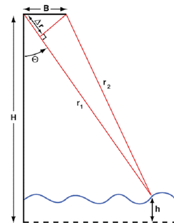
Figure 6.1-1. Geometric concept used for interferometric measurements.
