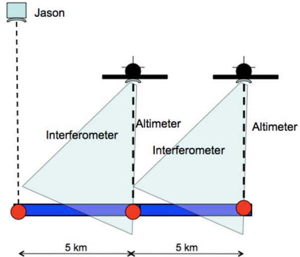
Figure 7.5-2. Conceptual scheme for AirSWOT altimeter calibration and juxtaposition of swaths. A Jason-class altimeter would provide a ground track with high-accuracy elevations and high consistency over scales of 100 km. The first AirSWOT 5 km swath residual roll errors would be corrected with this ground track; and a new, cross-calibrated nadir altimeter track would be measured with the AirSWOT nadir altimeter. The process would be iterated to achieve a wider effective swath.
