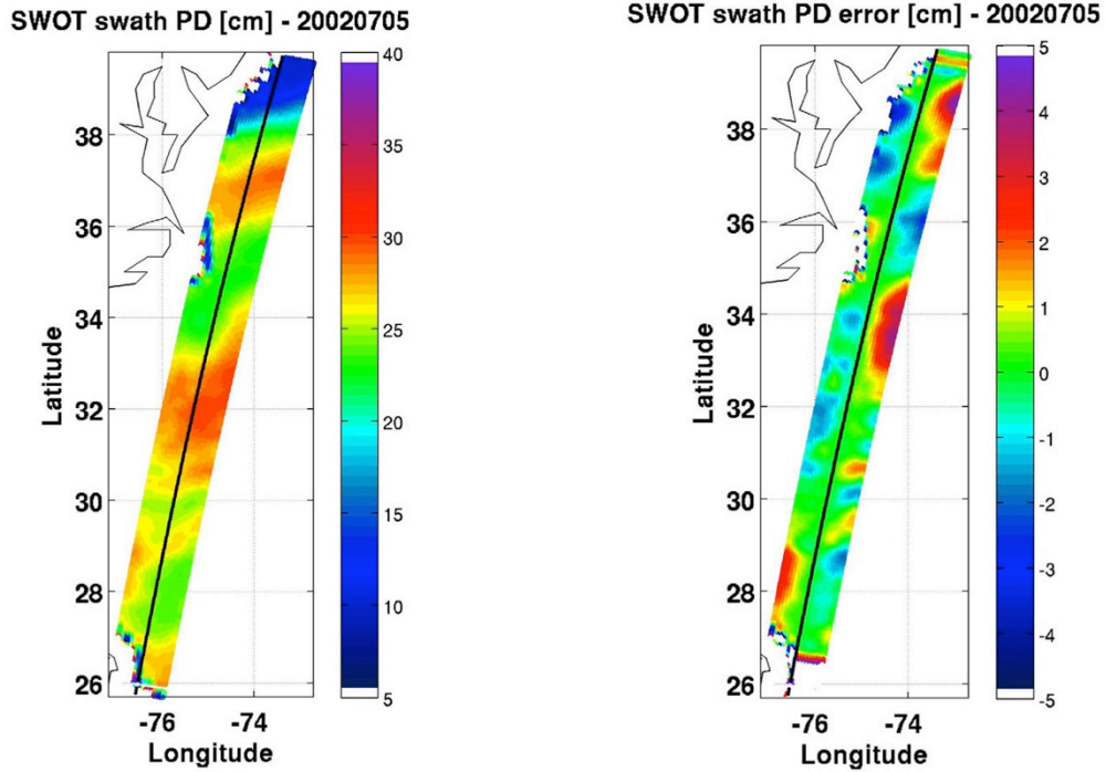
Figure 6.2-4. (Left) Path delay across the projected SWOT swath derived from AMSR-E fields. (Right) Residual path delay error structures across the SWOT swath from a nadir-only correction.
