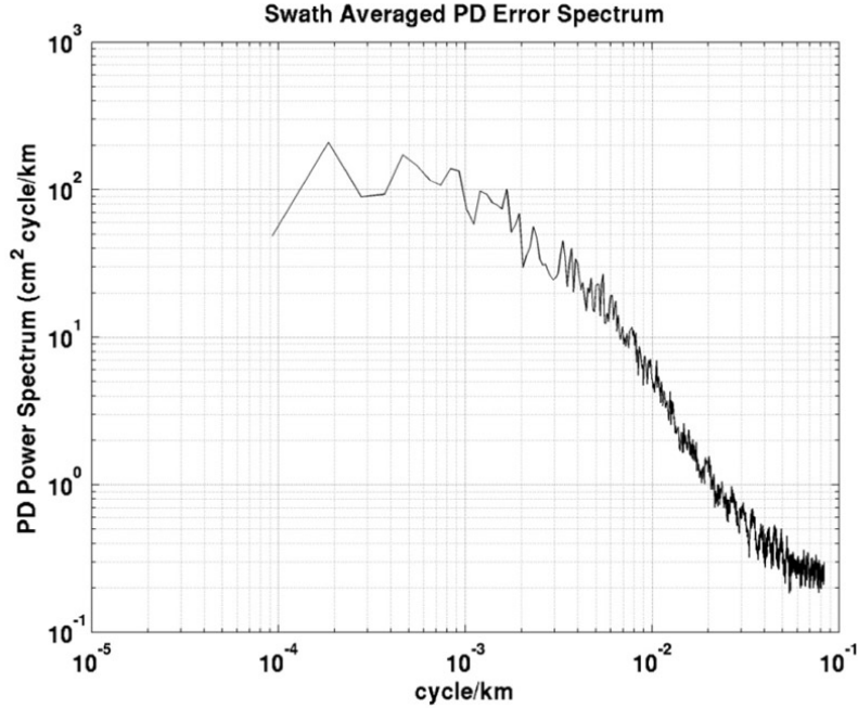
Figure 6.2-5. Residual path delay error spectrum averaged across the anticipated SWOT swath for a nadir-only path delay correction.
