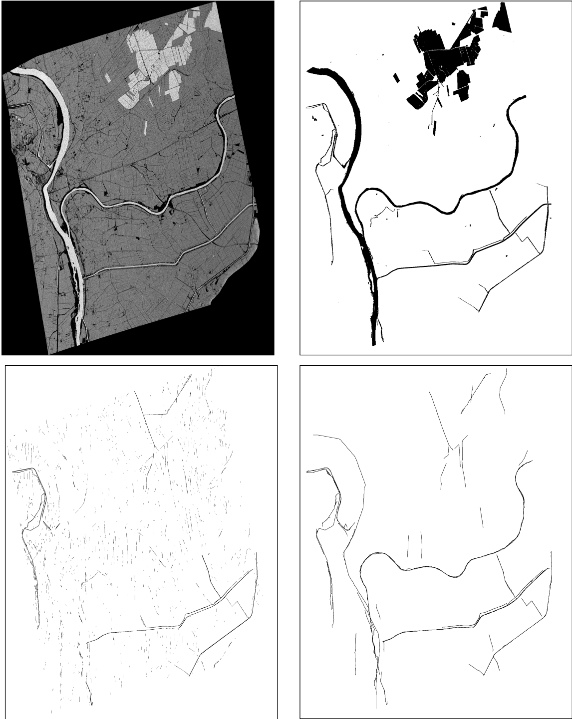
Figure 6.6-2. Example of result of detection of narrow water surfaces (Cao et al., 2011). Simulated KaRIn/SWOT amplitude image (upper panel, left), reference water mask (upper panel, right), result of low-level water detection step (lower panel, left), and result of high-level water detection step (lower panel, right).
