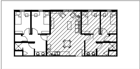
KEY PLAN: SEE 6.6 FOR RESIDENT LIVING SUITE
