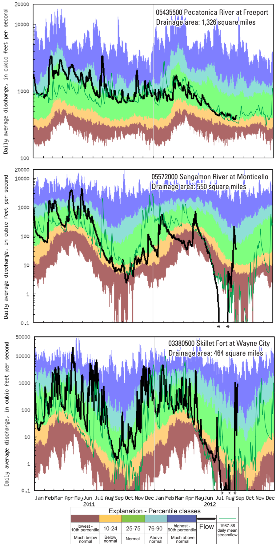
Figure 3. Duration hydrographs of daily average streamflow for 3 index stations in Illinois shown in Figure 1. Asterisk (*) indicates flow less than 0.1 cubic feet per second (cfs). Significant precipitation in August and early September 2012 resulted in increases in streamflow in Monticello and Wayne City.
