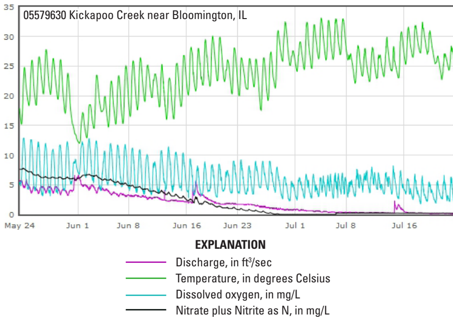
Figure 7. Real-time data recorded by sensors at a Kickapoo Creek site near Bloomington in cooperation with the Illinois Environmental Protection Agency. These data show that flow is decreasing, water temperature is increasing, and dissolved oxygen and nitrate concentrations are also declining.
