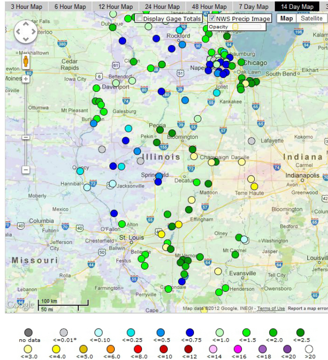
Figure 4. Precipitation gage data collected in the 14 days before August 21, 2012, in Illinois.
