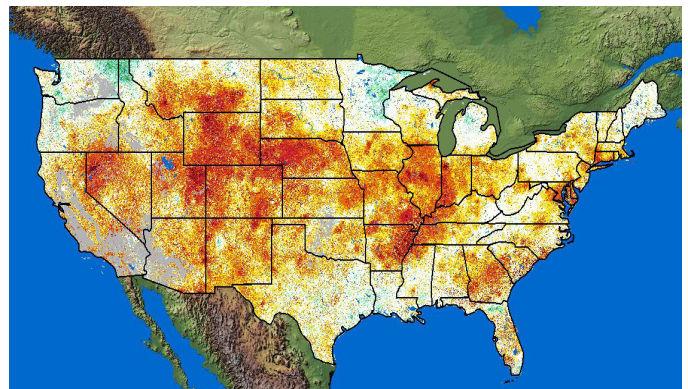
Figure 11. eMODIS VegDRI image for August 19, 2012, for the United States.
