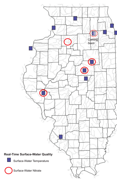
Figure 8. Real-time continuous nitrate and temperature sensors operated by the USGS in Illinois.
