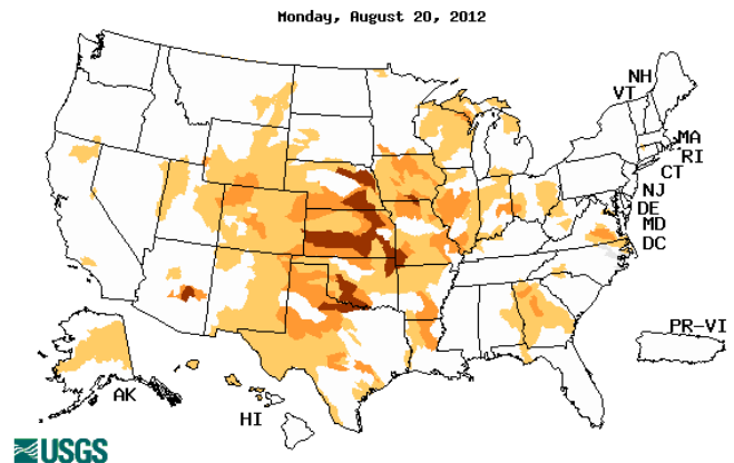
Figure 10. Below normal 7-day average streamflow compared to historical streamflow for August 20, 2012, for the United States.
