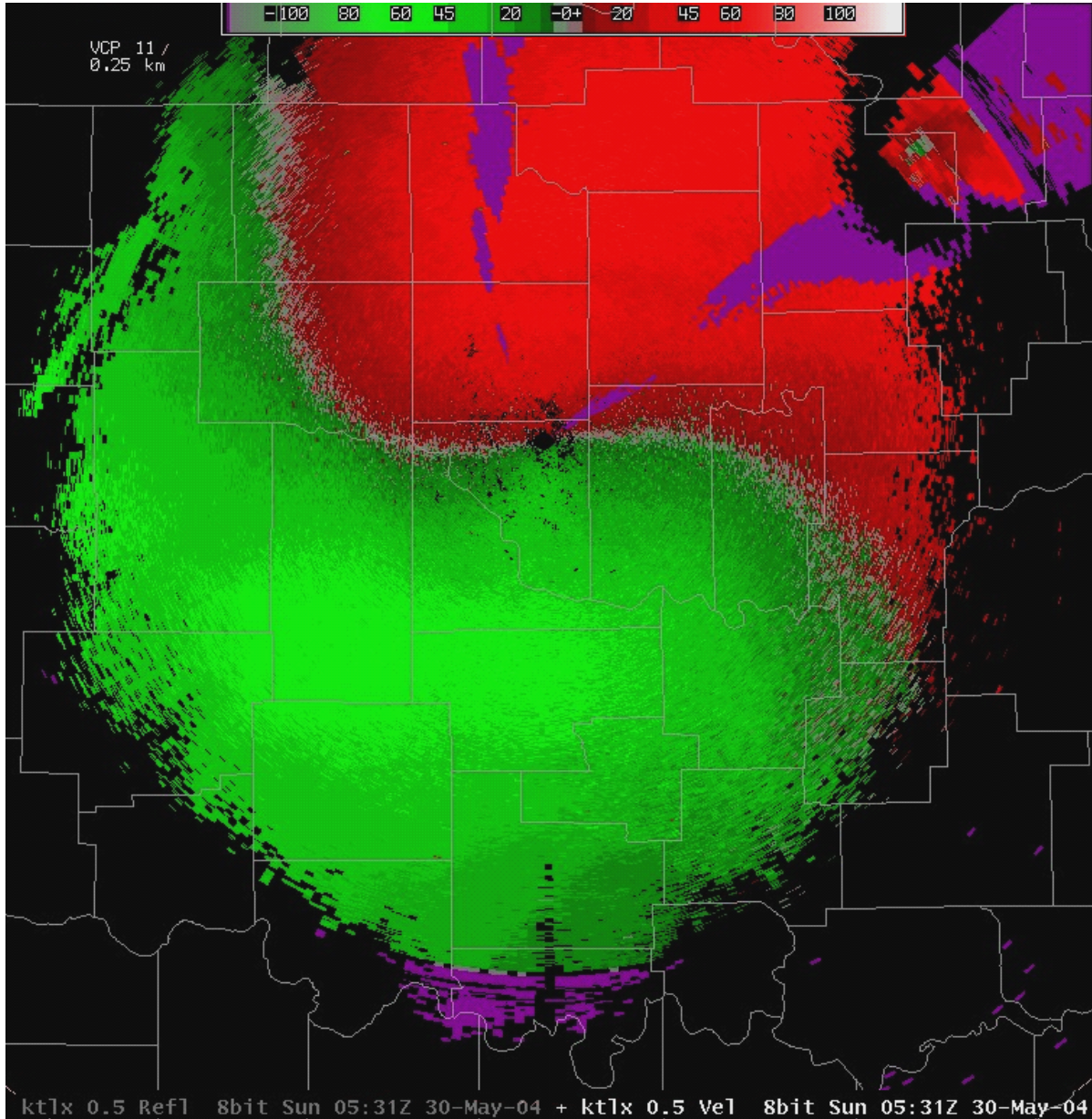
Figure 4-57 Base Velocity Data Array Product of a Low-Level Jet
