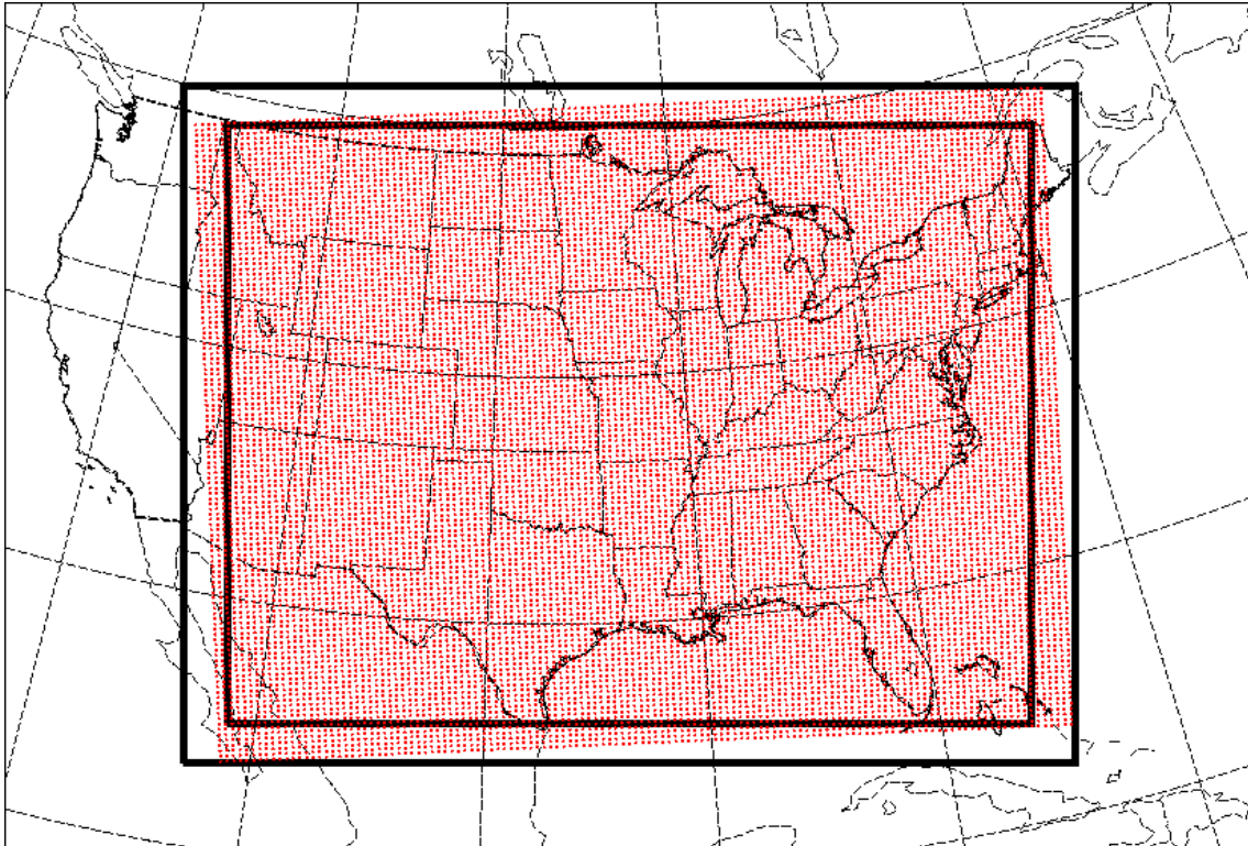
Figure 2. CAPS 00 UTC domains for the 2009 Season. The outer thick rectangular box represents the domain for performing 3DVAR ( Grid 1 – 1000 \times 760 ). The red dot area represents the WRF-NMM domain ( Grid 2 – 979 \times 650 ). The inner thick box is the domain for WRF-ARW and also for common verification ( Grid3 - 900 \times 672 ).
