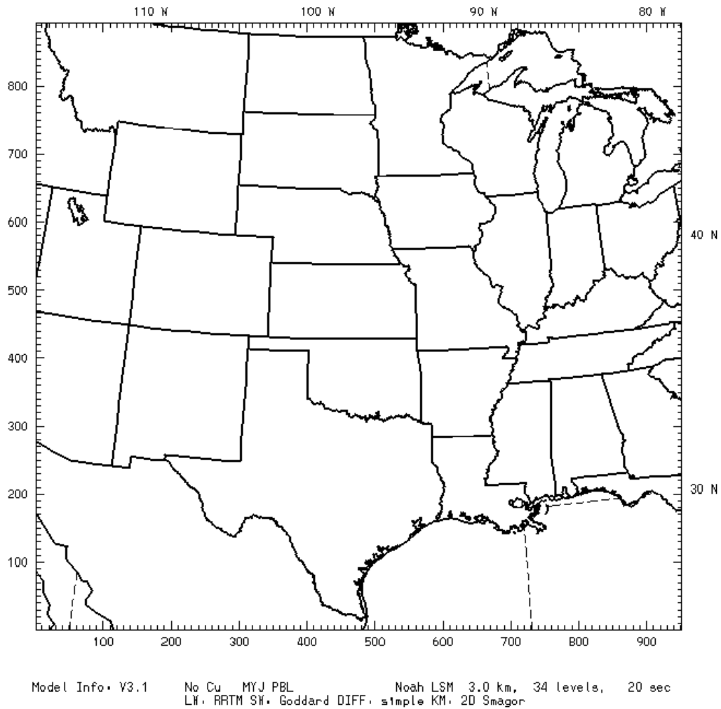
Fig. 6. NCAR 3 km WRF-ARW domain.
