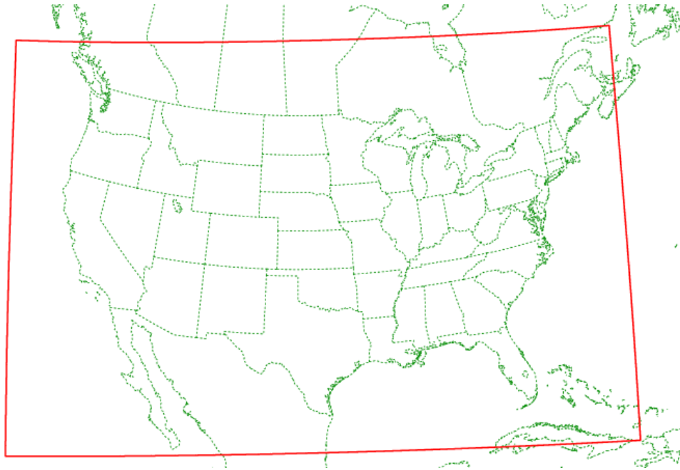
Figure 3. EMC 4 km WRF-NMM domain with 1239x920 horizontal grid points.
