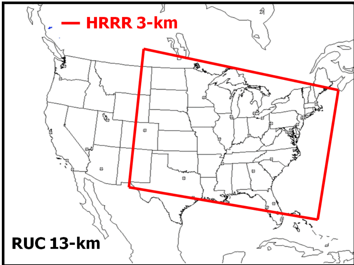
Figure 5. RUC 13 km domain (black) and HRRR 3 km domain (red) with 1000x700 horizontal grid points.
