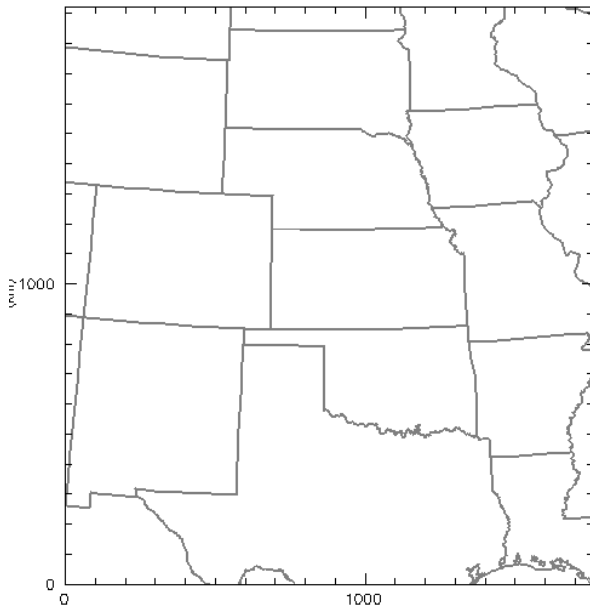
Figure 2. CAPS 12 UTC 4 km WRF-ARW update model domain with 444 \times 480 horizontal grid points.
