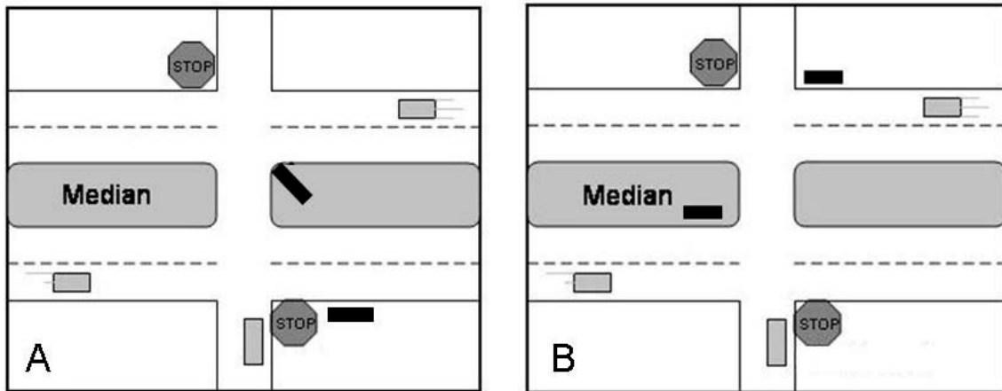
Figure 33. Location of Icon sign at intersection. A) The near-side sign is placed to the driver's right when at the stop sign while the median sign is placed on the driver's right in the median. B) The signs are placed to the left and right of the driver, but across the lanes.
