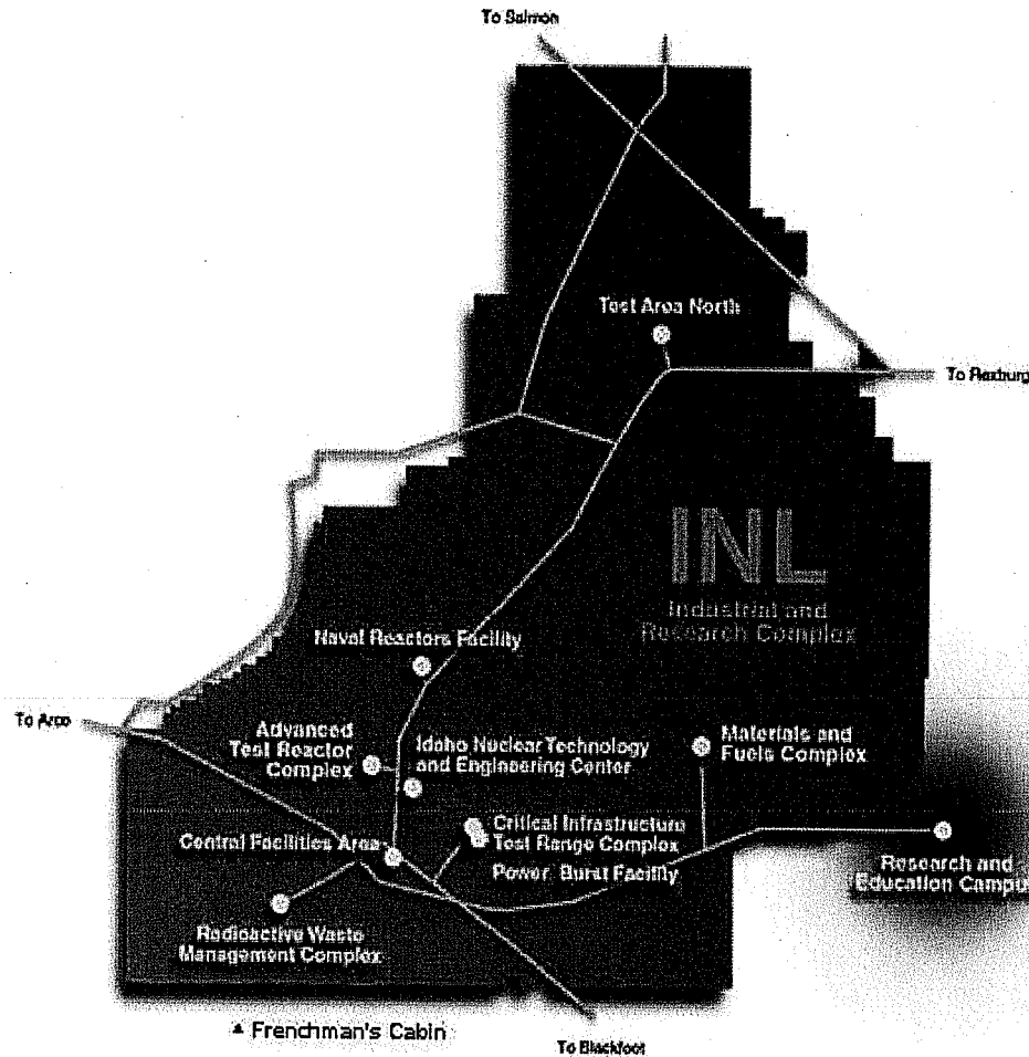
Figure 1. INL Site, including major facility areas and off-site MEI located at Frenchman's Cabin.
