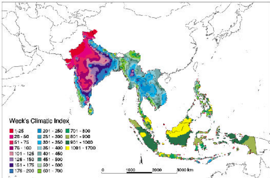
Fig. 6. Weck's Climatic Index for the study area, displayed
