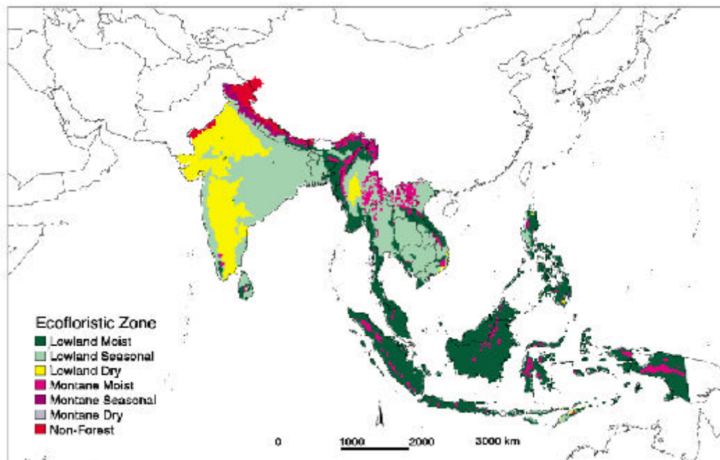
Fig. 10. Ecofloristic zone classification for the study area, displayed with 0.25-degree resolution.
