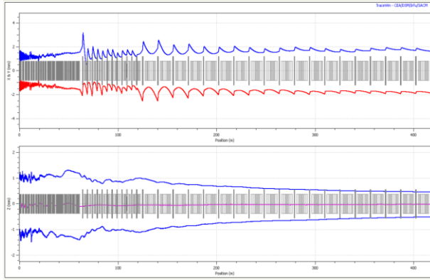
Fig. 2: Beam envelope in the transverse plane (top plot: X blue, Y red) and in longitudinal plane (bottom plot) is shown for SC linac.
