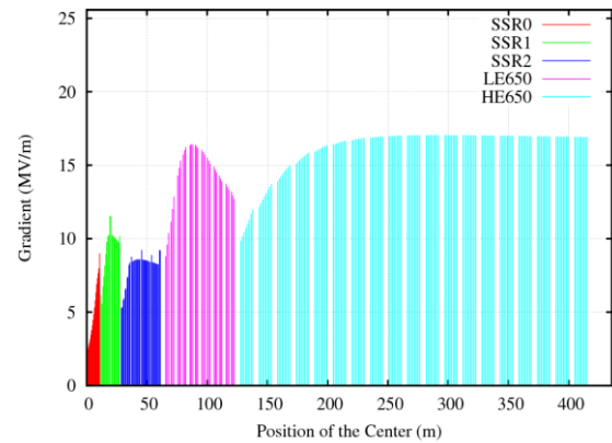
Fig. 5: Cavity gradient along the linac.
