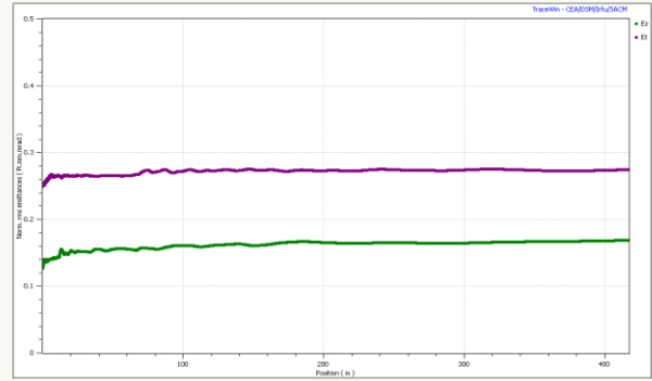
Fig. 4: Emittance dilution in Transverse (magenta) and longitudinal (green) plane along the linac.
