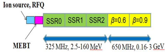
Fig. 1: Acceleration scheme
