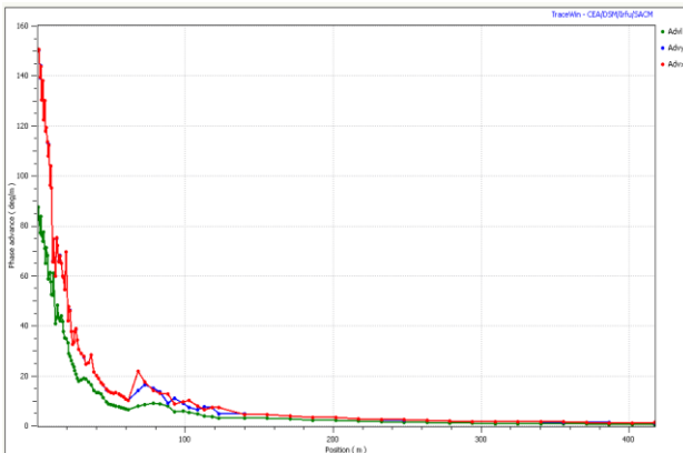
Fig. 3: Transverse (red & blue) and longitudinal (green) wave numbers along the SC linac.
