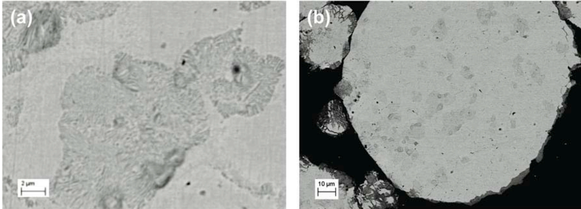
Fig. 3. Backscattered electron images for the U-7Mo/Al-2Si sample showing (a) decomposition in the U-7Mo alloy and (b) the morphologies of the interaction layers around different fuel particles.
