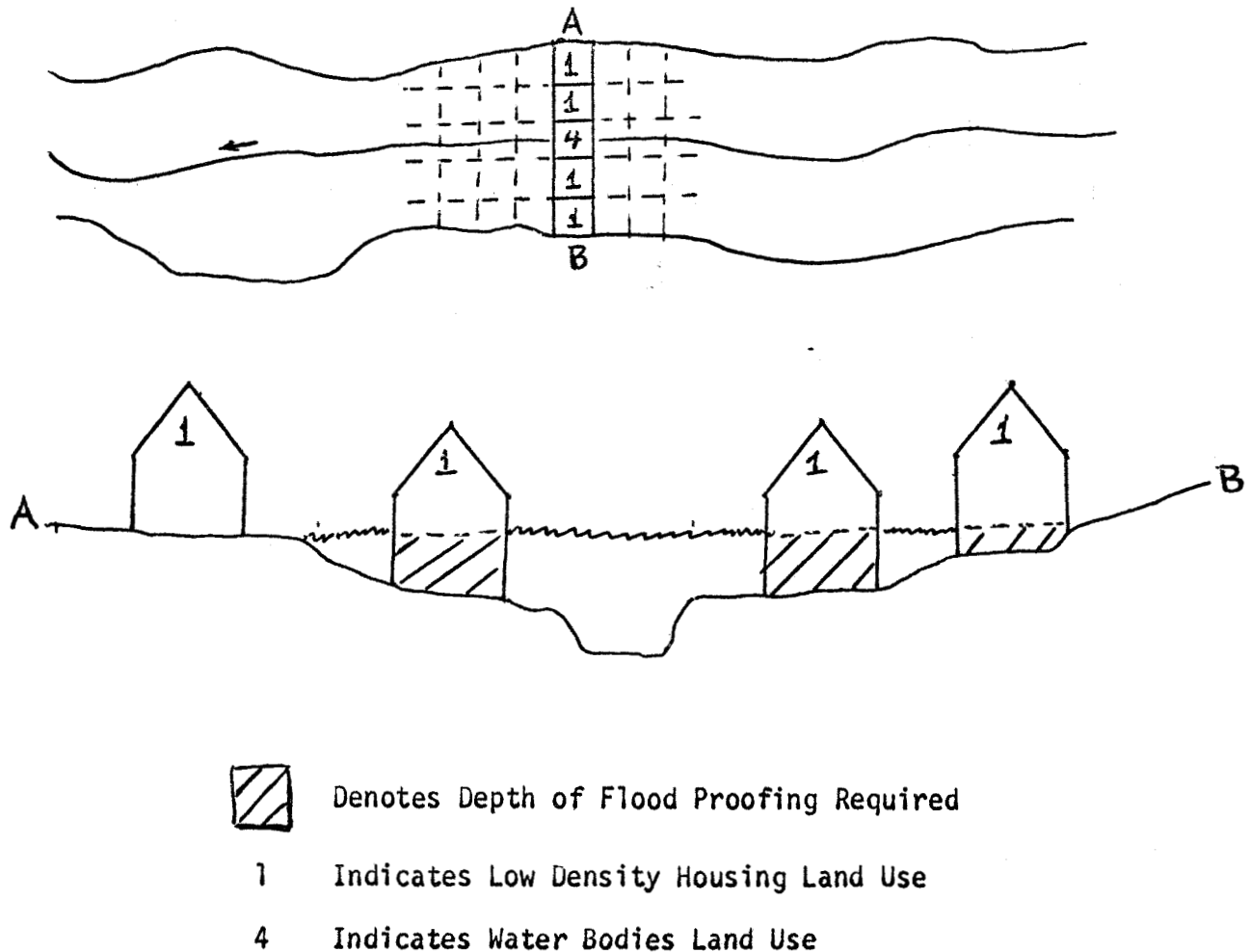
Fig. 5--Example Cross Section (From A to B)
