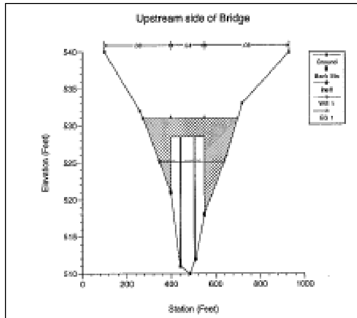
Figure 2 Cross Section Bridge Plot
