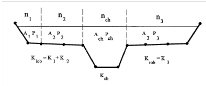
Figure 4 HEC-RAS Conveyance Subdivision
