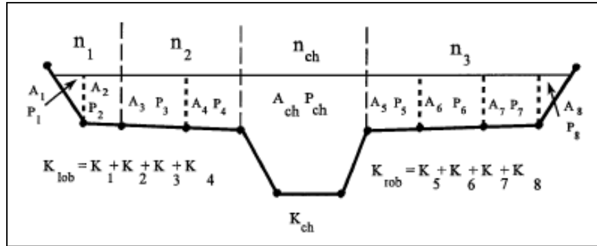
Figure 3 HEC-2 Conveyance Subdivision
