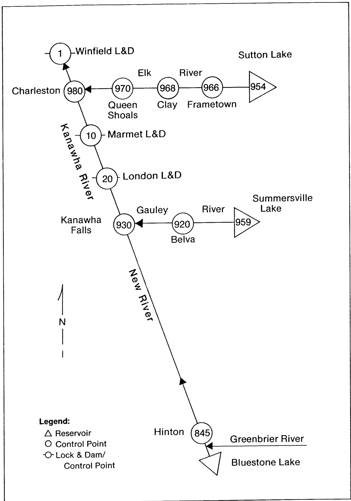
Figure 7 KANAWHA RIVER BASIN SCHEMATIC
