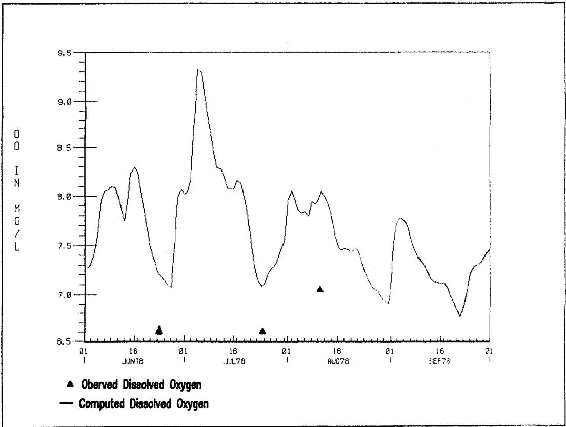
Figure 12 MONONGAHELA RIVER ABOVE PITTSBURGH - DISSOLVED OXYGEN
