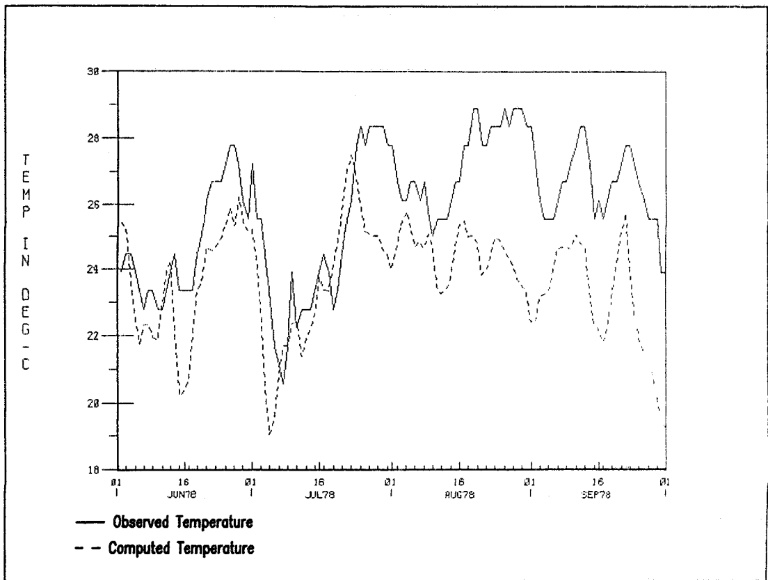
Figure 11 MONONGAHELA RIVER ABOVE PITTSBURGH - WATER TEMPERATURE
