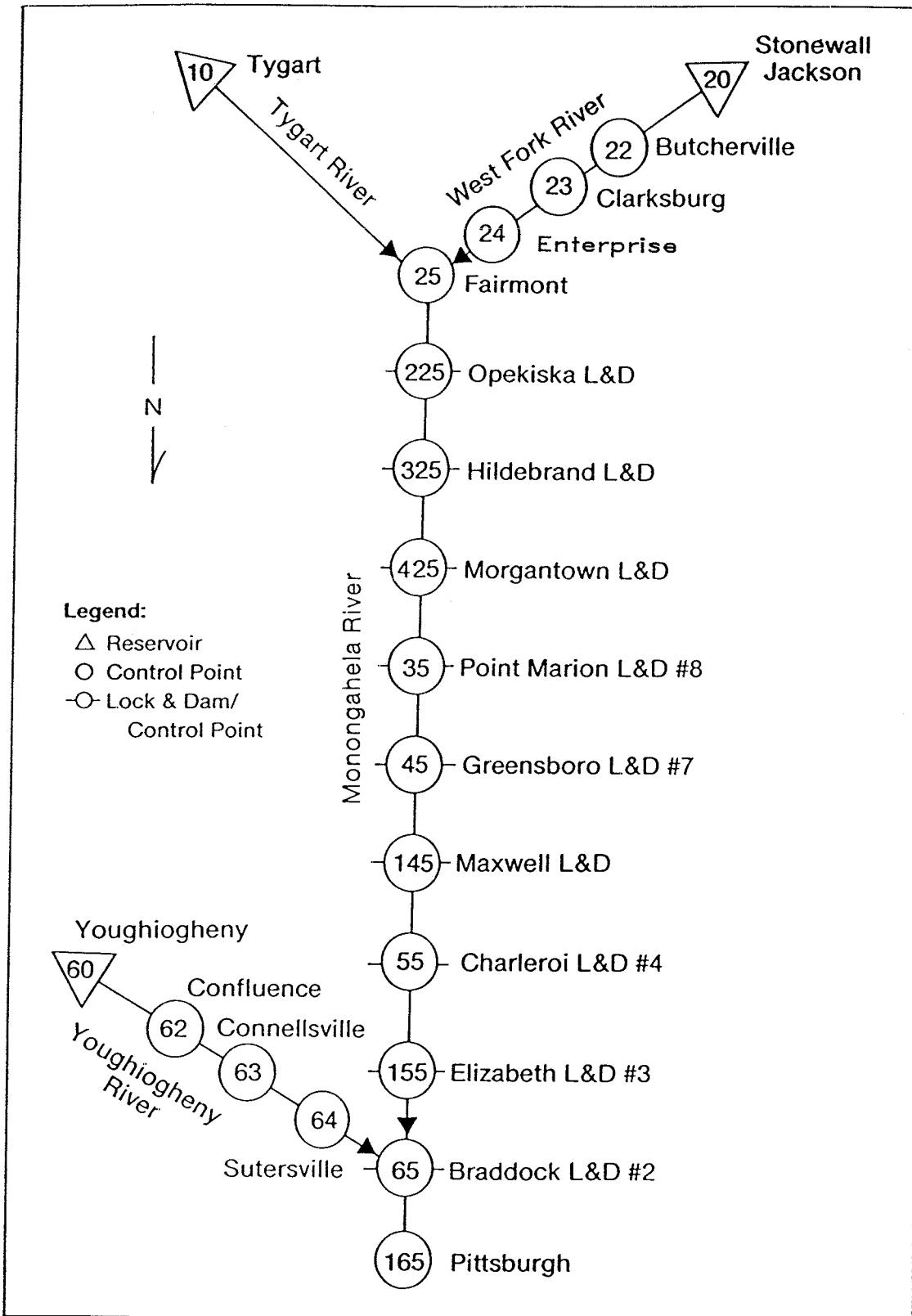
Figure 10 MONONGAHELA RIVER BASIN SCHEMATIC
