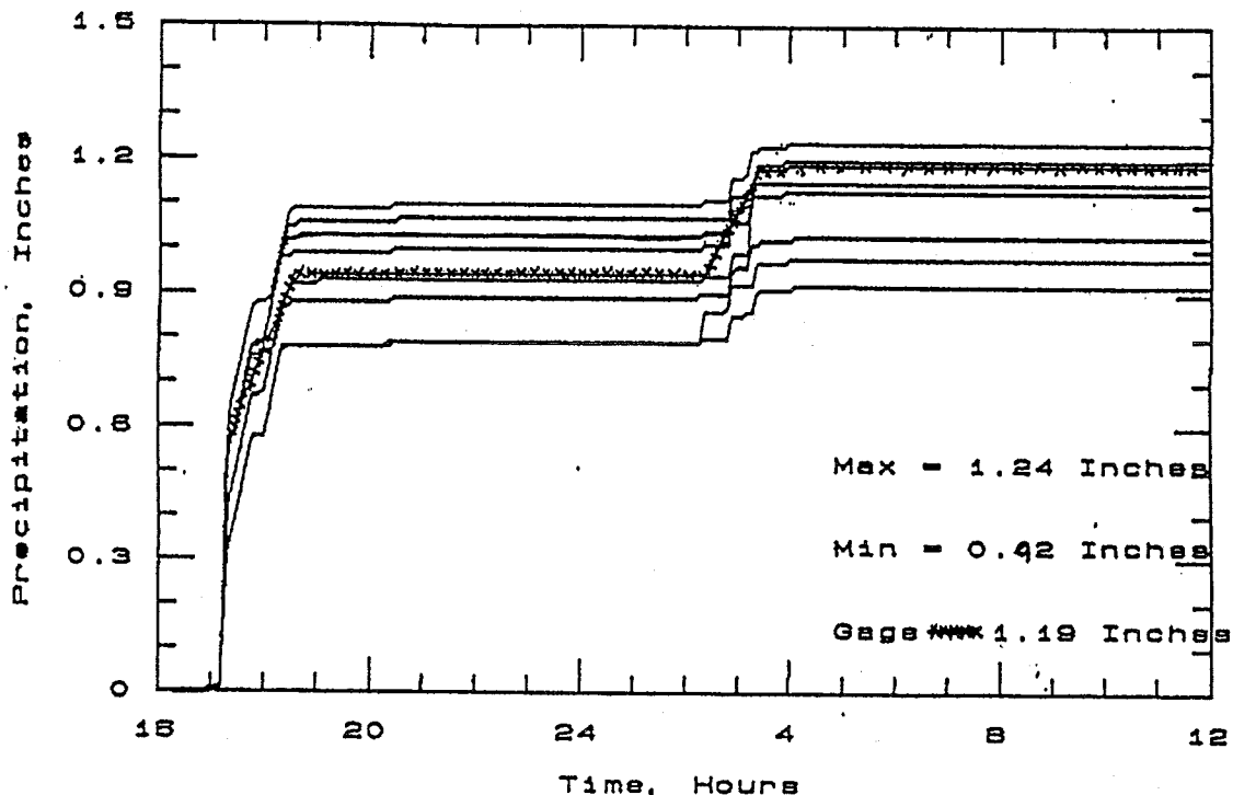
Fredericktown Radar Precipitation vs. RAIN GAGE April 14, 1987
