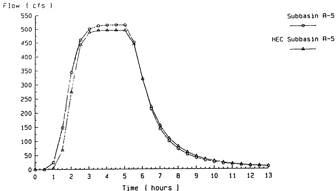
Figure 5. Subbasin R-5 (non-urbanized) runoff comparison.
