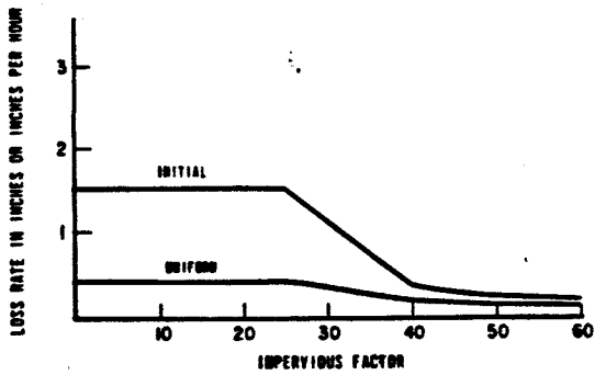
Figure 5 - LOSS RATE FUNCTION, 10-YEAR EVENT
