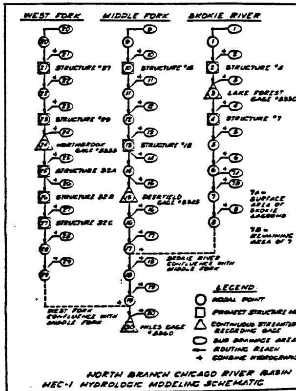
Figure 2 - Basin Schematic
