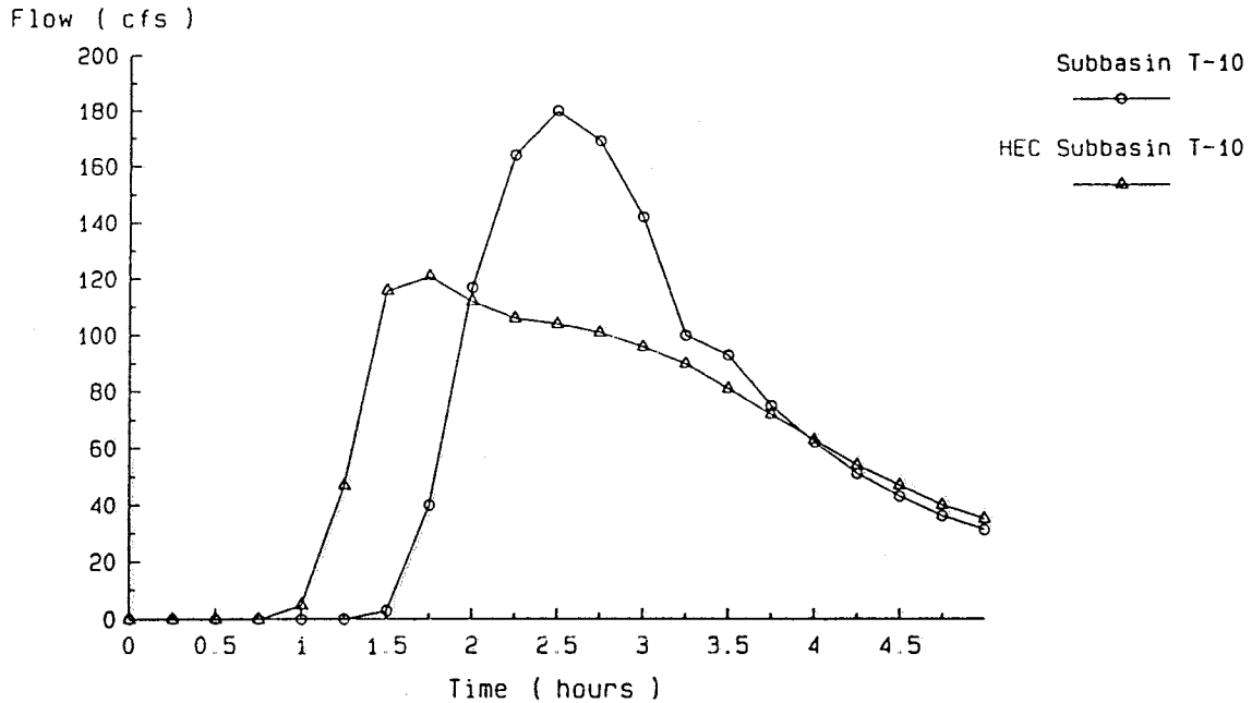
Figure 3. Subbasin T-10 (partially urbanized) runoff comparison.
