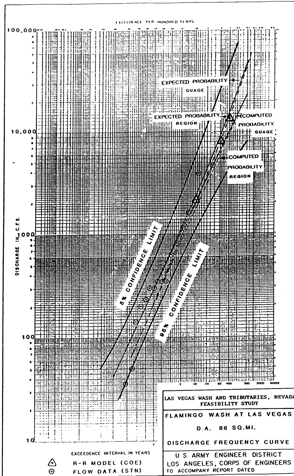
Figure 6. Comparison of kinematic wave model to gaged frequency curves.
