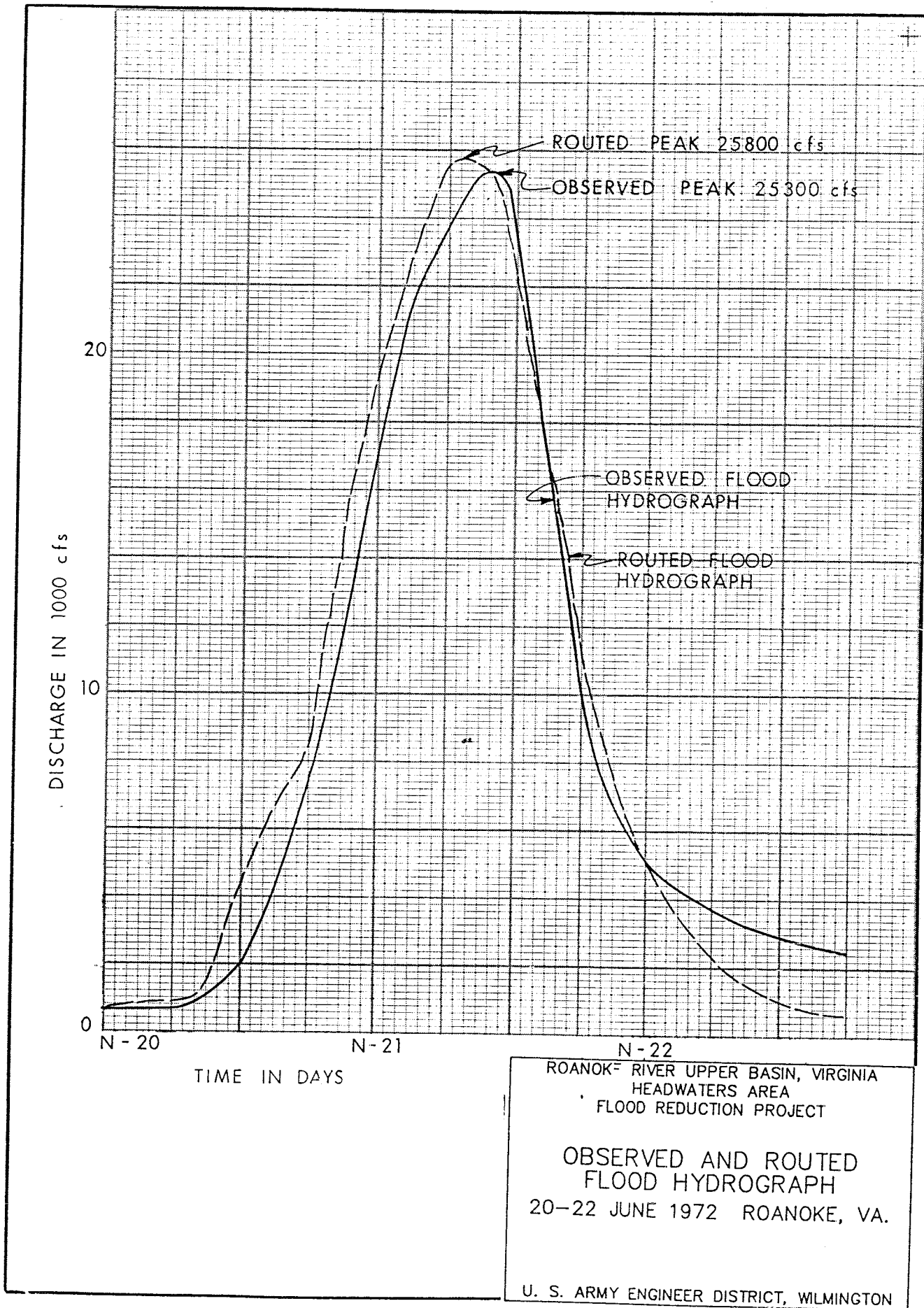
FIGURE 7. OBSERVED AND ROUTED FLOOD HYDROGRAPH
