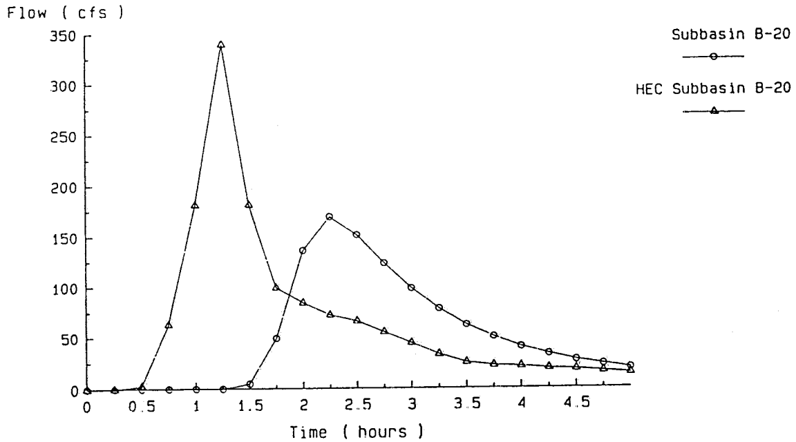
Figure 1. Subbasin B-20 (fully urbanized) runoff comparison.
