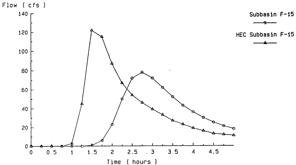
Figure 4. Subbasin F-15 (partially urbanized) runoff comparison.
