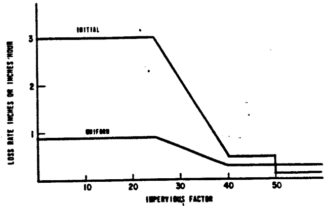
LOSS RATE FUNCTION, 100-YEAR EVENT
