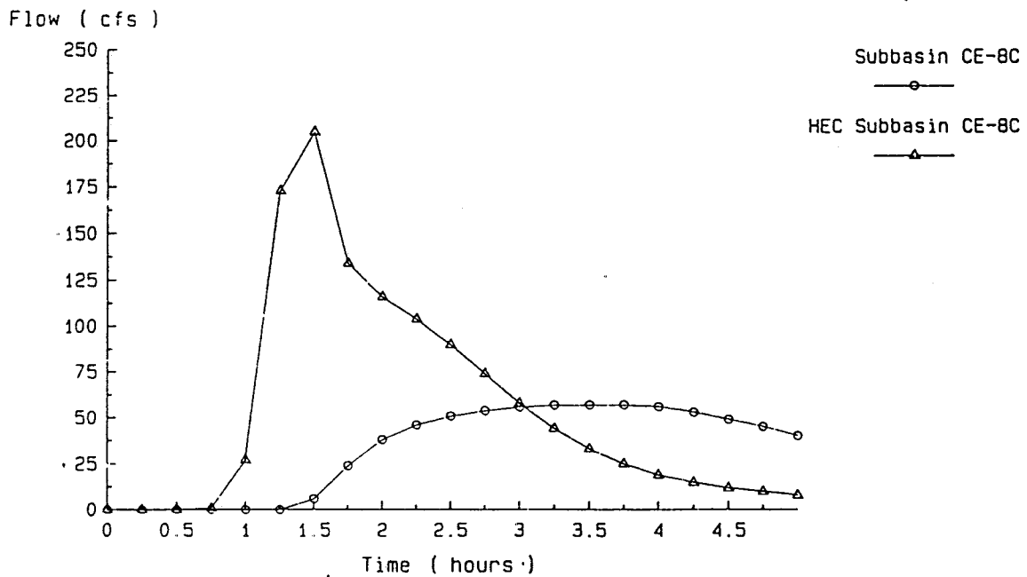
Figure 2. Subbasin CE-8C (fully urbanized) runoff comparison.
