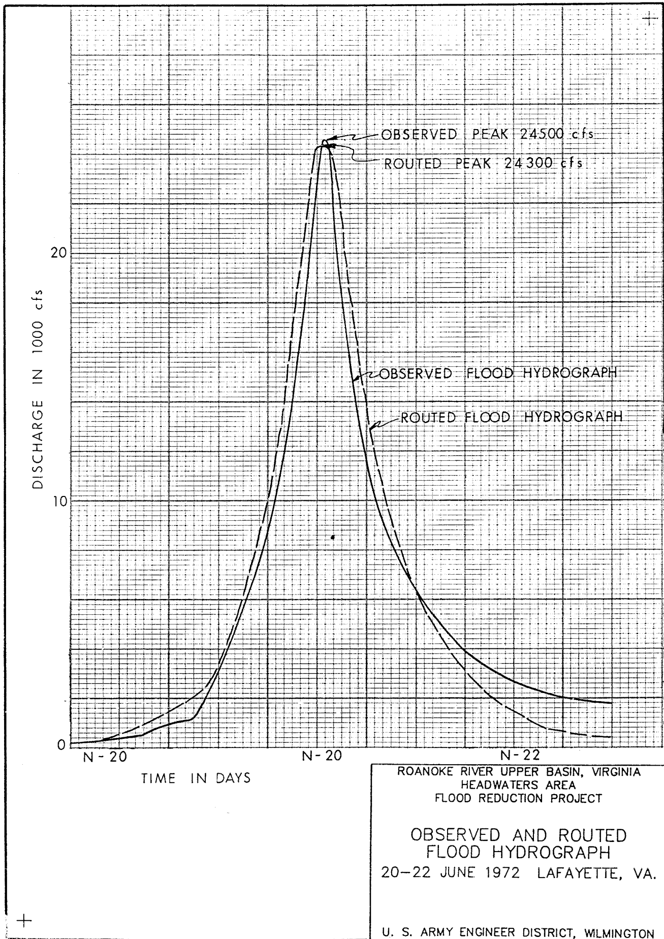
FIGURE 6. OBSERVED AND ROUTED FLOOD HYDROGRAPH
