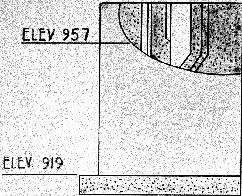
PROFILE INTAKE STRUCTURE BUFORD DAM
