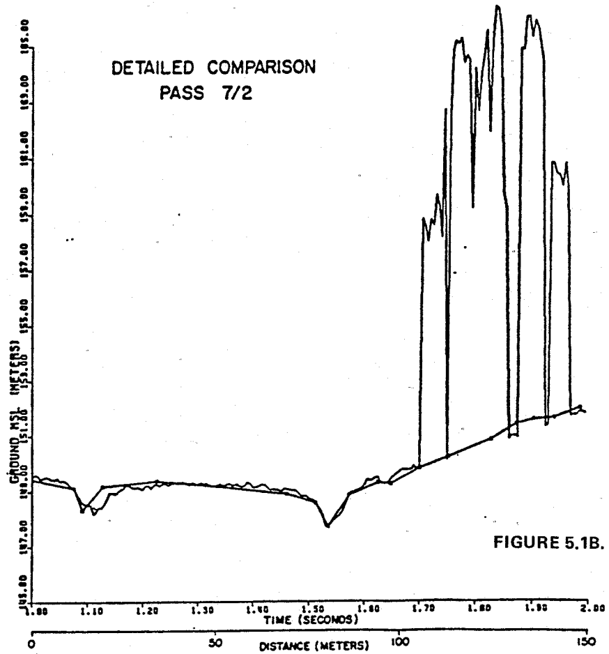
FIGURES 5.1A / 5.1B. Comparisons of laser reference profile for stream valley.
