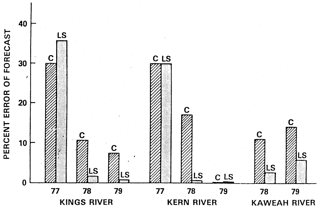
Figure 5.6: Seasonal snowmelt runoff forecast error using conventional (C) and Landsat snow cover (LS) procedures in the southern Sierra Nevada on May 1.
