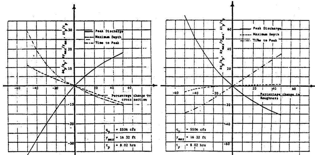
FIGURE 2.14B. Impact of Uniform Errors in the Cross Sections on Response.
