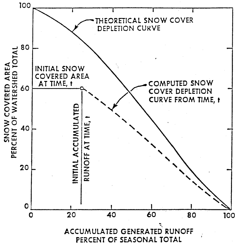
Figure 5.5. Snow Cover Depletion Curve
