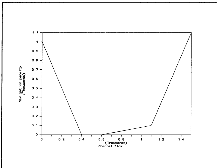
FIGURE C-10 Typical Navigation Penalty Function
