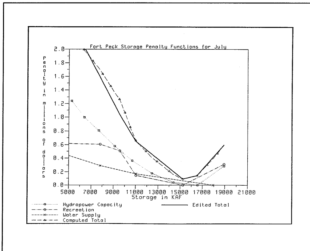
FIGURE C-16 Penalty Functions Combined
