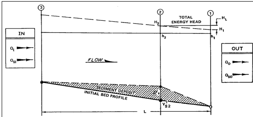
Definition Sketch for HEC-6 Modeling Computations
