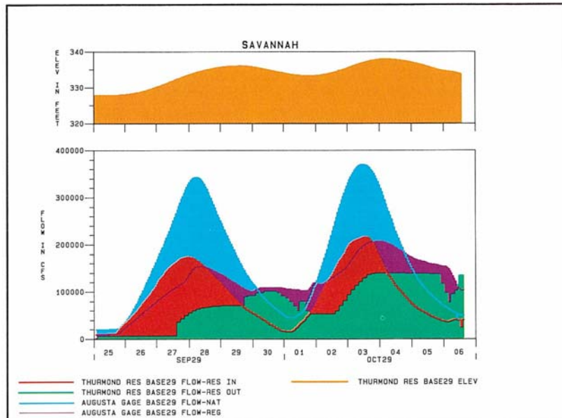
Computer Graphics of a Reservoir Operation
