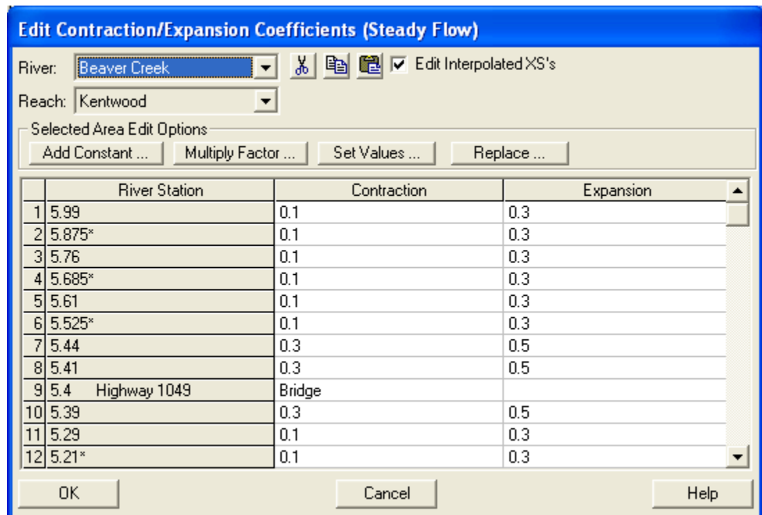
Figure 2-6: Coefficients For Beaver Creek
