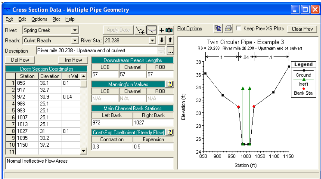
Figure 3-2: Cross Section Data Editor
