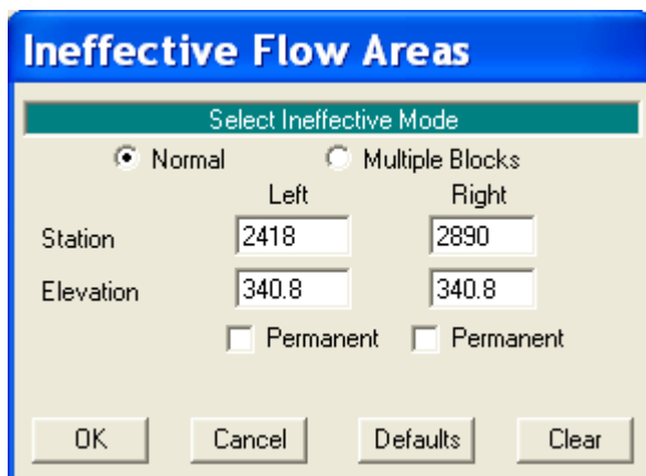
Figure 13-9: Normal Ineffective Flow Areas for Cross Section 52.38
