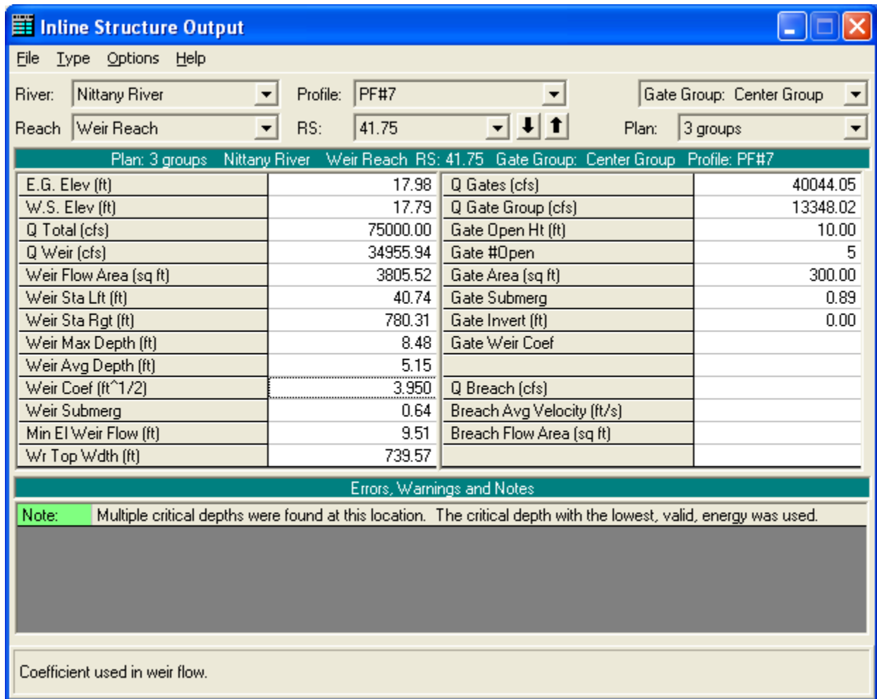
Figure 12-16: Inline Structure Output Table for Profile 7
