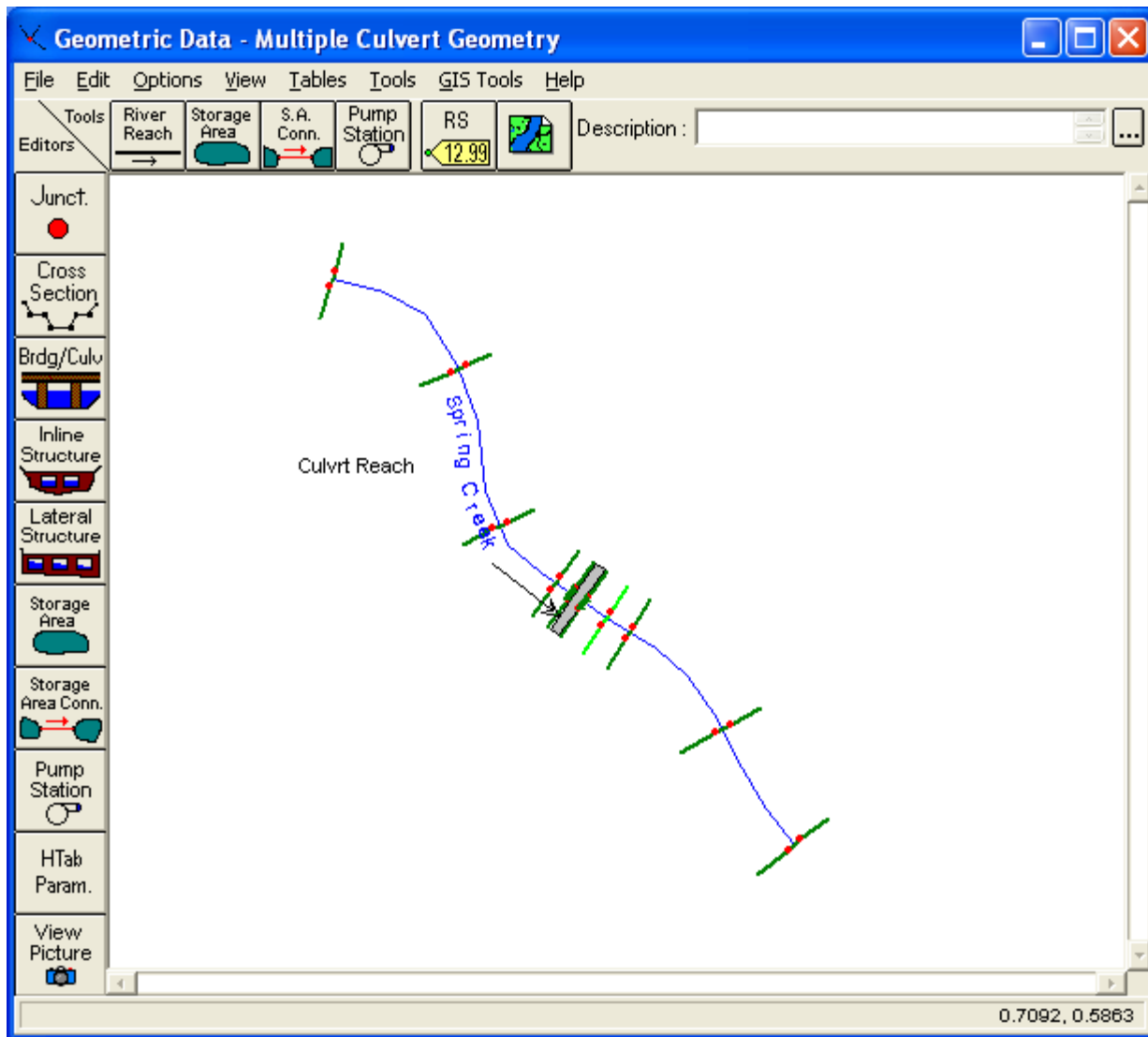
Figure 4-1: River System Schematic For Spring Creek
