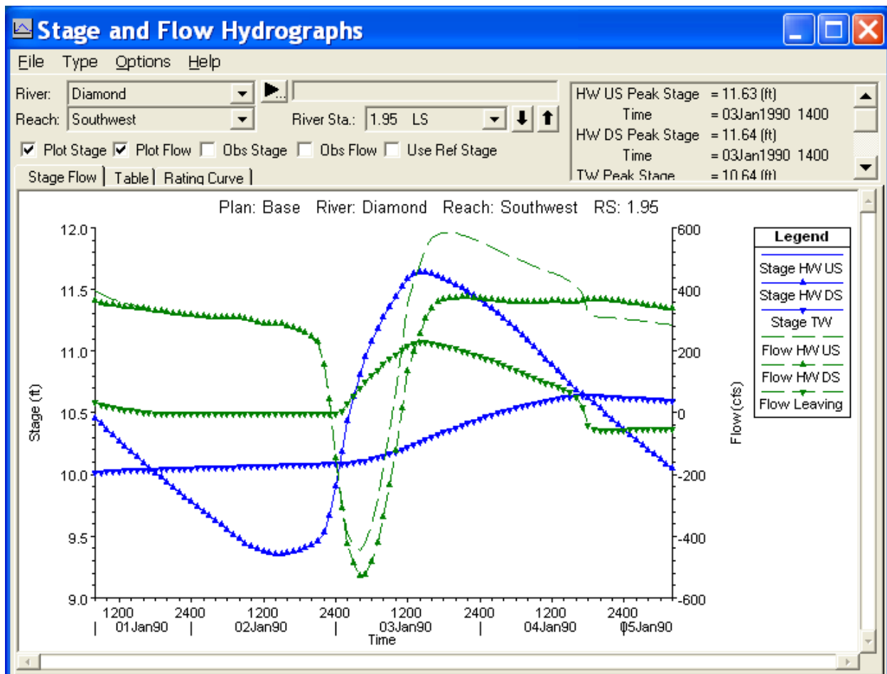
Figure 17-23: Stage and Flow Hydrograph for Lateral Structure Located on the Southwest Reach
