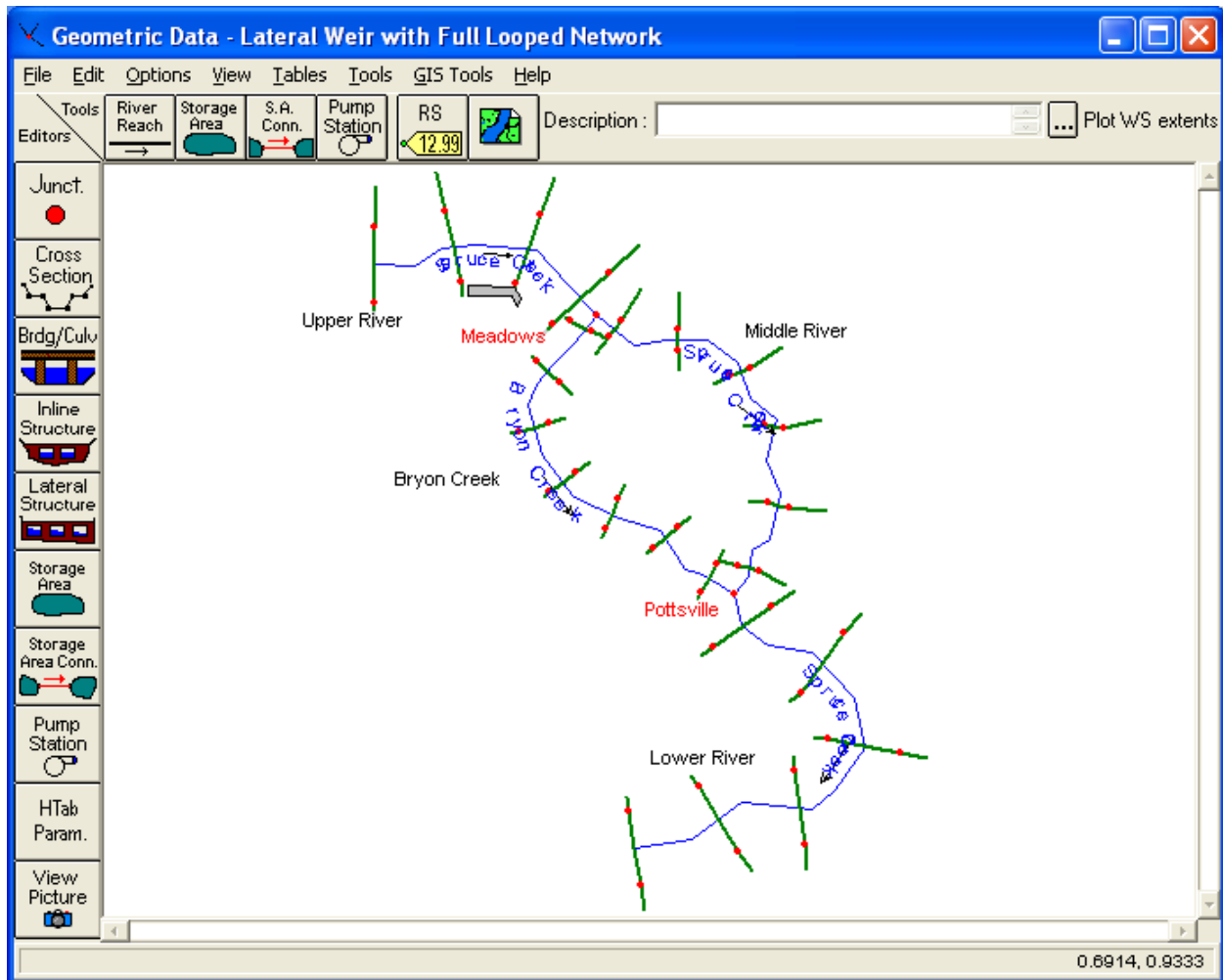
Figure 15-1: River System Schematic for Split Flow Example
