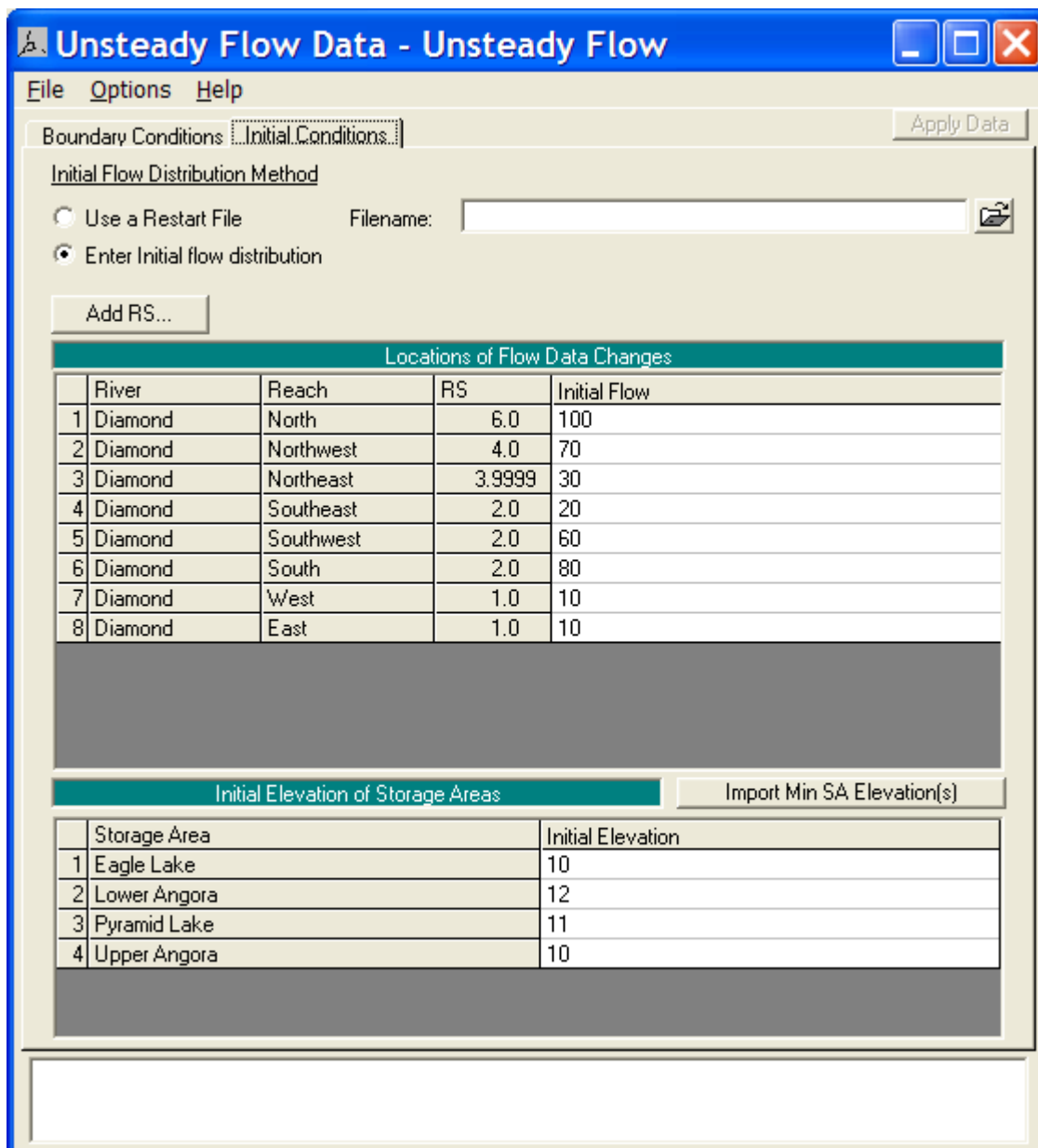
Figure 17-16: Unsteady Flow Data Initial Conditions
