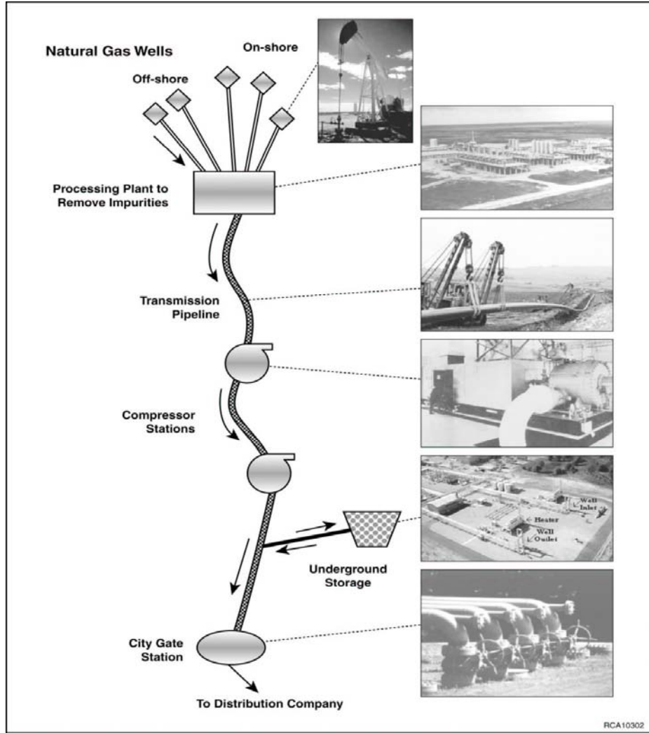
FIGURE 1.1-2 Schematic of Natural Gas Production, Processing, Transmission, and Storage (Source: Cirillo et al. 2003)
