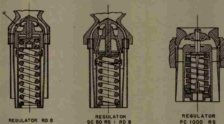
Figure 1 — Pressure Regulators for Solid Propellant Motors
