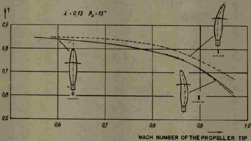
Figure 20 — Test Results of Swept Blades
