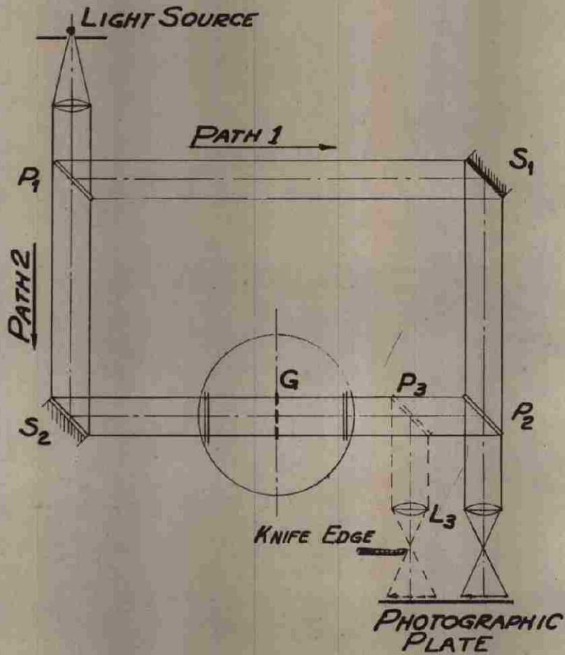
SCHEMATIC DIAGRAM OF COMBINED INTERFERENCE AND SCHLIEREN SYSTEM
