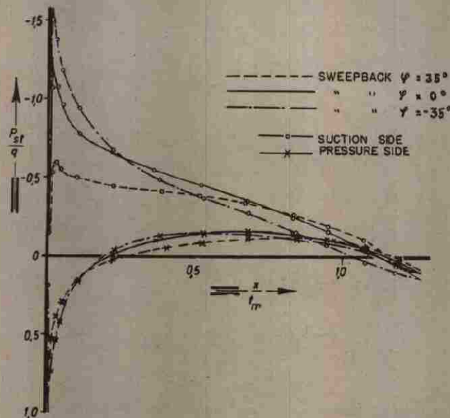
Figure 17 — Pressure Distribution near the Center of Sweep Forward and Sweepback Wings
