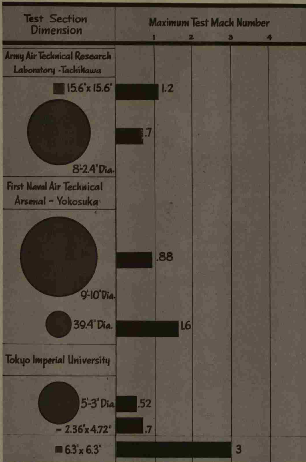
Figure 47 — Japanese Wind Tunnels
