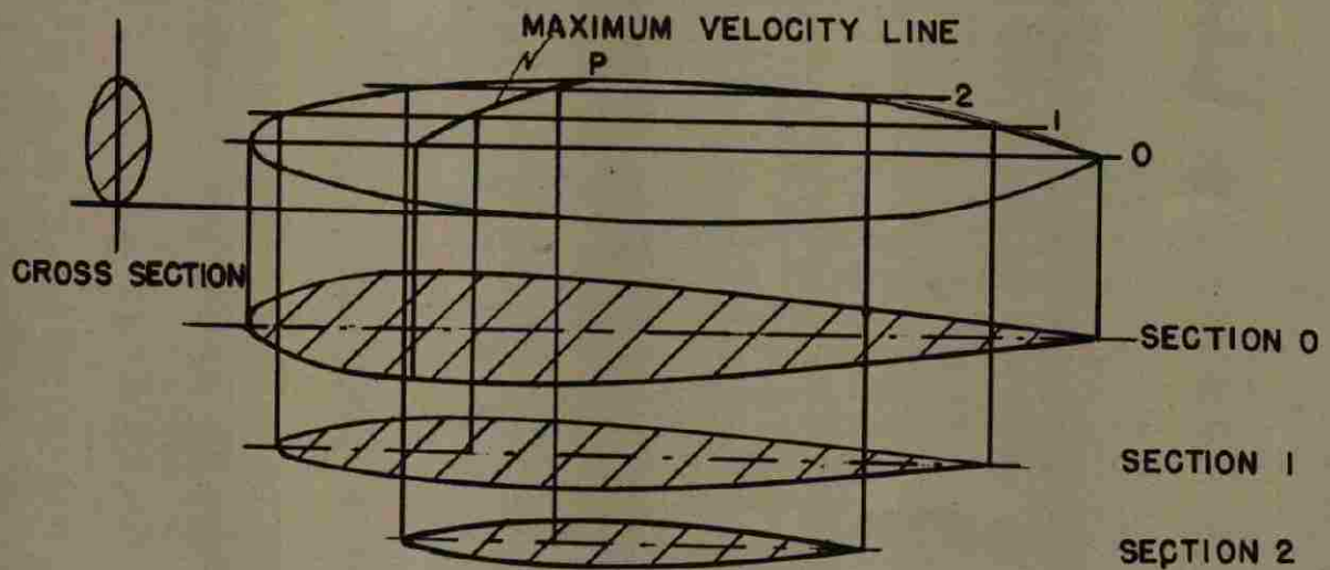
Figure 23 — Fuselage with High Critical Mach Number
