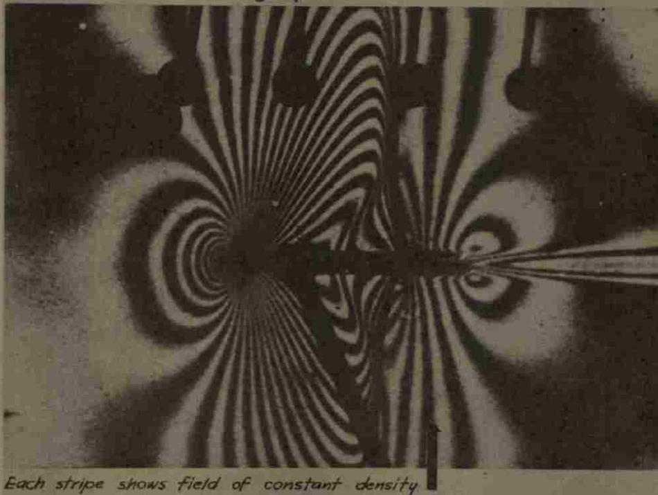
Figure 38 — High Speed Air Flow Photographs
