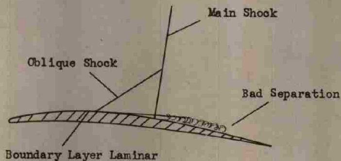
Figure 31 — Shock Formation at Small Reynolds Number
