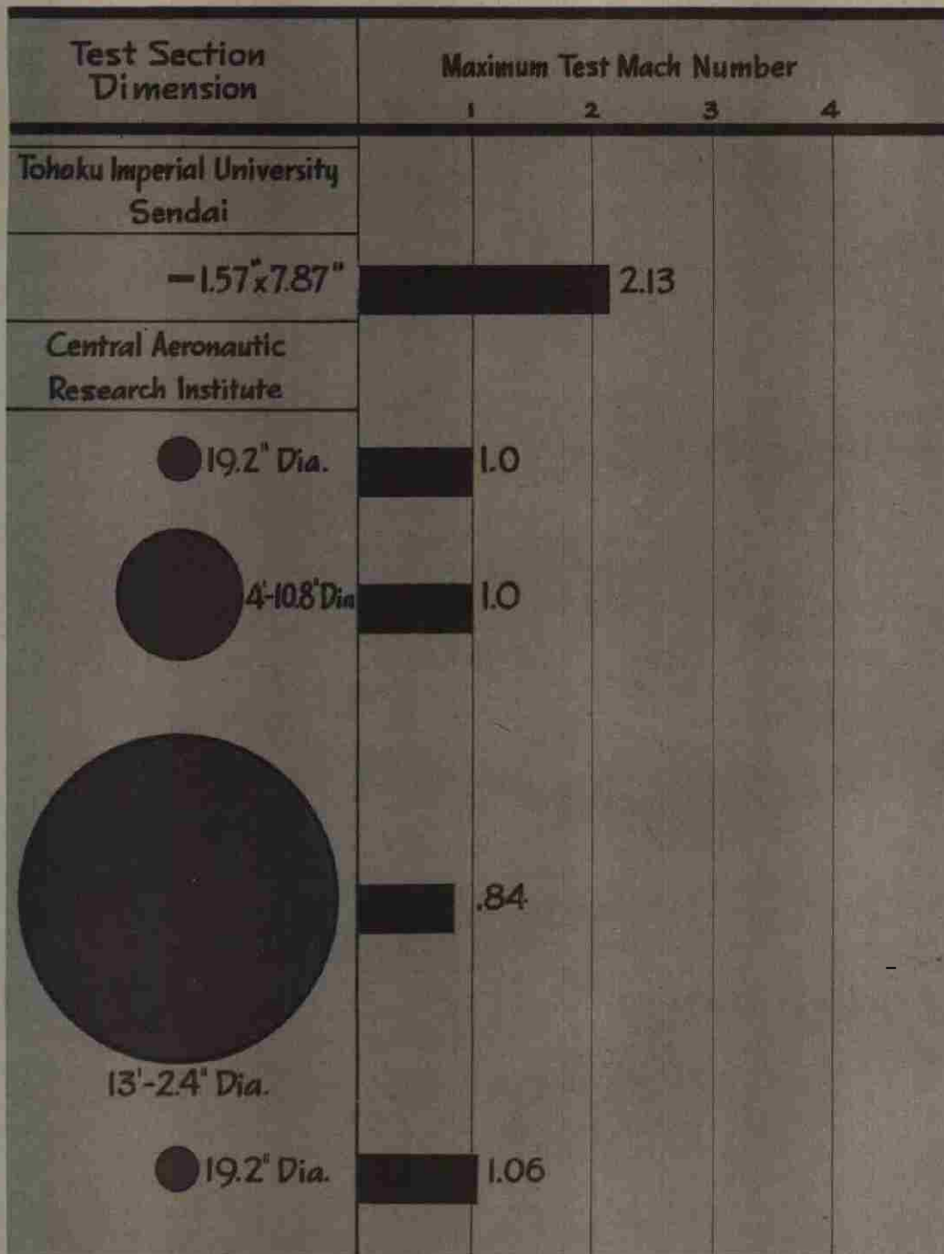
Figure 48 — Japanese Wind Tunnels
