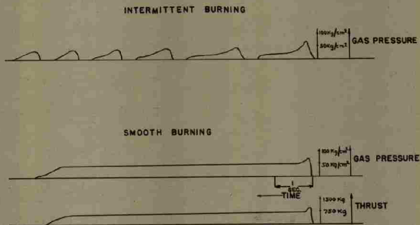
Figure 2 — Effect of Pressure Regulators
