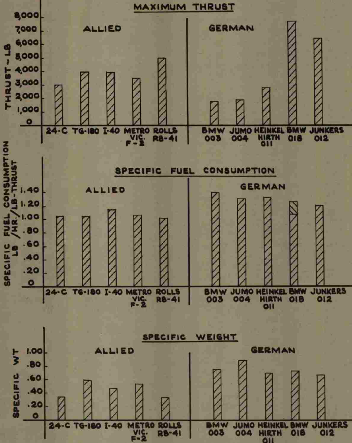
Figure 34 — Characteristics of German and Allied Turbojets
