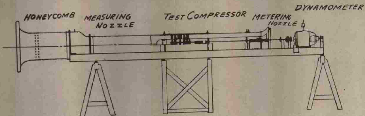
Figure 36 — Compressor Test Stand
