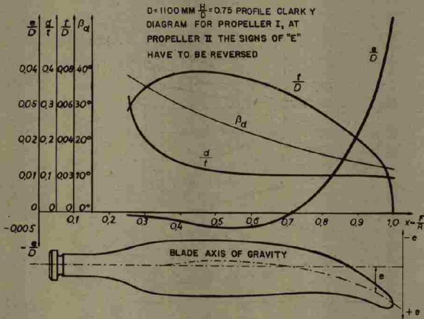
Figure 19 — Test Blade Form
