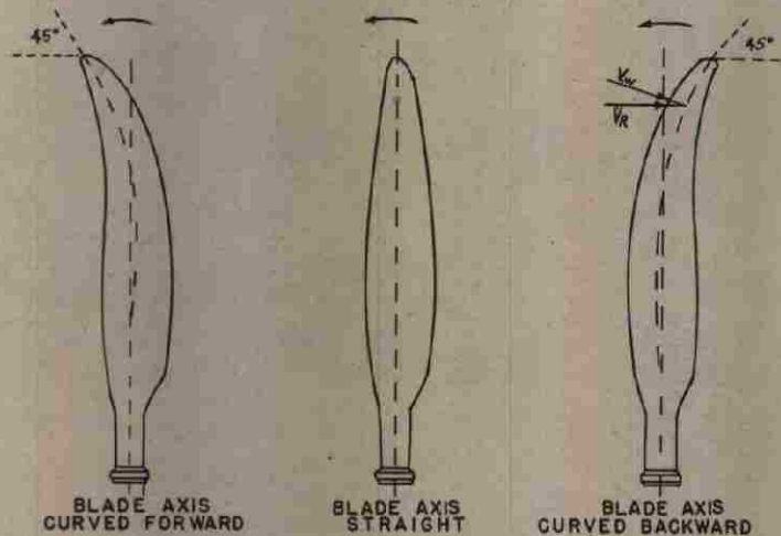
Figure 18 -- Sweep Forward and Sweepback Propeller Blades
