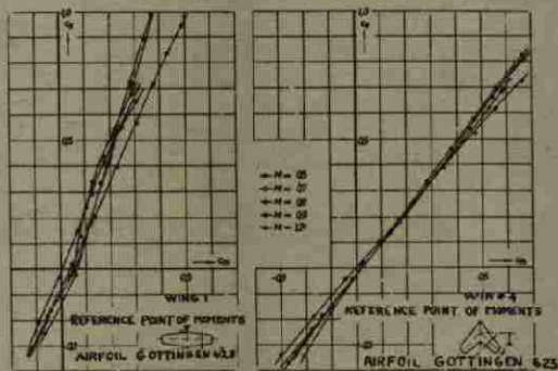
Figure 12 — Moment Coefficients C_m as Functions of Lift Coefficient for Wings No. 1 and No. 4
