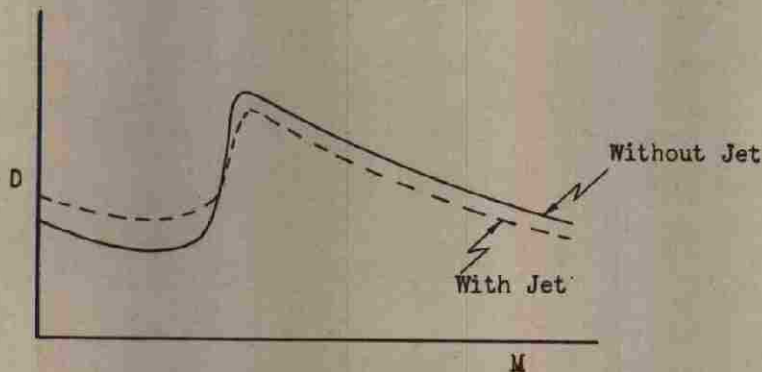
Figure 28 — Effect of Rocket Jet on the Drag of a Missile
