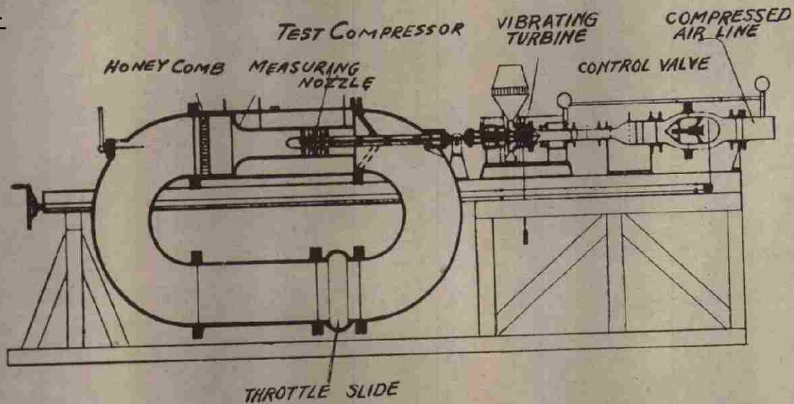
Figure 37 — Compressor Test Stand
