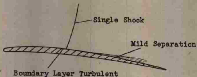
Figure 32 — Shock Formation at Large Reynolds Number
