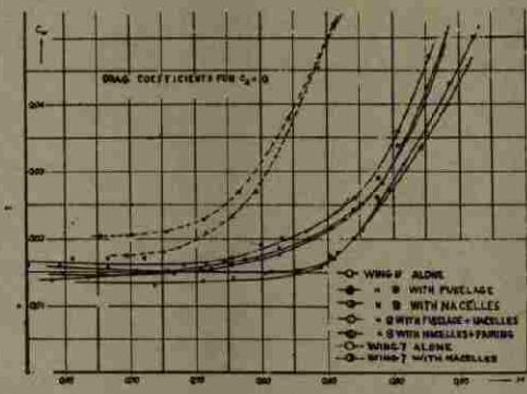
Figure 15 — Drag Coefficient C_w with and without Fuselage and Nacelle as Function of Mach Number at Lift Coefficient C_L = 0
