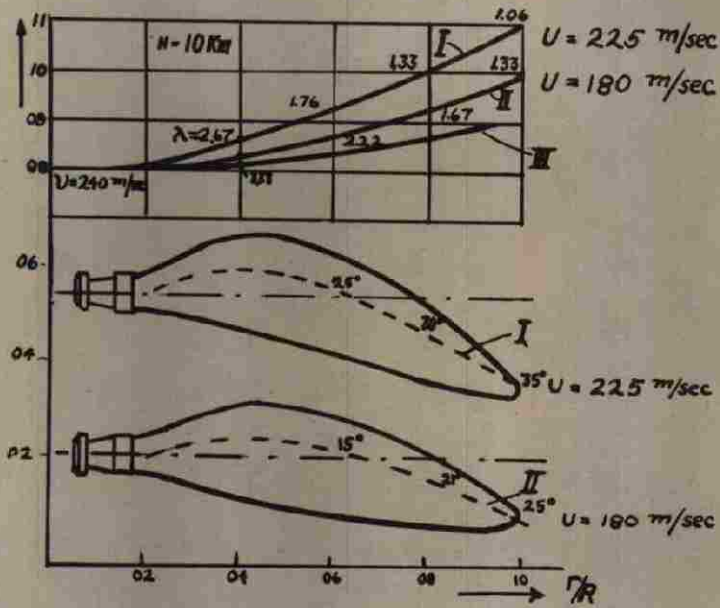
Figure 21 — Sweepback Blades for Flight Mach Number 0.8
