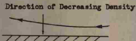
Figure 29 — Bending of the Light Ray Due to Transverse Density Gradient (Flow Velocity Perpendicular to Paper)
