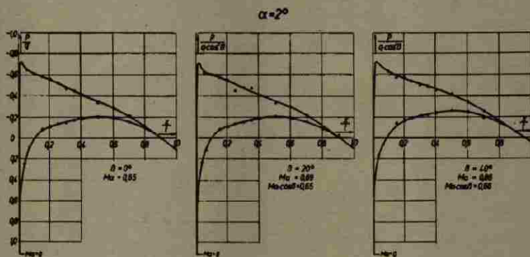
Figure 8 — M \cos \beta = 0.65
