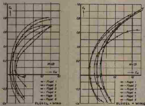
Figure 10 — Polars for Wings Nos. 1 to 6 for Mach Numbers 0.8 and 1.21
