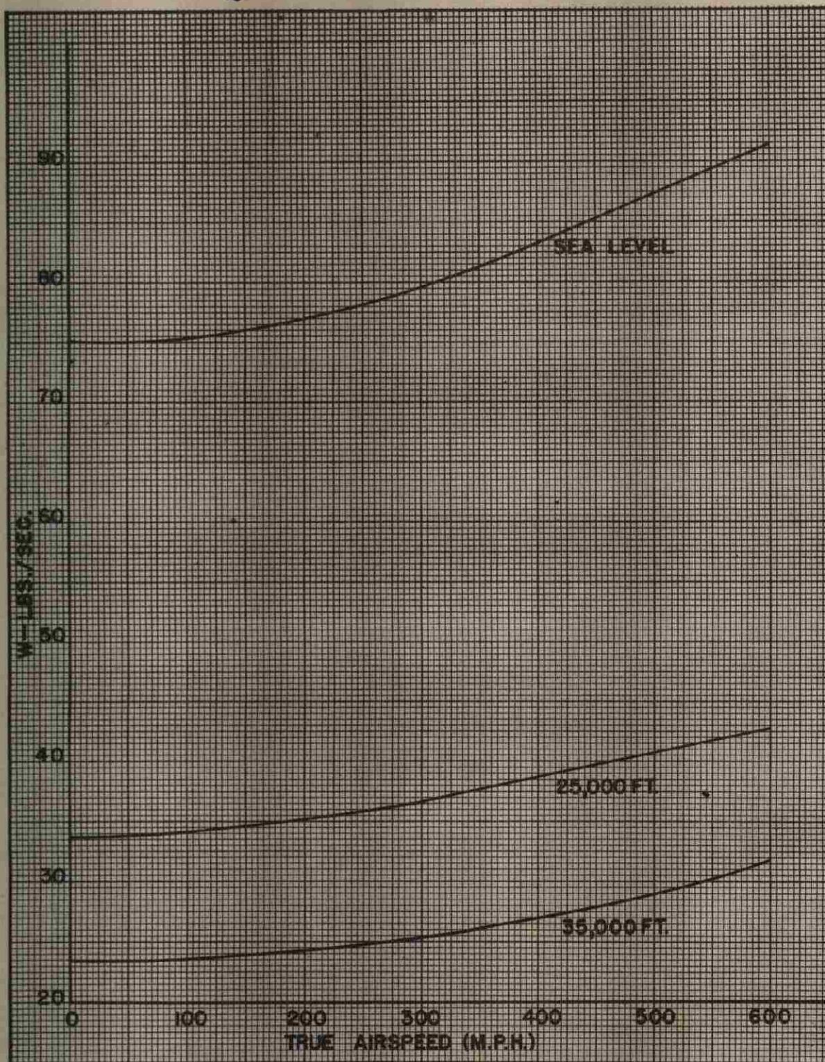
Figure 12 — Type I-40 Turbojet (11,500 RPM)
