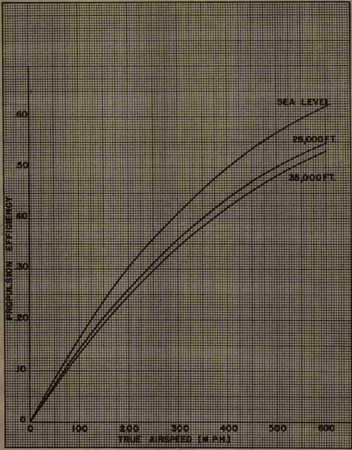
Figure 13 — Type I-40 Turbojet (11,500 RPM)
