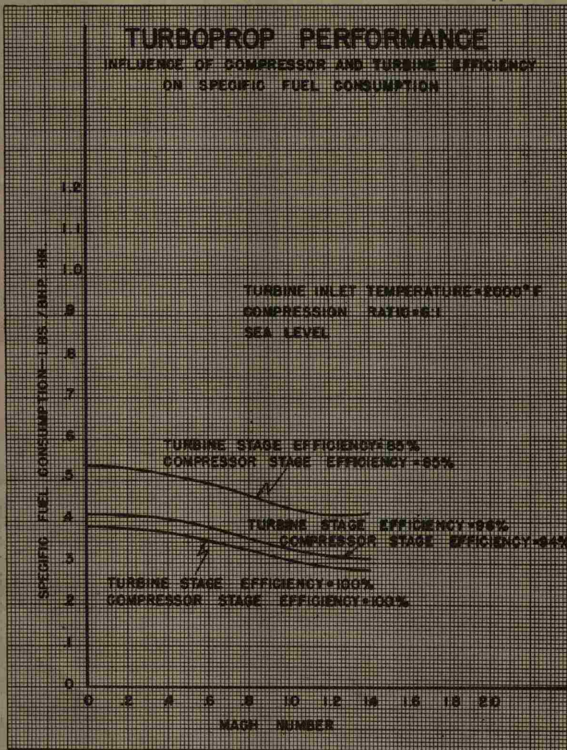
Figure 5 — Turboprop Performance (Influence of Compressor and Turbine Efficiency on Specific Fuel Consumption)
