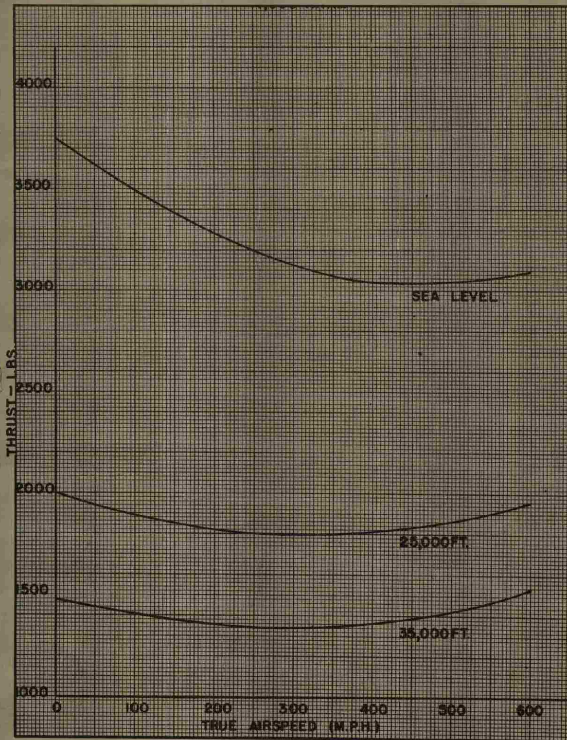
Figure 11 — Type I-40 Turbojet (11,500 RPM)
