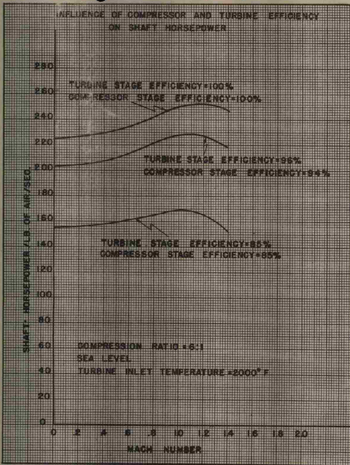
Figure 6 — Turboprop Performance (Influence of Compressor and Turbine Efficiency on Shaft Horsepower)
