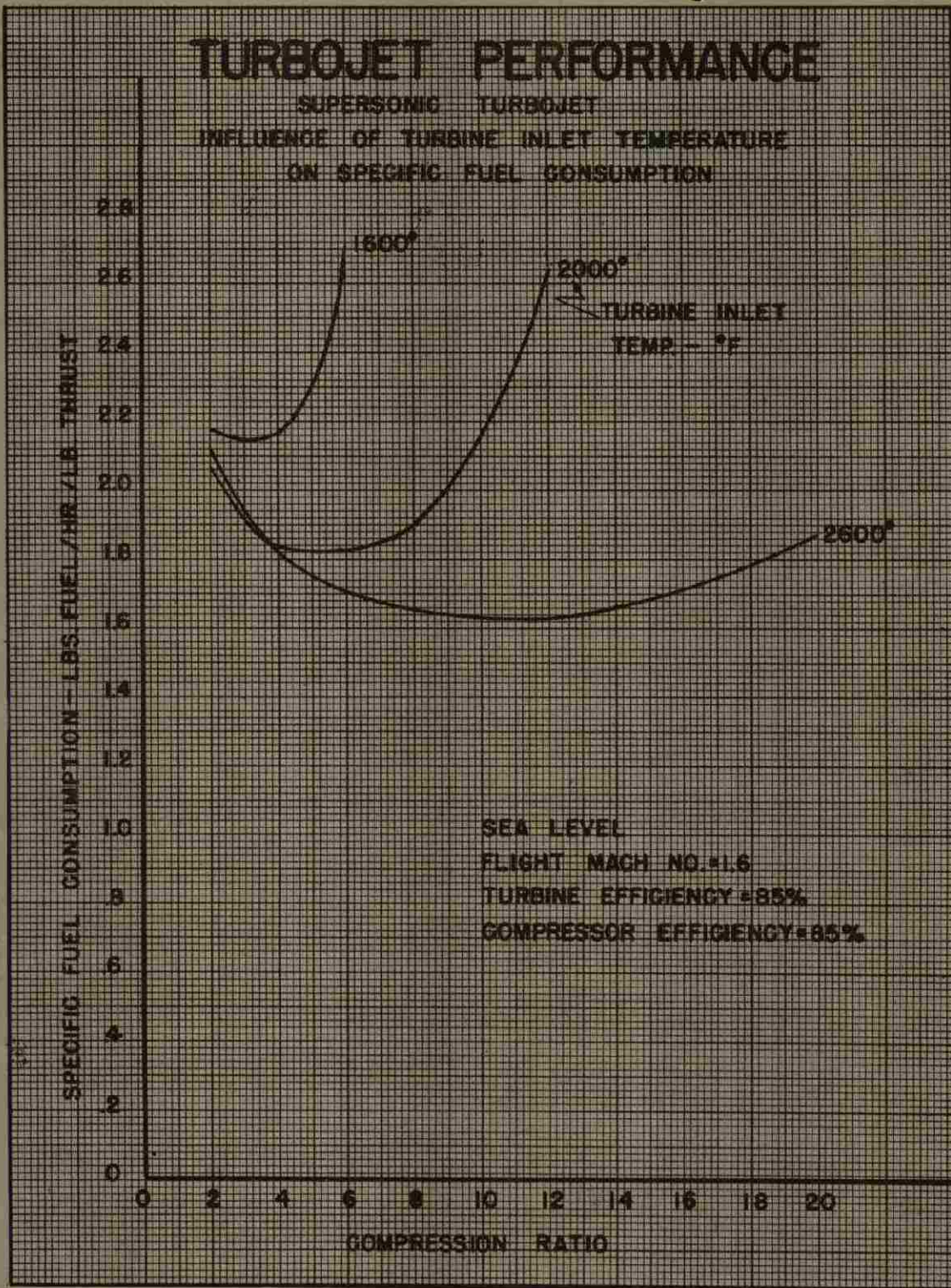
Figure 15 — Turbojet Performance (Supersonic Turbojet Influence of Turbine-Inlet Temperature on Specific Fuel Consumption)
