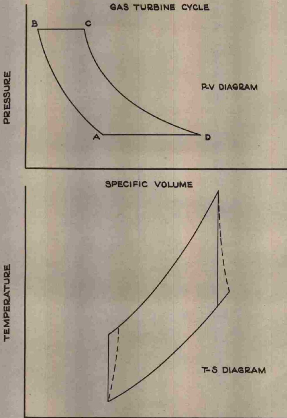
Figure 2 — (S) Entropy
