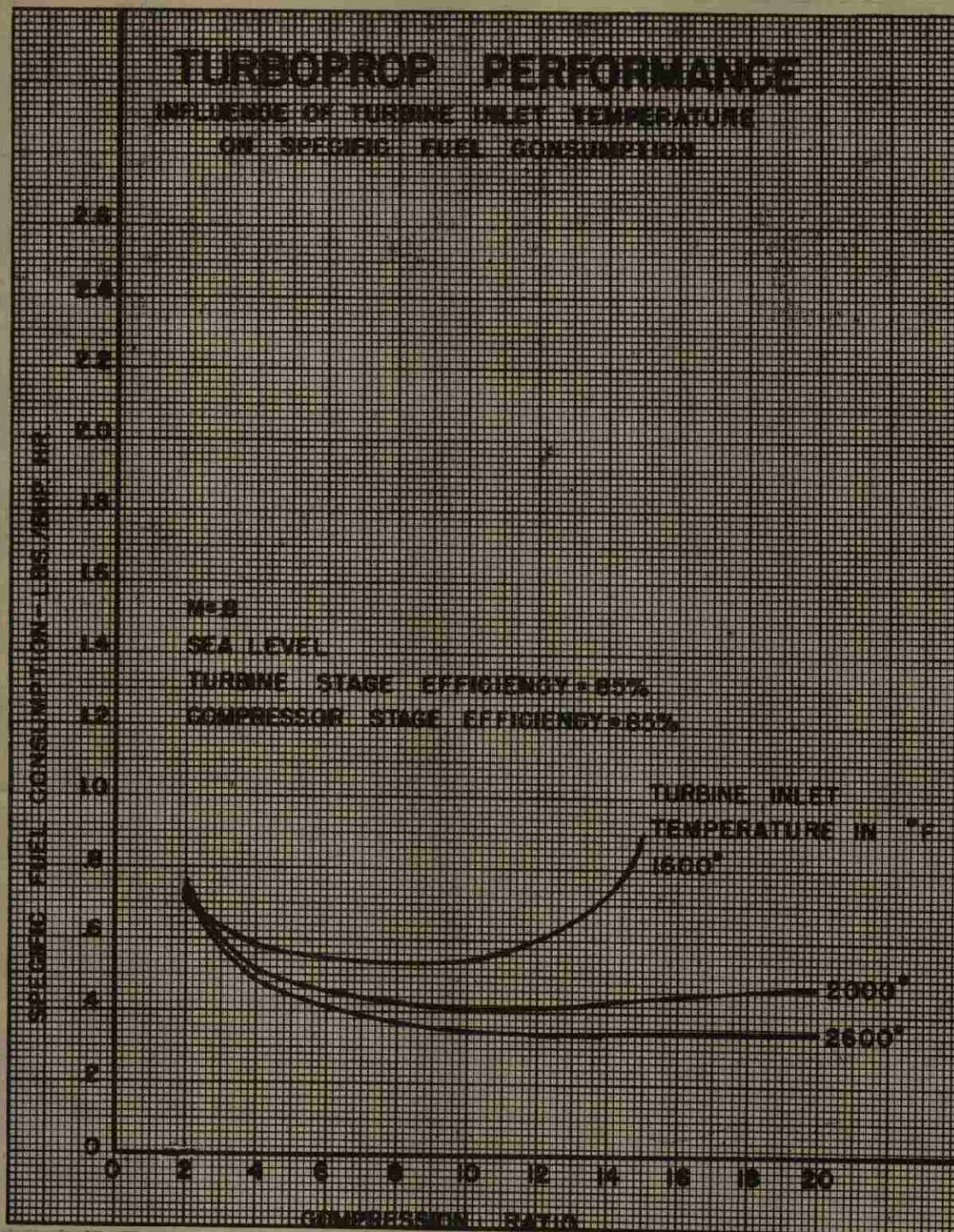
Figure 3—Torboprop Performance (Influence of Turbine-Inlet Temperature on Specific Fuel Consumption)
