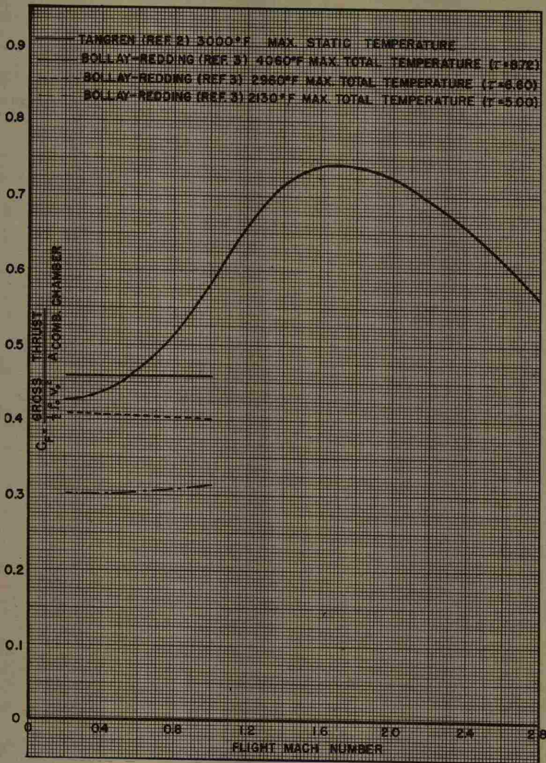
Figure 5 — Estimated Thrust of Ramjet at Sea-Level
