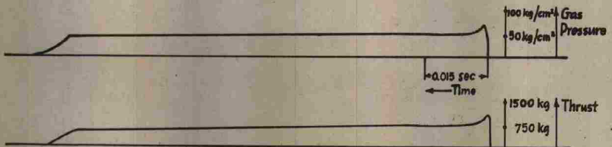
Figure 5 — Smooth Burning
