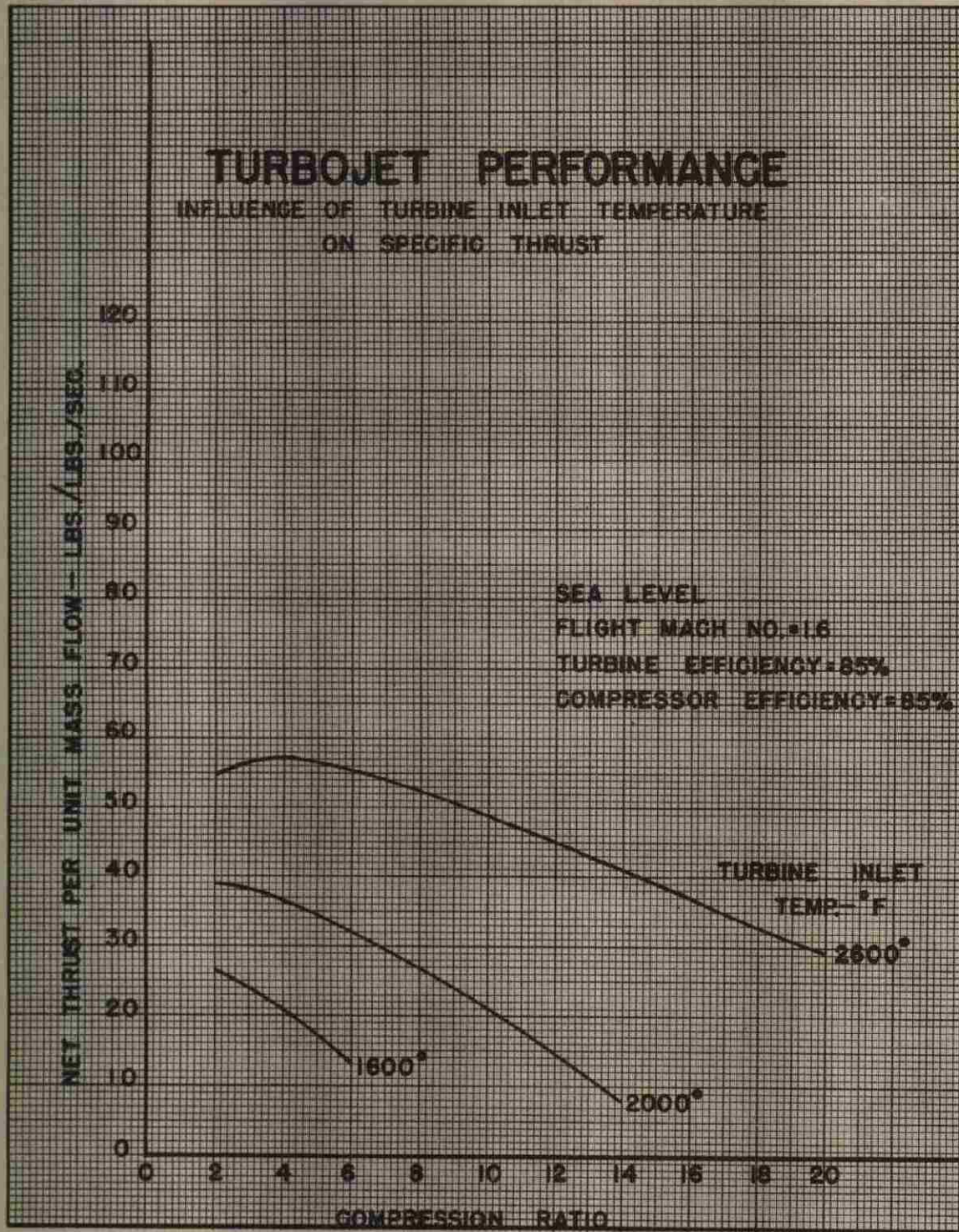
Figure 16 — Turbojet Performance (Influence of Turbine-Inlet Temperature on Specific Thrust)
