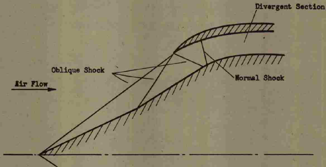
Figure 3 — Oswatitsch Diffuser
