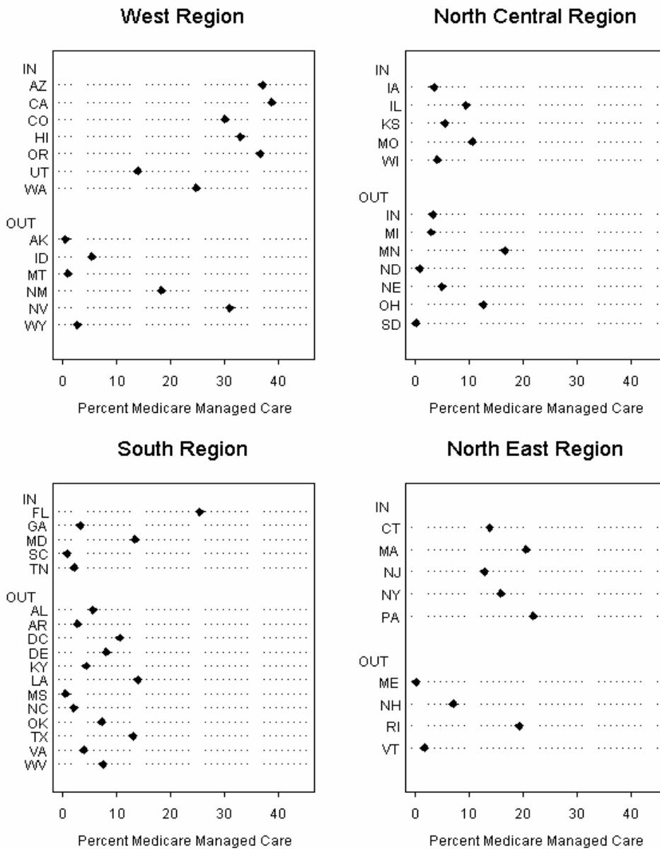
Figure 3 Percent Medicare Managed Care
