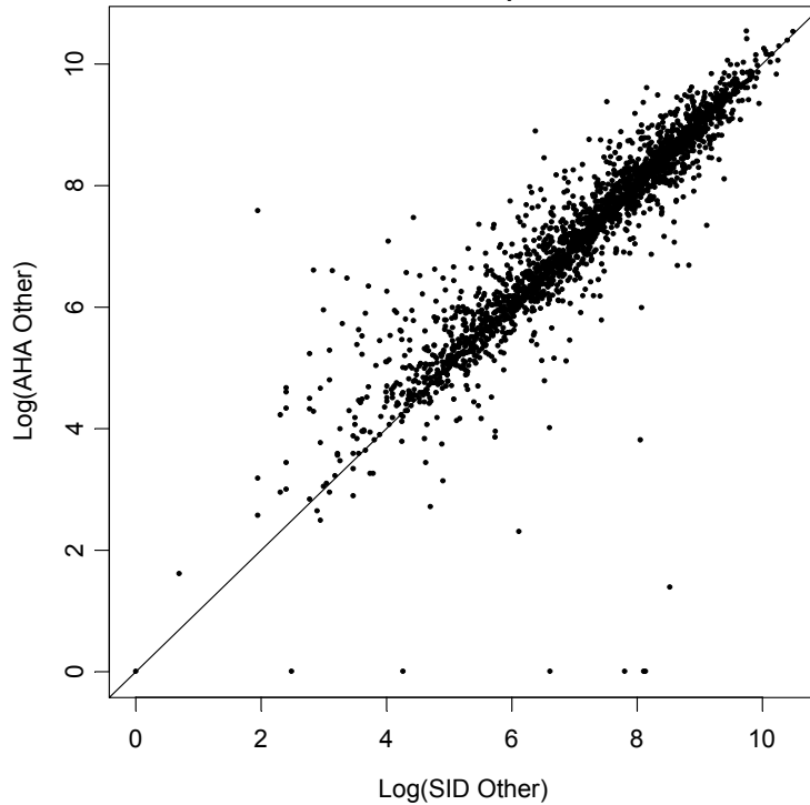
Log(SID Other Nonbirths) vs. Log(AHA Other Nonbirths) for Matched Hospitals, 1997
