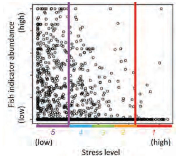
Fig. 1. Scatter plot of a fish indicator versus one landscape stress, showing upper (purple) and lower (red) condition thresholds and the scoring system (colored bars and numbers at bottom).
