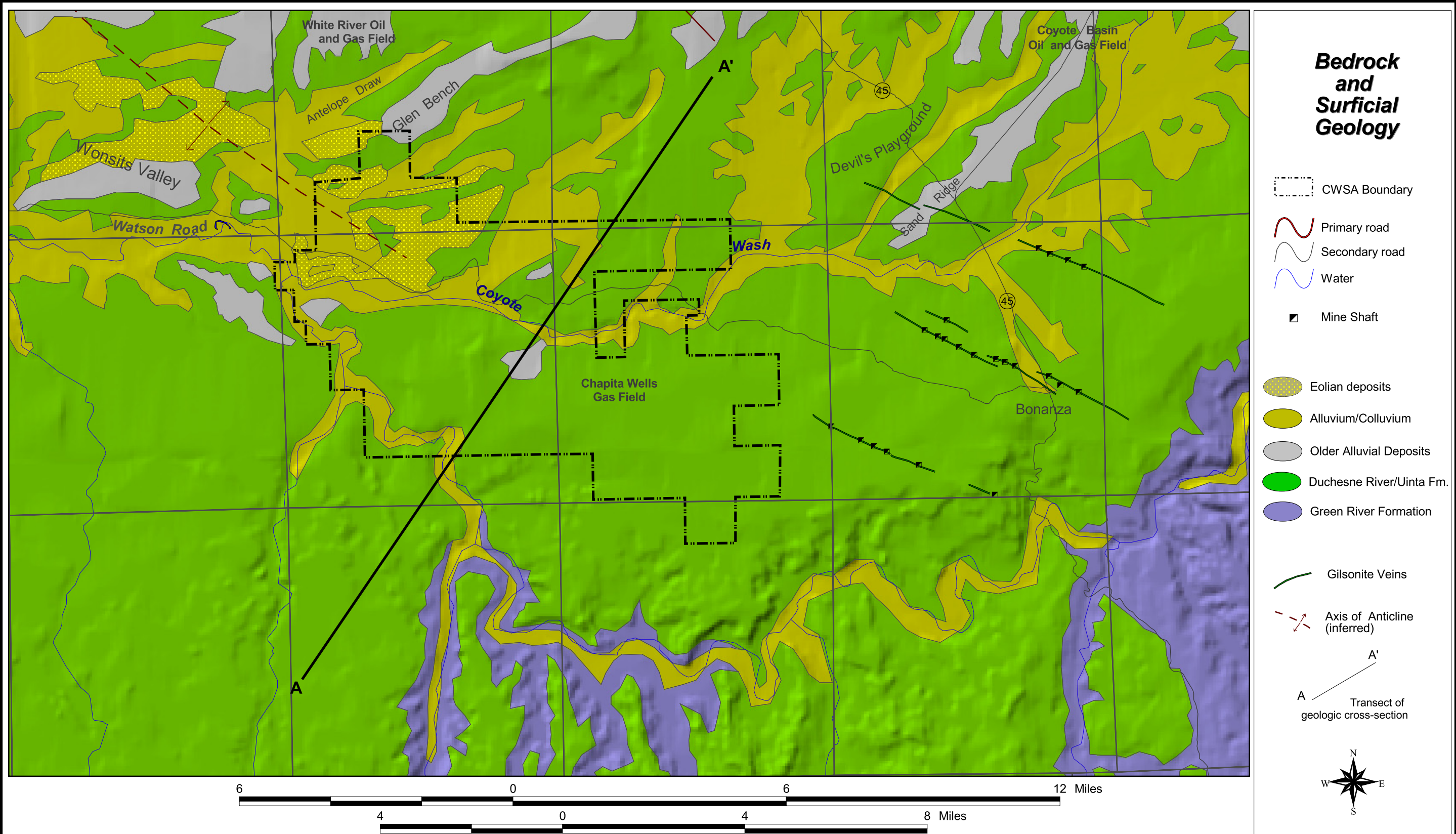
Figure 3.1-2. Geology within and near the CWSA (from Hintze, 1980).
