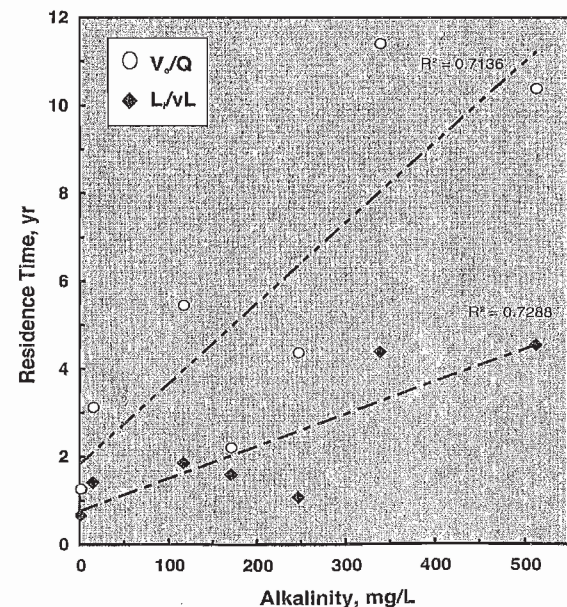
Figure 8. There is a positive correlation between discharge alkalinity and residence time calculated by either the volume-discharge ( V_p/Q ) or linear velocity ( L/v_L ) methods; however, the one to five year range of the latter best fits available field data for mine pool residence time.
