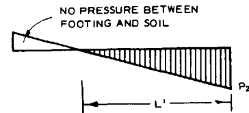
DISTRIBUTION OF BEARING PRESSURES BENEATH STRIP FOOTINGS
