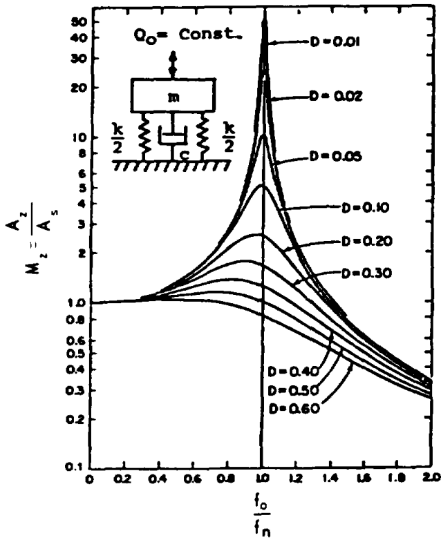
(a) CONST. FORCE AMPLITUDE EXCITATION Q = Q_o \sin \omega t
