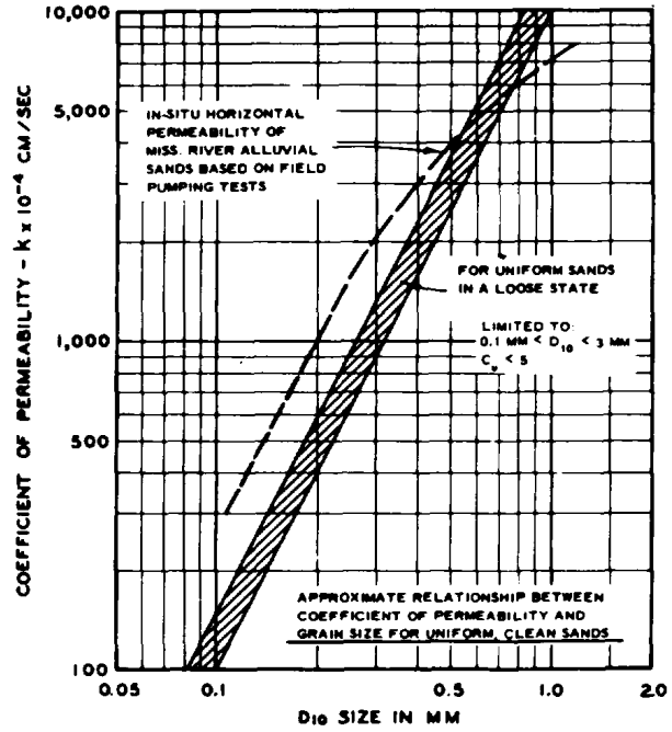
COMPUTATION OF PERMEABILITY FROM GRAIN SIZE
